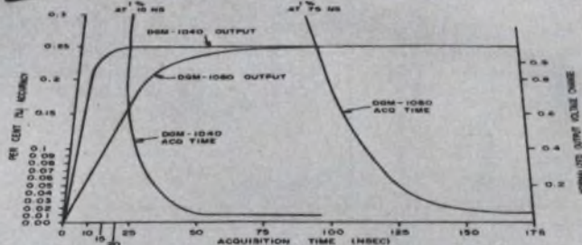
FIG. 3 ACQUISITION TIME VS. SETTLING ACCURACY
