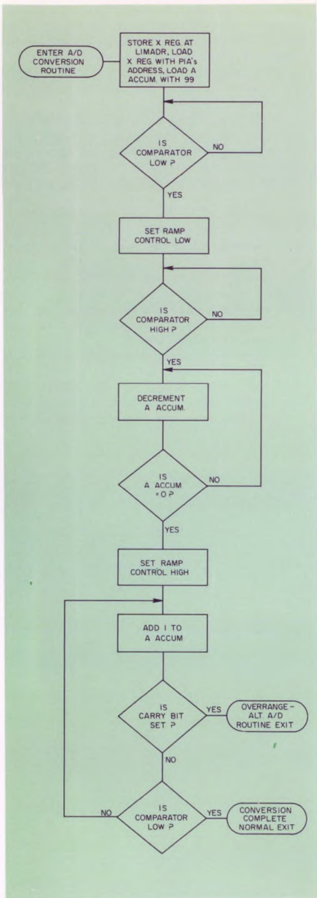
3. Flow chart shows the section of the program that controls the converter chips and performs the analog-to-digital conversion routine.
