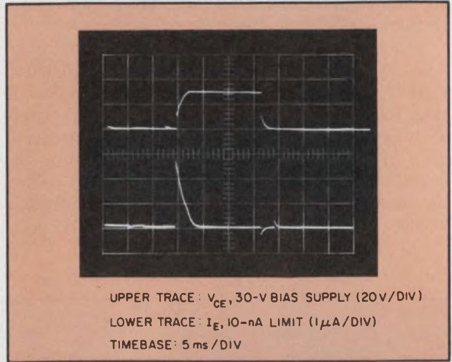
4. The effects of reduced base capacitance: As the base voltage stabilizes, the collector voltage rises to the full bias level, and the emitter current drops to the I_{CE0} level.
