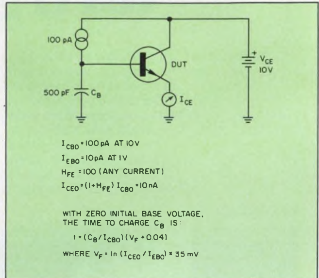
1. The effect of stray capacitance on I_{CEO} test time: With the values shown, it takes 1.4 s to charge the base capacitor—an unacceptably long time.
