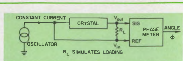
7. Crystal frequency is adjusted with a phase meter by use of resonance.
