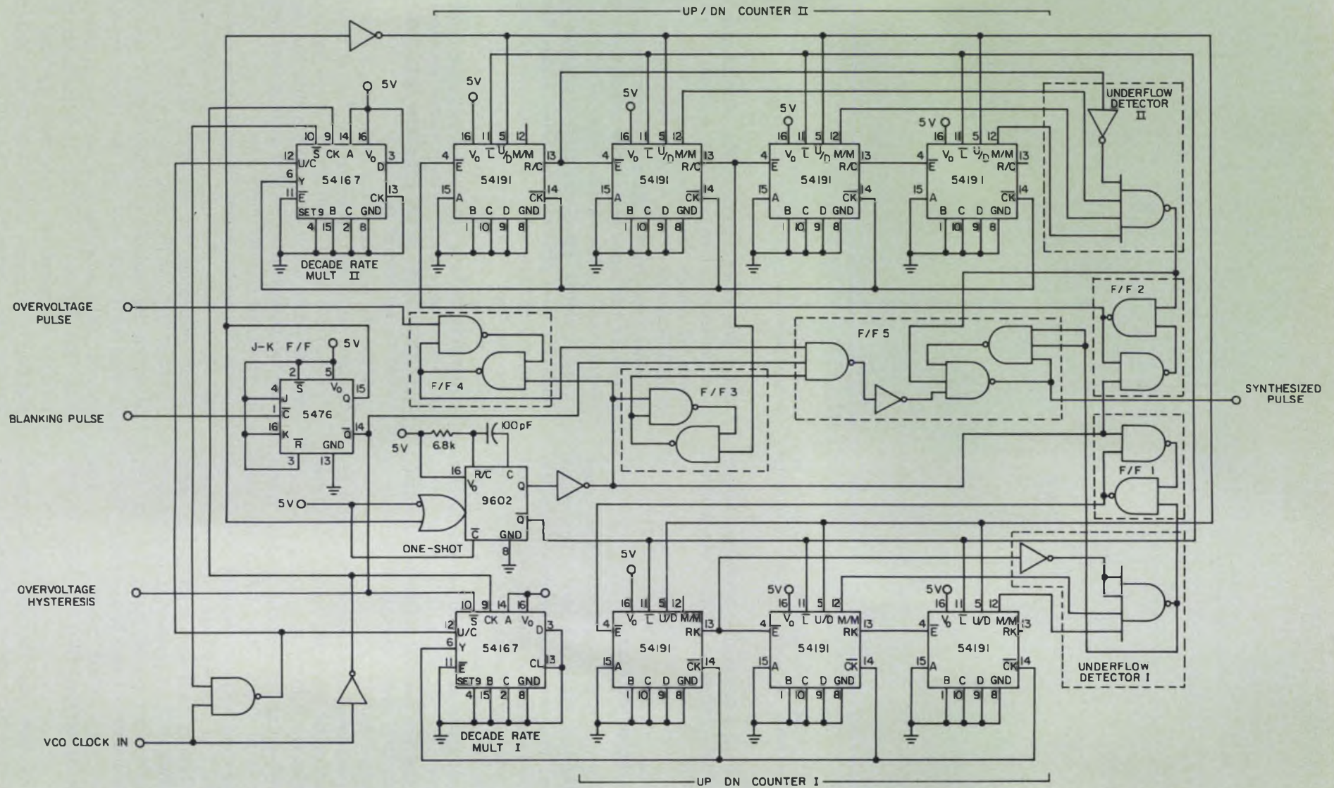
6. The digital section of the PWS converts the VCO signal to the final, synthesized pulse. To do this, the processor compares an incoming pulse's power with the
