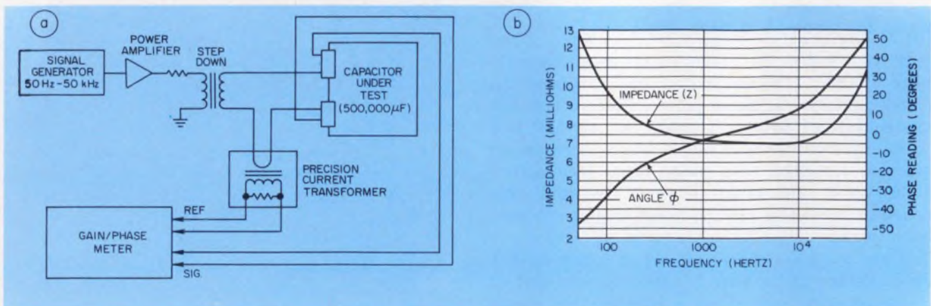
5. Gain/phase meters are ideal to measure very low impedances, such as that of a 0.5-F capacitor (a). The re-
