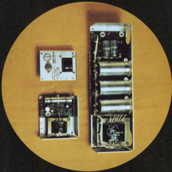
SINGLE OUTPUT
