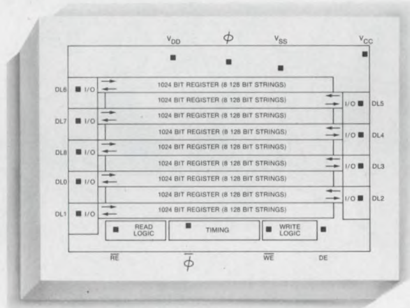
The first production CCD memory is Fairchild's CCD450, 1-Kilobyte serial storage device comprised of nine 1024-bit registers each organized in eight 128-bit strings. The CCD450 utilizes production proven Fairchild CCD buried-channel, ion-implanted barrier structure in the registers and Fairchild's Isoplanar N-channel MOS structure in on-chip timing, charge-detection and interface circuitry.
