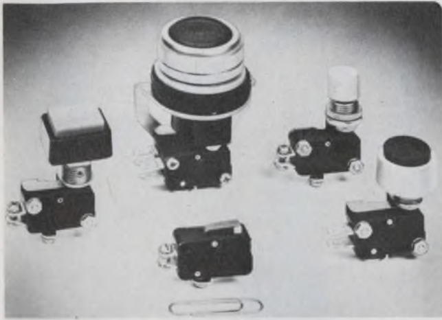
Many different superstructures attached to Cutler-Hammer's basic SS12 snap-action switch provide a flexible approach to pushbutton-switch design.
