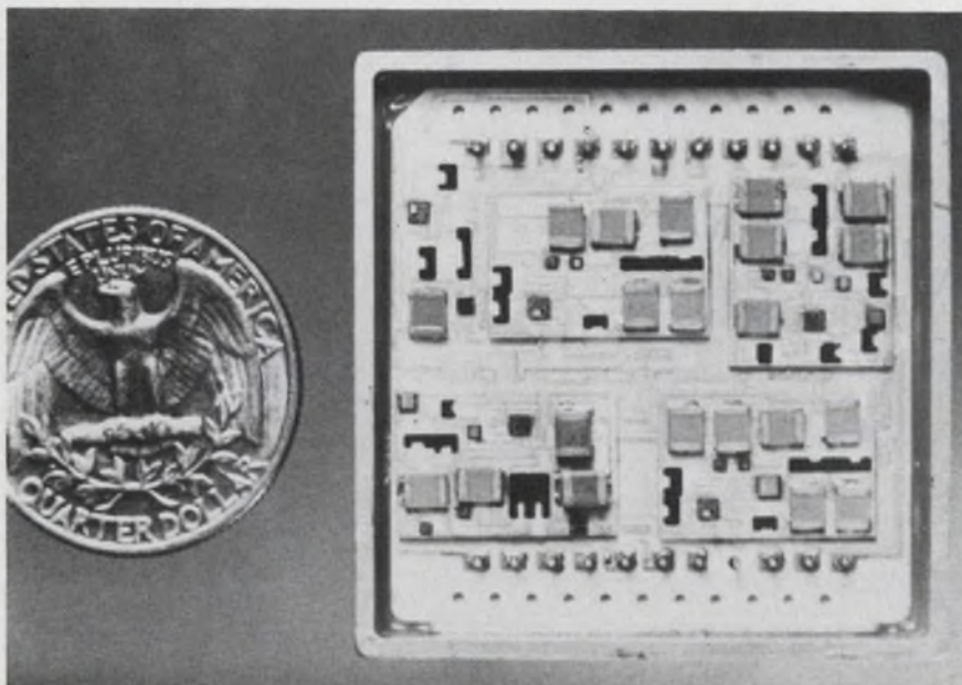
Hybrid houses have put multiple-pole active filters in small plug-in packages. Chip components are op amps and capacitors, assembled along with thick-film resistors on a ceramic substrate. This 1.6 x 1.6 x 0.25-in. package from General Instrument contains an eight-pole elliptic filter for operation in the 3-to-50-kHz region.
