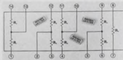
STANDARD PRECISION RPD1800 THIN-FILM ATTENUATORS/DIVIDERS FROM ANALOG DEVICES, INC.
