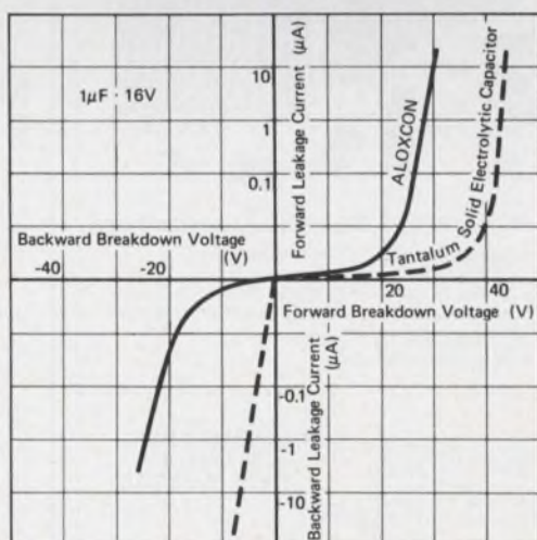
E-I Characteristics
