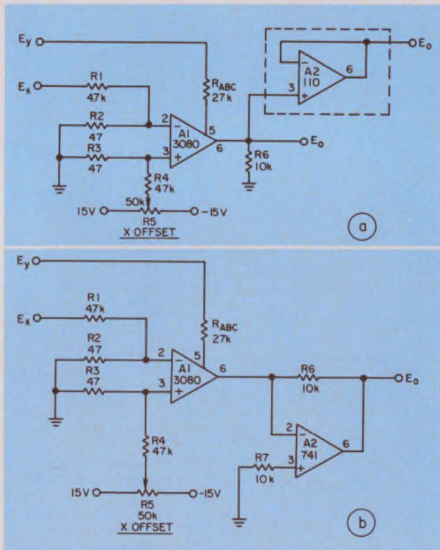
6. Let E_c control the differential current, and the operational transconductance amplifier provides variable gain. The first version (a) isolates the output ( Z_o \approx 10 k) with a voltage follower. Alternatively a current-to-voltage converter (b) can be used with the same results.
