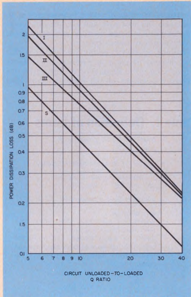
3. Circuit unloaded-to-loaded Q vs power dissipation loss in dB shows that the 90% point of Fig. 2 is equivalent to a loss close to 0.5 dB—unsatisfactory for rf circuits that provide gains of only 3 to 8 dB.
