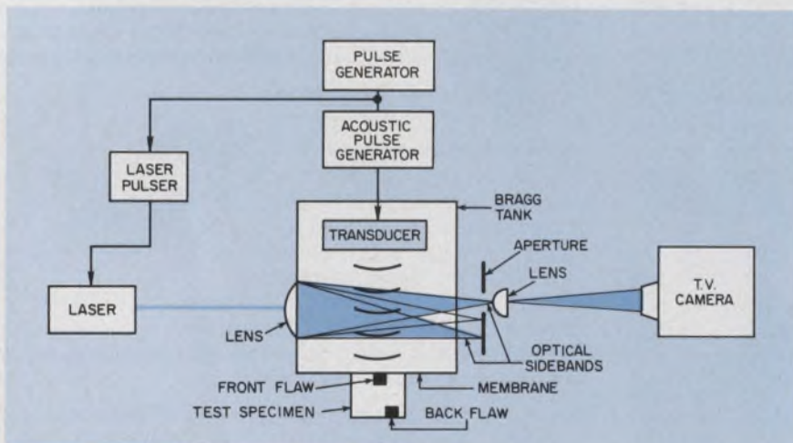
Images of flaws inside test specimens are produced in optical sidebands generated when sonic energy and a laser beam are mixed inside a Bragg tank. The laser is gated to detect flaws at different depths.
