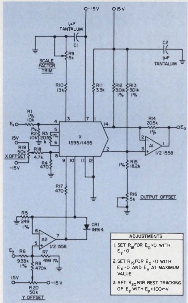
4. Two-quadrant operation of 1595/1495 IC increases the dynamic range to 80 dB. The connections shown disable one of the two-quadrant multipliers. Op amp A_2 provides a controlled current source, as in Fig. 2.
