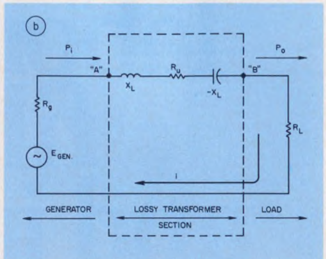
1. Network efficiency is reduced by the parallel-source resistance R_p of the current generator (a). The equivalent series circuit at resonance is shown in "b."
