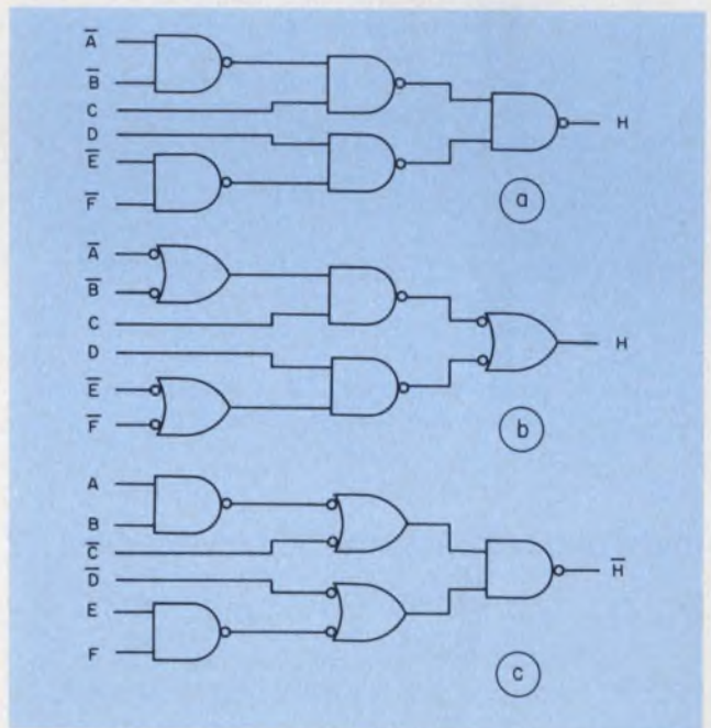
3. The proper choice of symbols can make it easier to see what's happening. Both schematics "a" and "b" have the same inputs and yield the same output. But the logic equation that relates output to input can be put down almost immediately with schematic "b." If, however, emphasis is to be put on the output AND function, a third schematic can be drawn (c).
