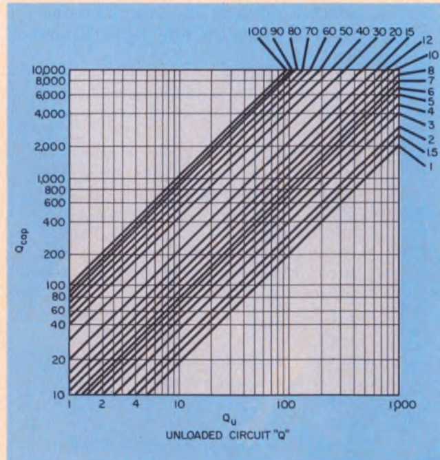
5. The required capacitor unloaded Q can be found quickly once the Q_{cap}/Q_{ind} ratio is established. Careful capacitor selection is needed to get high values.
