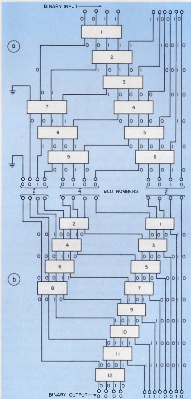
2. Binary-to-BCD (a) and BCD-to-binary (b) converters of any size can be assembled from building blocks of the logic modules shown in Tables 3 and 4. Building blocks made of specially programmed ROMs, such as the MC 4001, provide identical conversion functions with fewer packages and operate at higher speeds.
