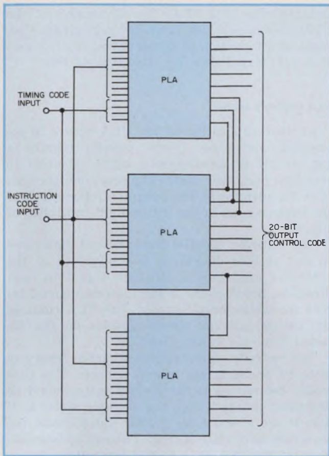
5. Three PLAs can replace a multiplexer data decoder that uses ROMs. The advantages of the PLA approach include higher speed and fewer components.
