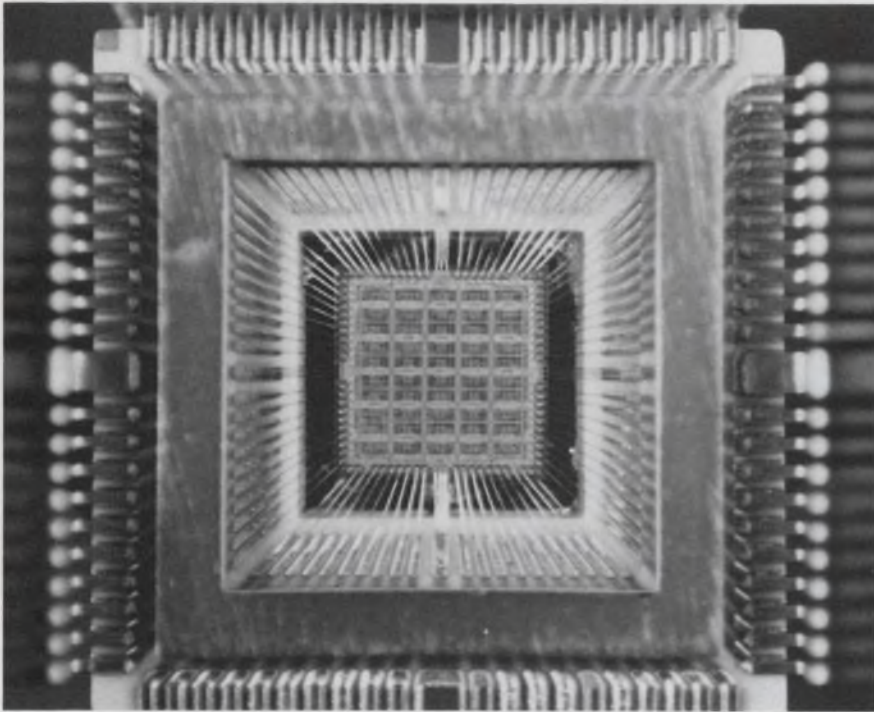
Mounted LSI array used in the central processing unit of the model 470 computer now under development by Amdahl Corp., Sunnyvale, Calif., contains gold in the wire bonds to the chip terminal, the chip carrier and the substrate terminals. The array uses ECL, contains 100 gates and measures 150 mils on a side.
