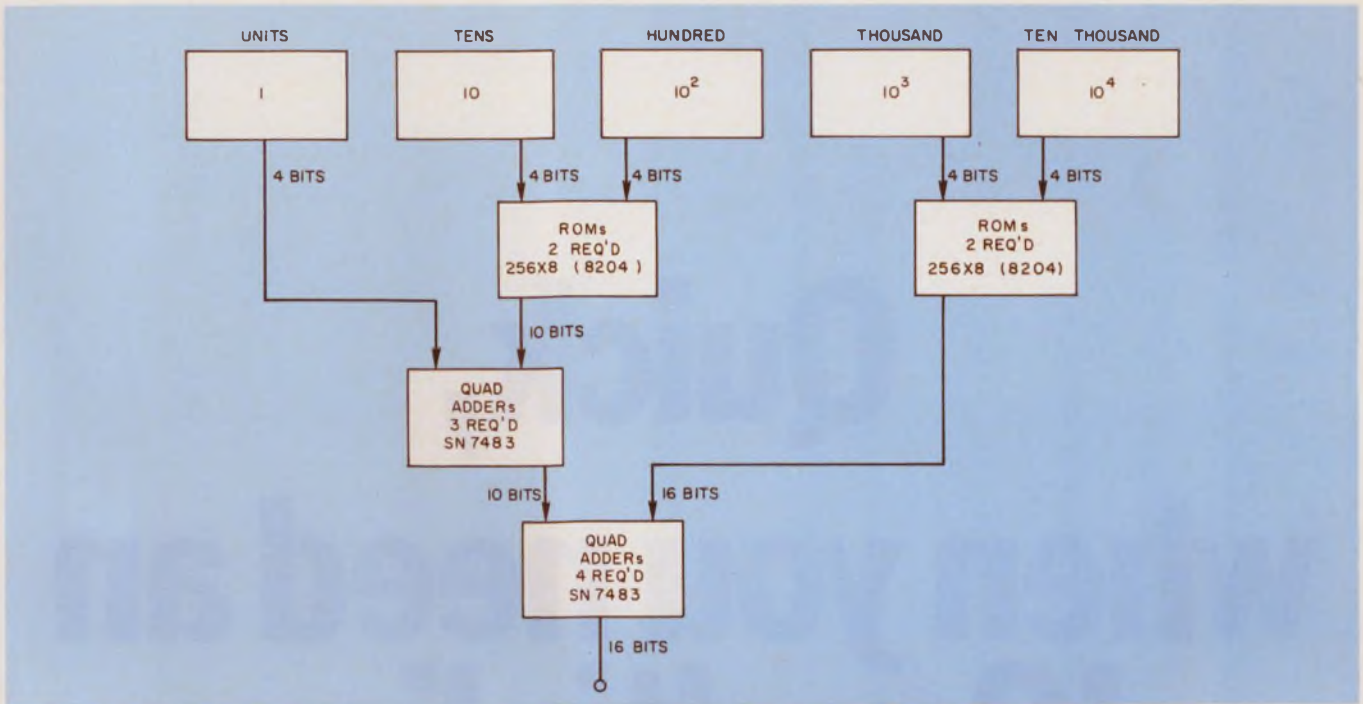
4. Reduced part count and increased speed result when the outputs of specially programmed ROMs are com-
