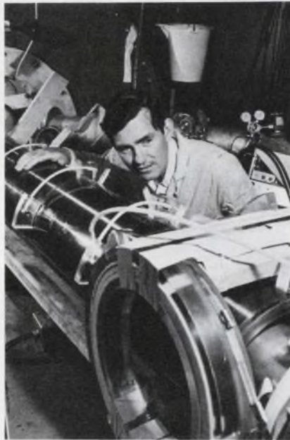
Hydrogen-fluoride laser developed by Sandia will be used to explore the possibility of producing electrical power through laser fusion.
