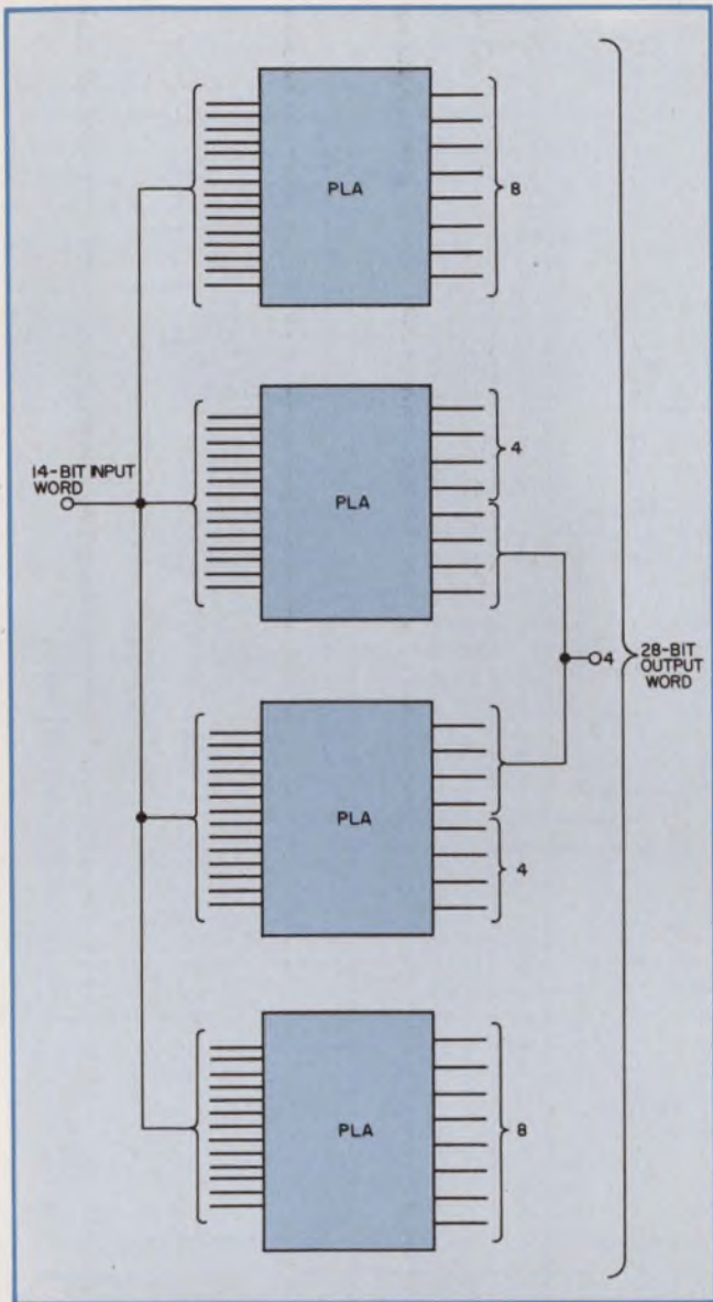
2. Common control codes can be grouped together to simplify mask-programming of partial product terms. Negative-TRUE logic permits wired-OR connections.
