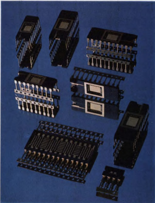
To protect light-sensitive integrated circuits and to enhance the contrast of LED displays, these black alumina ceramic packages, by American Lava, have a dark, opaque filling. The packages have multilayer interconnections. They also provide a good heat sink.
