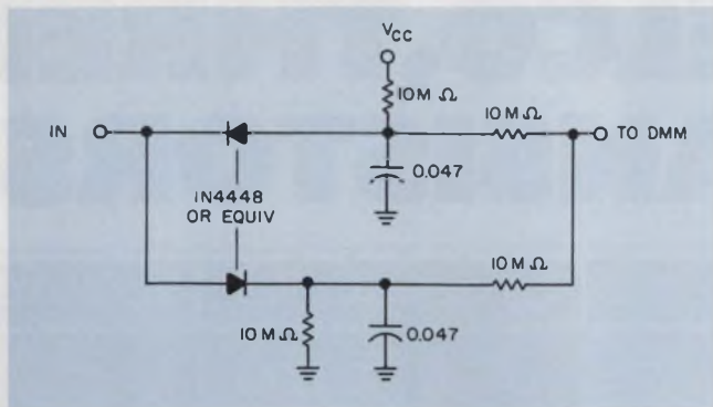
6. Need a logic checker? With this pulse stretcher, a DMM can indicate a HIGH, LOW or pulse train.
