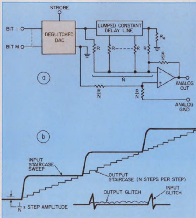
3. The addition of a multitapped delay line (a) to the deglitched DAC lets the boxcar integrator average glitches over the conversion cycle (b) to reduce the quantization error in a staircase sweep.
