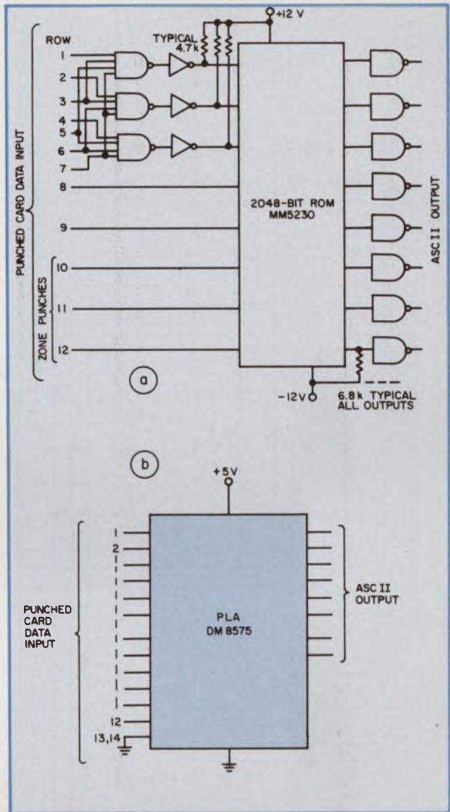
3. A Hollerith-to-ASCII conversion requires external components when using a ROM (a). But with a PLA (b), such conversions can be performed directly.
