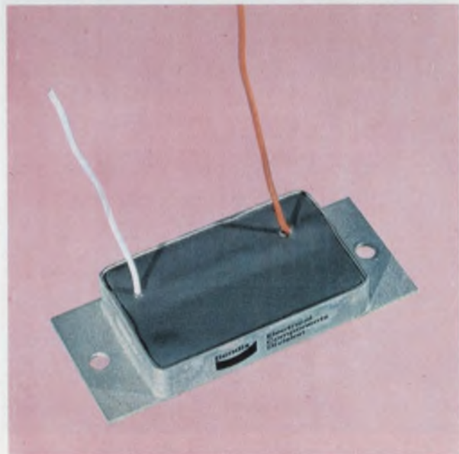
Good heat-transfer and environmental protection is provided by this silicone potting for a Bendix 3000-V silicone rectifier used in a 500-F ambient. The silicone is filled with alumina to improve heat transfer.
