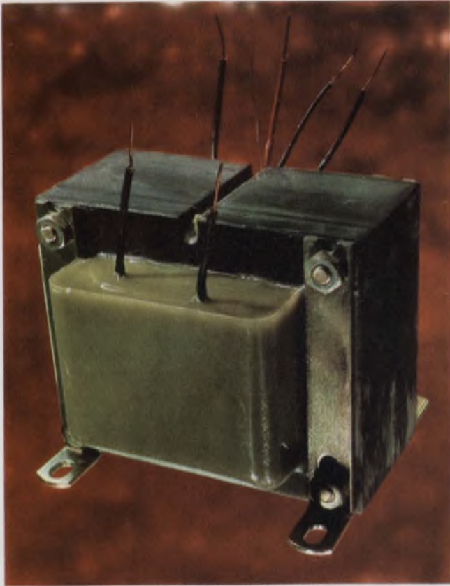
Control transformer is used in a high-temperature environment with intermittent current overloads. It's potted in a filled Scotchcast 28 semiflexible resin, which meets NEMA's Class F rating (155 C).
