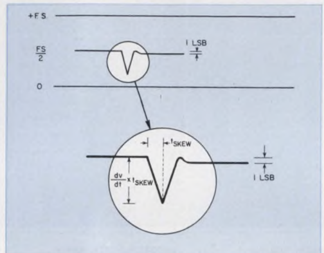
1. The major carry transition at the DAC half-scale shows the glitch caused by skewed data on the inputs and a high op-amp slew rate.
