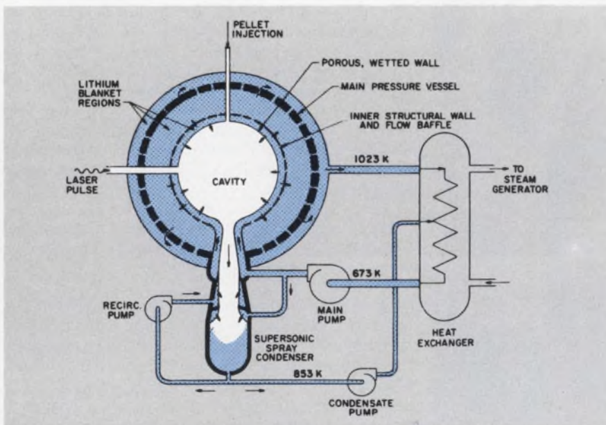
A proposed fusion power plant uses a lithium blanket to absorb the high energy neutrons. The lithium heats up, and transfers the energy to water which in turn produces steam to drive a generator.
