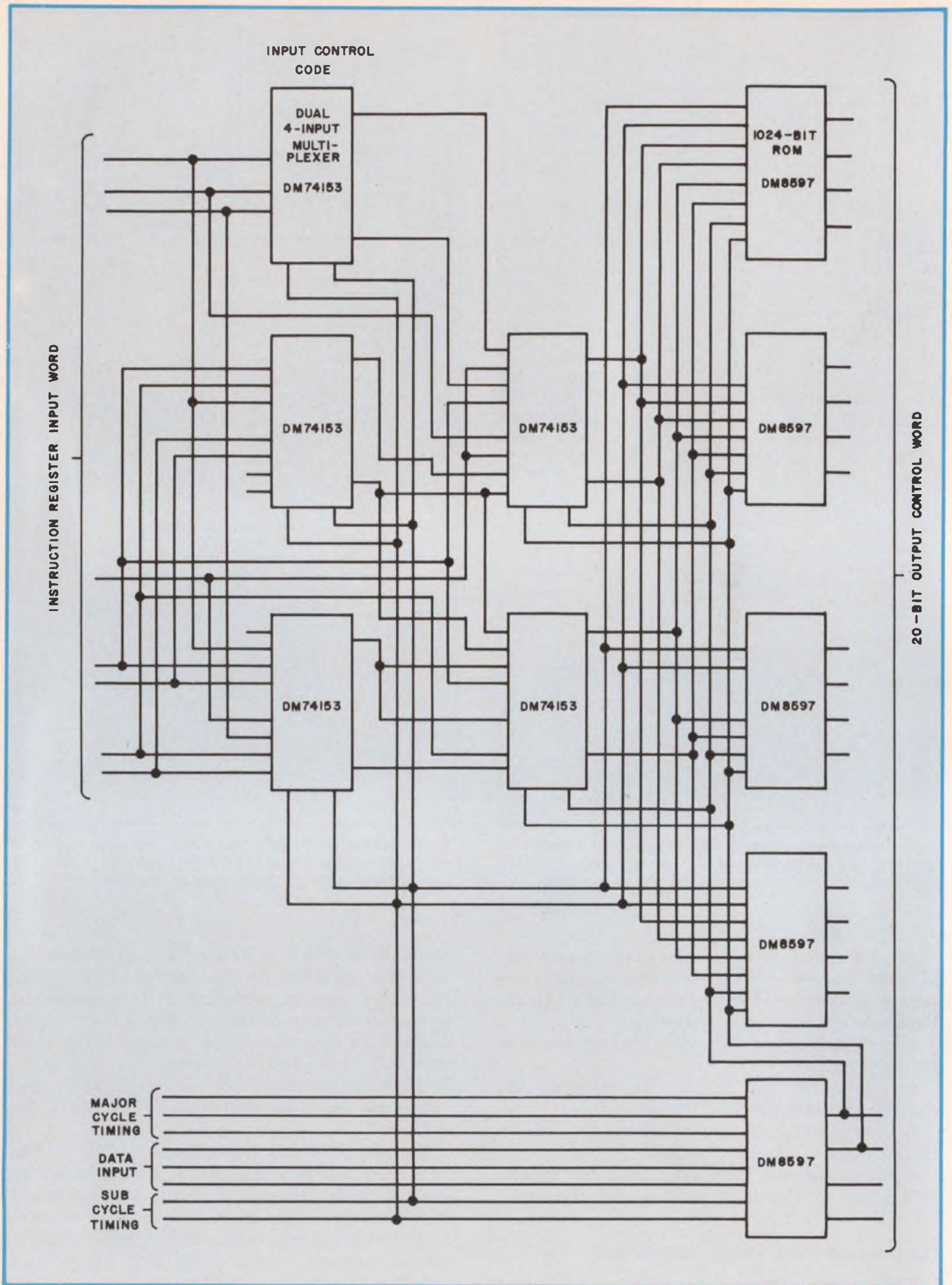
4. A multiplexer data decoder routes data to the appropriate ROM group. Two levels of multiplexing reduce
