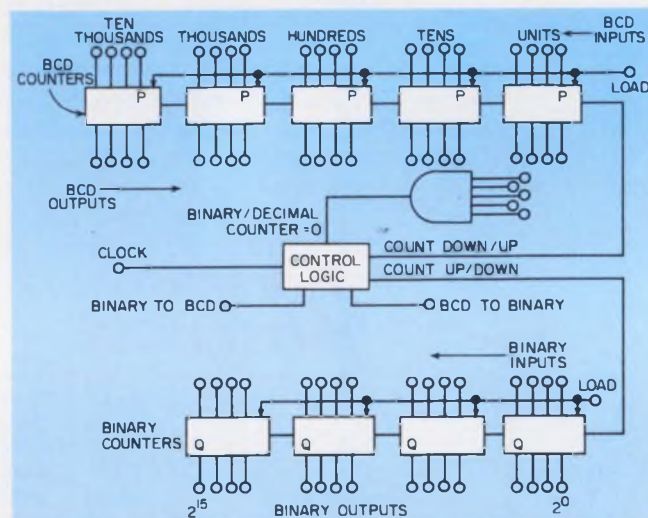
1. Serial counting is the easiest BCD/binary conversion method to understand. It can be done with few MSI packages, but it is slow.
