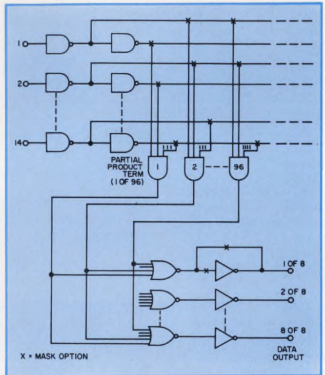
1. A PLA generates a sum of partial product terms that have the inputs as variables. The DM 8575/8576 PLA can accommodate up to 96 such terms.
