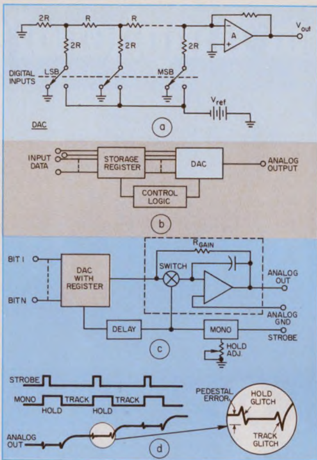
2. The basic DAC (a) can be improved by adding a storage register (b) and then a track-and-hold amplifier (c) to eliminate some of the major glitches that would otherwise appear in the output (d).
