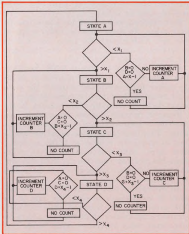
7. The state diagram for the traffic controller illustrates the functions performed. While in any state, the controller checks the others possible to obtain the timing interval of the present state.
