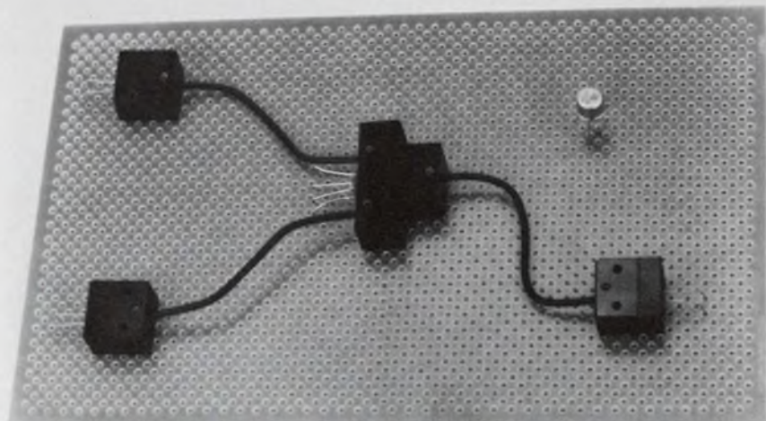
The electrical input from two emitter modules (left) is summed in the optical AND gate (center). Output is decoded by detector module (right).
