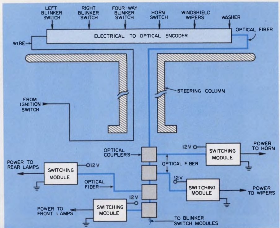
Fiber optics for control of automotive electrical equipment has the electrical-to-optical signal encoder in the steering wheel. Optical fiber carries control signals to switching modules for decoding and device switching.
