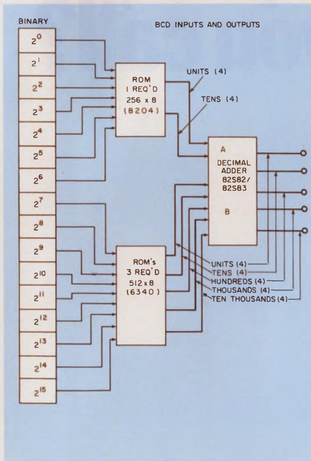
5. Binary numbers can be converted to BCD by the use of BCD decimal adders. This approach reduces part count and increases conversion speed. A 16-bit binary number converts to a five-digit BCD number in about 220 ns and uses approximately nine circuit packages.
