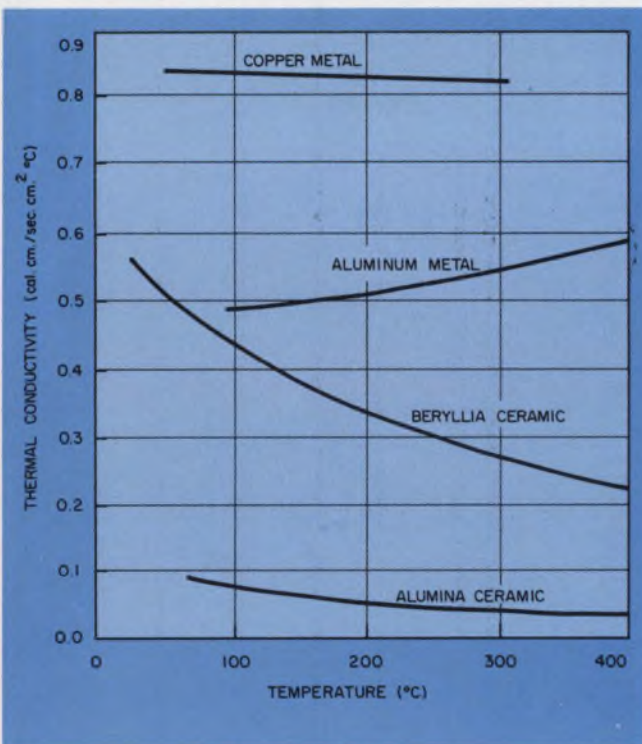
2. The thermal conductivity of beryllia ceramic is about six times that of the alumina ceramics at room temperatures. This advantage decreases at elevated temperatures. The curves shown are for a 99.5% beryllia and alumina. A major use of beryllia is in heat sinks.
