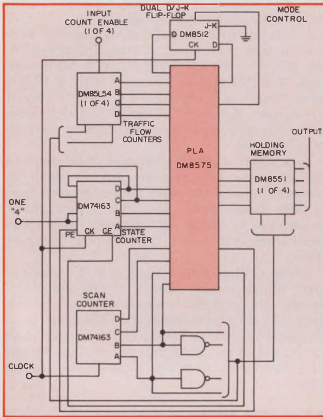
6. The PLA controls the timing interval in this traffic-light controller. The controller handles traffic flow in any of four directions and can start the control sequence from any state.
