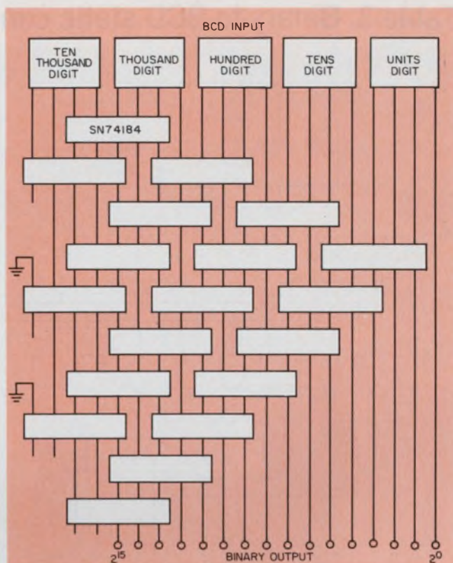
3. A five-decade BCD number can be converted to a 16-bit binary number with 19 SN74184 ROM packages. Conversion time is only 400 ns.
