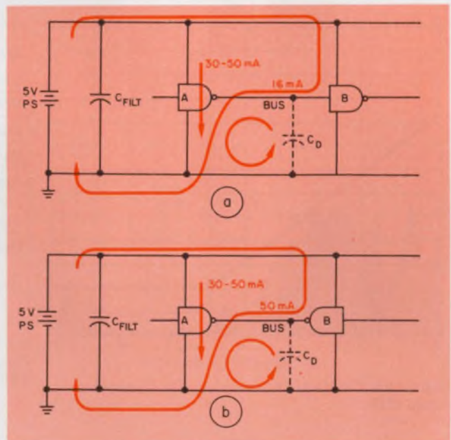
1. Very similar transient currents arise in both TTL (a) and TSL (b) when gates with opposite states turn on simultaneously on the same bus. In the TTL system, gate B represents all loads driven by gate A. In the TSL system, gate B represents all other TSL devices connected to the bus.
