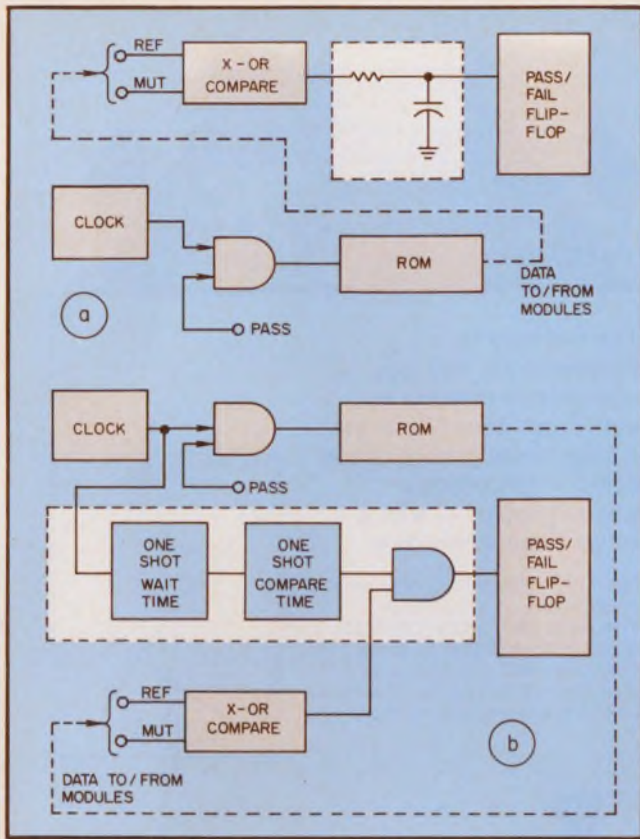
5. A simple RC circuit delays a pass/fail judgment after a test-sequence step until the voltages settle (a). The delay is generated by two one-shots (b).
