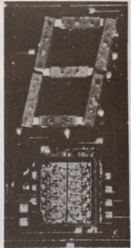
Basic display module consists of a seven-segment GaP LED and seven-bit, serial-input, parallel output shift register.
