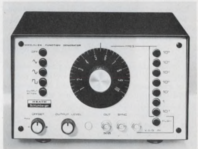
One of the lowest-priced function generators, Heath's EU-81A, delivers 100 mHz to 1 MHz and costs $245.
