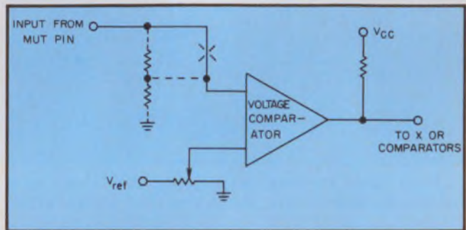
4. A voltage comparator is used to verify logic levels. Its threshold level is set by the adjustable potentiometer on the reference side.
