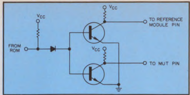
3. Two transistors provide an interface between the ROM and the modules and also isolate the MUT and reference-module inputs from each other. A failure in one module cannot affect the other. Without such isolation, some failure modes will not be detected.
