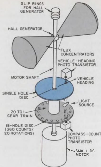
Hall sensor and photo-optical disc are spun by motor to give a direct digital readout of compass angle.
