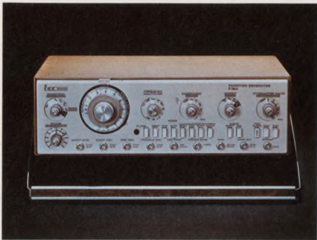
The output frequency of the F55 from Interstate Electronics Corp. can be phase-locked to an external periodic signal. This instrument—for 500 \mu Hz to 10 MHz—costs $1195.
