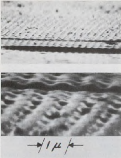
The surface of a holographic tape is shown in these photomicrographs taken with an electron microscope.
