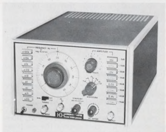
Pulse width and triangle slope can be set independently of rep rate in Krohn-Hite's 5400A, a $575 generator for 2 mHz to 5 MHz with voltage control of frequency over a 1000-to-1 range.
