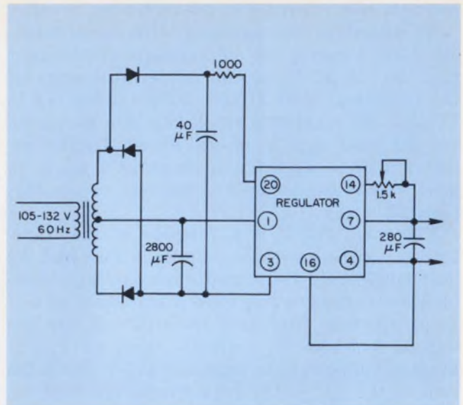
5. A more complex design for wide-range ac input calls for a smaller transformer and heat sink.
