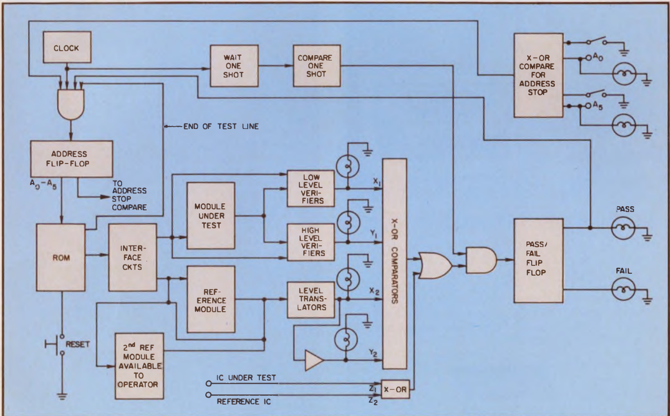
6. To aid troubleshooting, these features are included in the semi-automatic tester: lamps to indicate output
