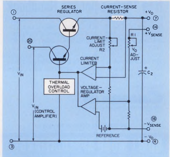
1. The basic hybrid regulator, designed for raw-dc input, has a power section (in white) and a control section. Circled numbers are package pin numbers.
