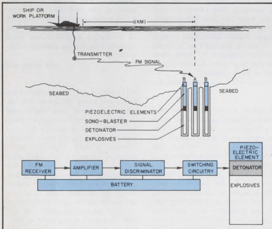
Transmitter suspended beneath surface ship sends FM signal to sono-blast-er unit A. The explosion activates piezoelectric elements in sono-blast-er units B, causing each in turn to explode.
