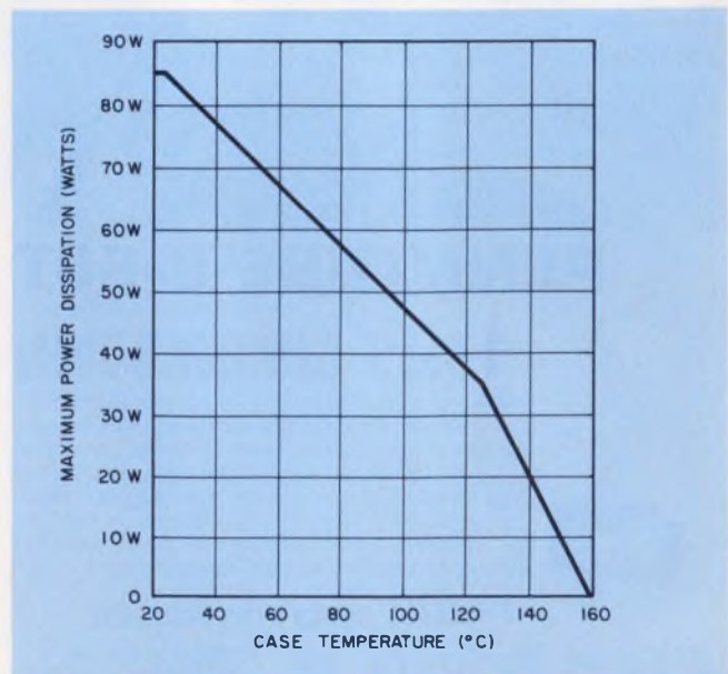
2. The maximum allowable power dissipation of the hybrid regulator goes down as a case temperature goes up, but the case can be cooled to boost dissipation.
