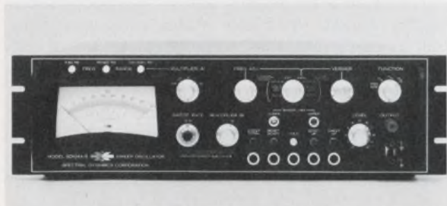
Intended mainly for sweep-generator functions, the Spectral Dynamics SD104A-5 provides linear or logarithmic sweeps of the basic sines, squares and triangles over 5 mHz to 100 kHz. Prices start at $1965.
