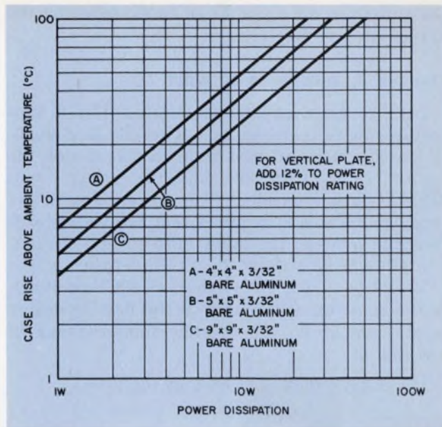
4. Typical heat-sink data for a horizontal plate. Another 12% can be added to the power-dissipation rating for a vertical plate and an additional 10% can be added if surfaces are painted.
