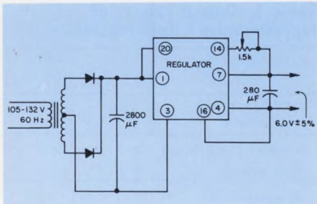
3. A simple approach to a design for wide-range ac input may not be as effective as the approach in Fig. 5.
