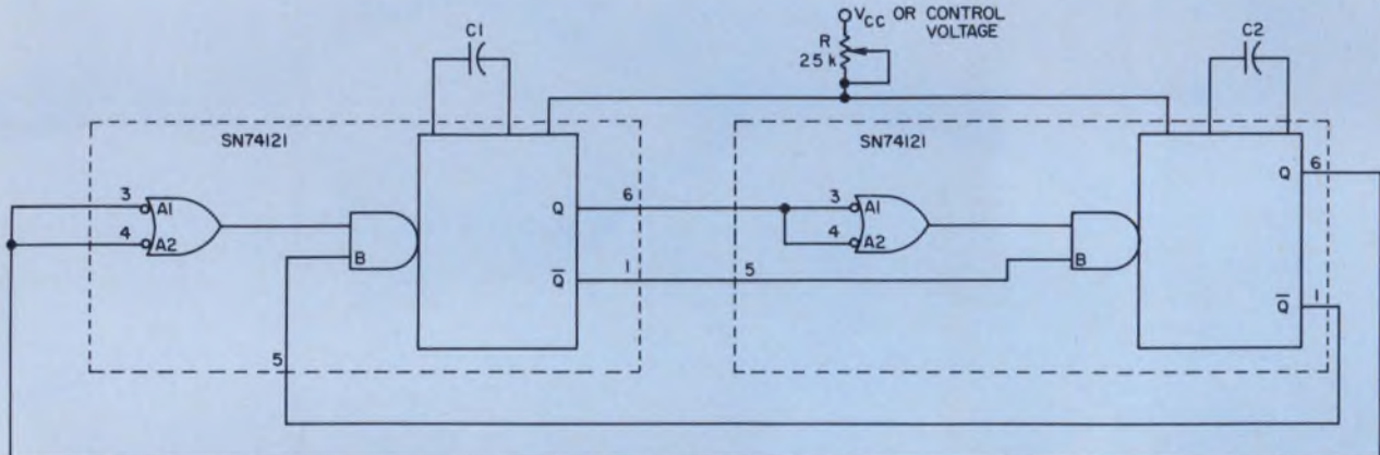
Multivibrator and truth table for logic inputs, where t_n is the time before and t_{n+1} the time after
