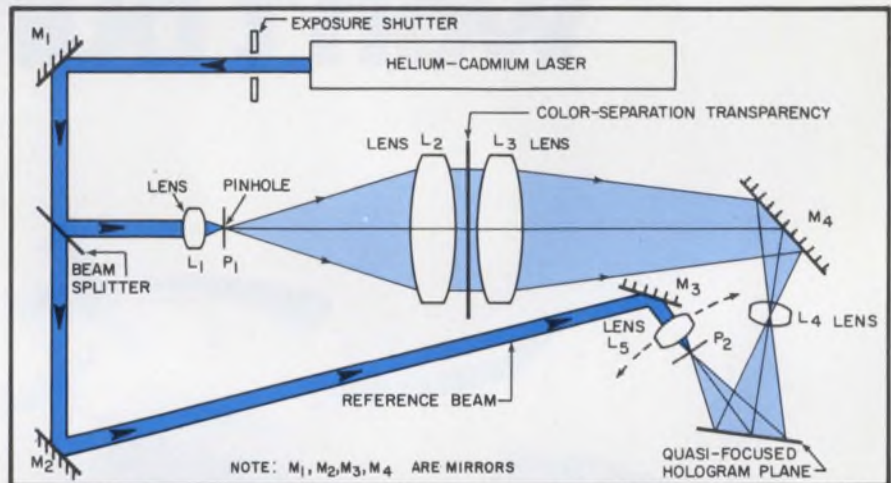
Three color-separation transparencies are recorded with this system as three overlaid holograms on a common photoresist area. Each hologram is made with the reference beam positioned at a different angle.
