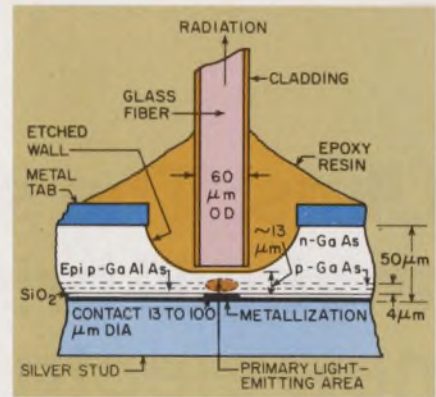
6. Fiber optics transmission lines will require emitter diodes, like the one above, fabricated by Bell Labs.
