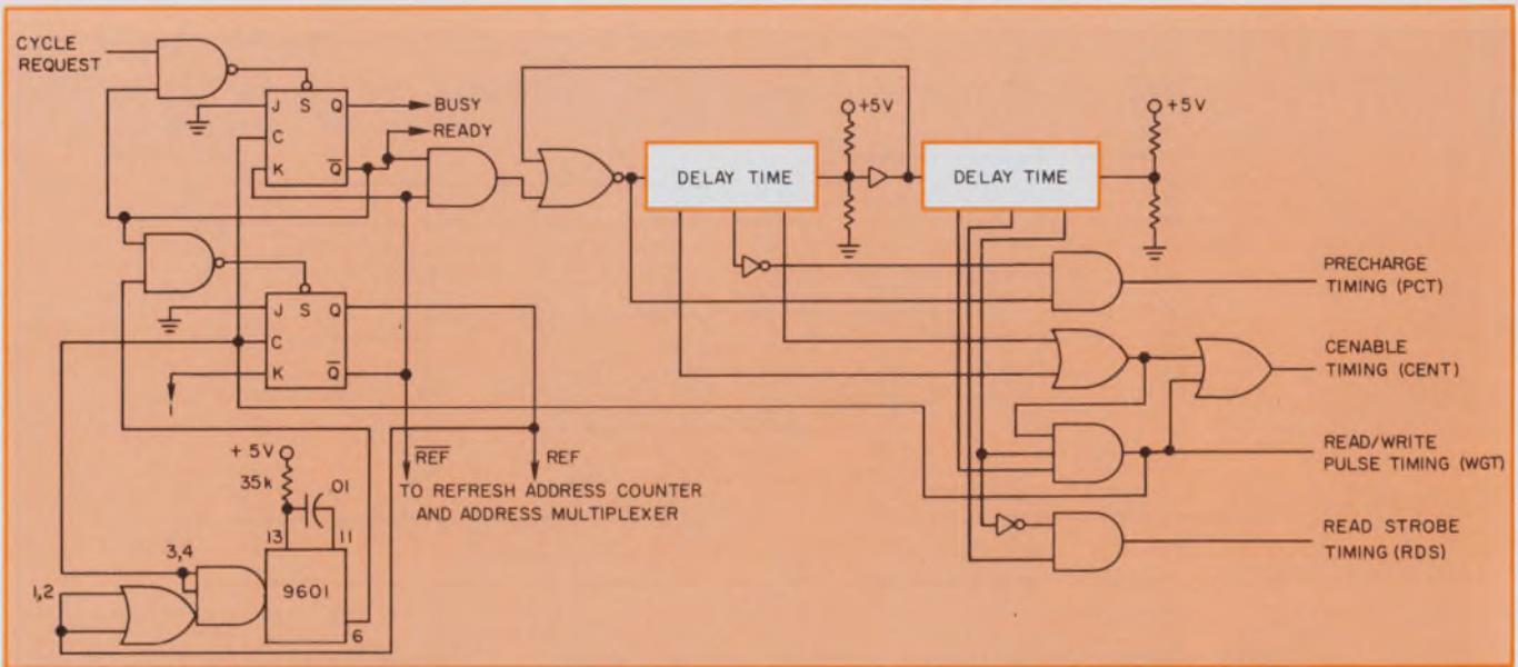
3. Controller uses delay lines to produce cycle timing signals. A refresh cycle generated by a single-shot multivibrator is requested every 60 \mu s. The timing of
