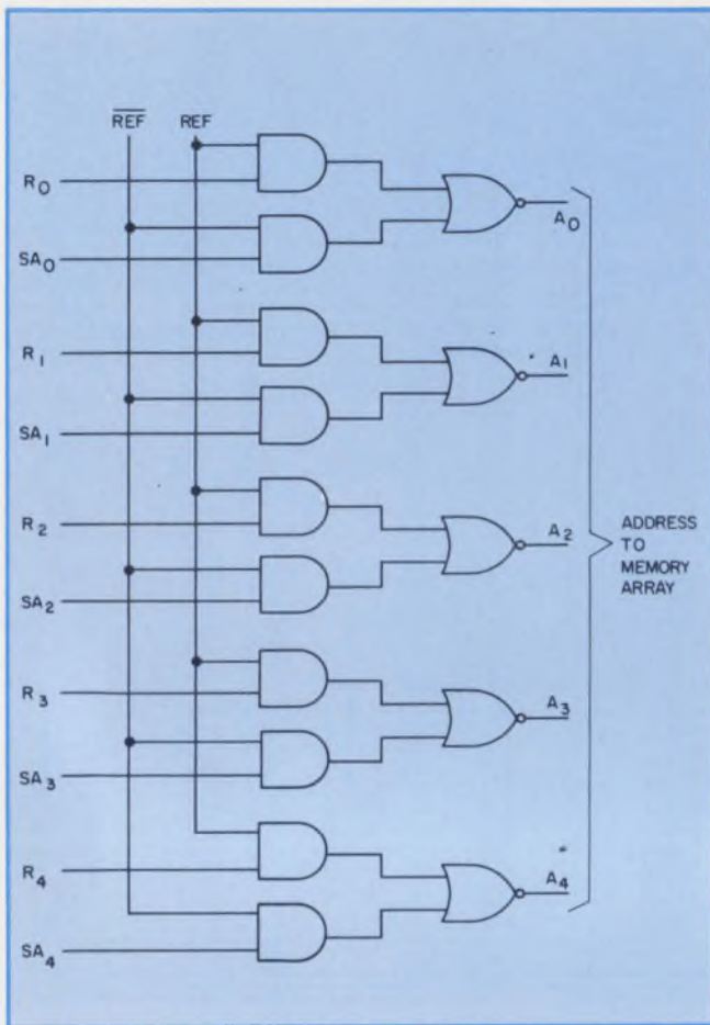
6. Refresh address switching circuit selects a five-bit address ( R_0 through R_4 ) from an address counter for refresh cycles, or from a memory address register ( SA_0 through SA_4 ) for normal requests. REF line selects the input. Only the row-address lines A_0 through A_4 are switched during refresh cycles.
