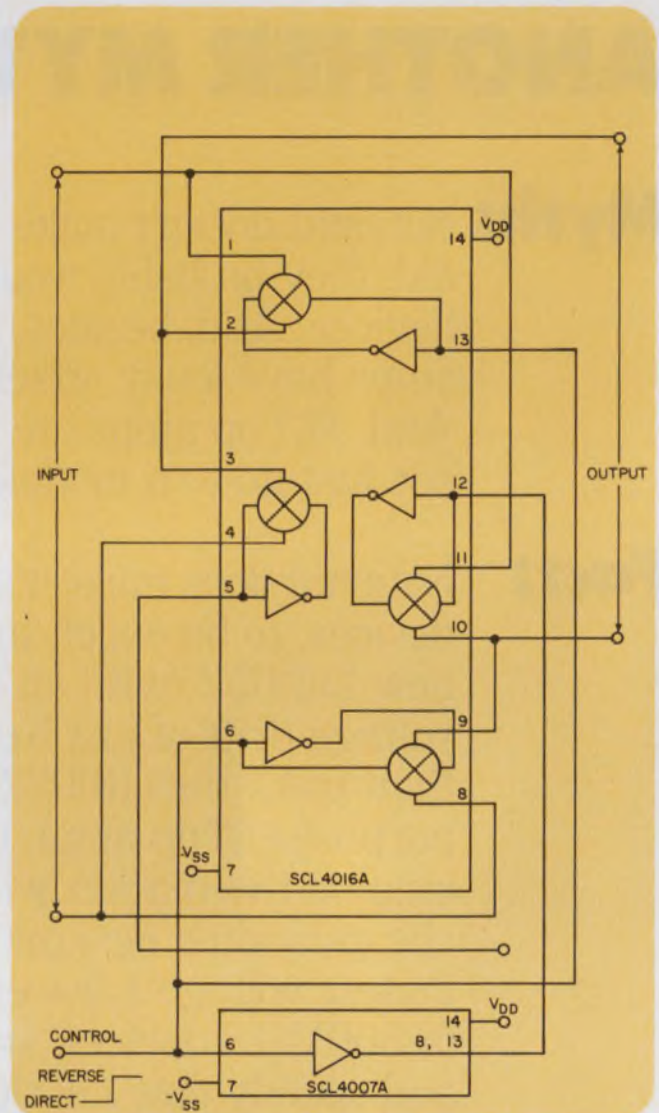
An SCL4016A quad bilateral switch reverses the polarity of analog signal inputs, with an SCL4007A acting as a control-signal inverter.
