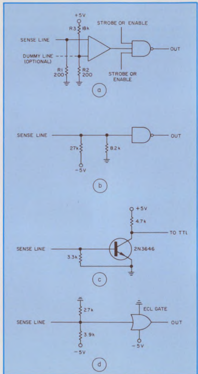
1. A balanced-input sense amplifier converts the 1103 current output to TTL logic levels. R_2 and R_3 provide threshold bias. The optional dummy line return reduces noise coupled into the data-output line (a). The lower-power TTL element is biased for direct sensing of output (b), and here a discrete transistor does the sensing (c). The circuit converts to ECL levels (d). Note that the higher impedance inputs in b, c and d increase system delays.
