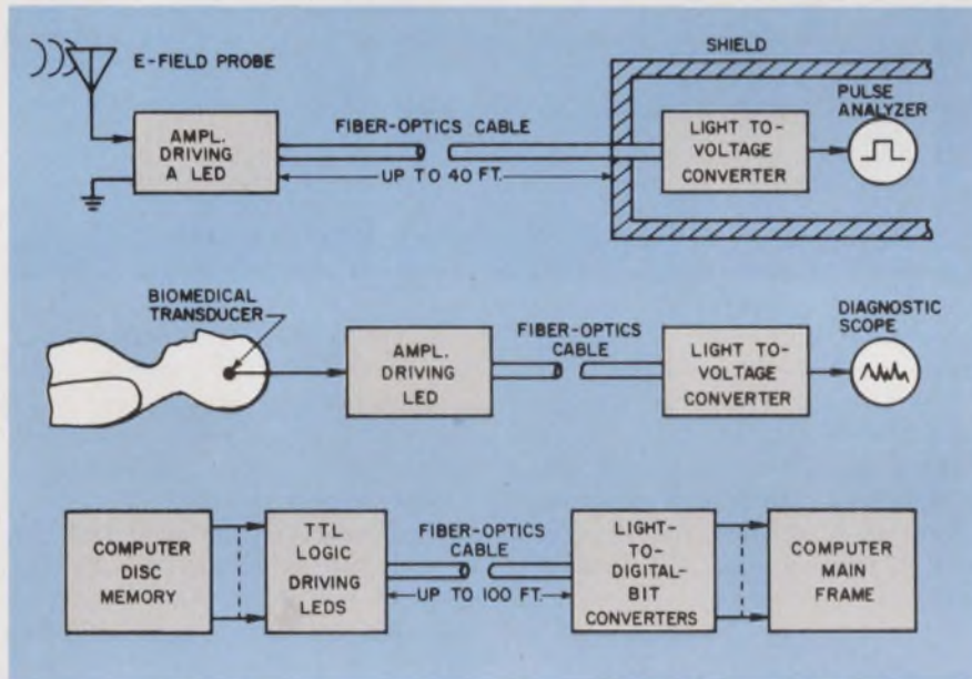
4. Representative applications of instrumentation and data transmission systems using fiber optics cables for information carriers. The two top applications are by Emtel Systems, the bottom by Quadri Corp.
