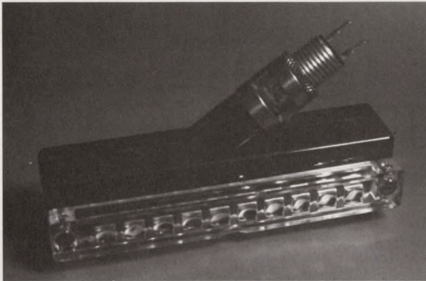
3. A fiber optics light distributor for an optical keyboard by Electro Fiberoptics Corp. uses plastic lenses to focus light from the fiber bundles down 11-inch channels. Key-operated shutters pass the beams to photosensors.
