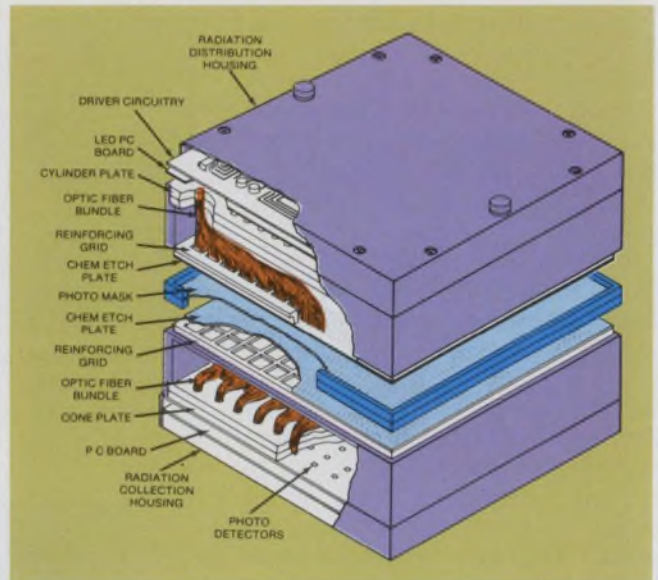
fiber bundles, left, are potted in position over photosensors. The basic mask area is about 5 x 5 inches with a storage density of about 4000 bits per square inch.
