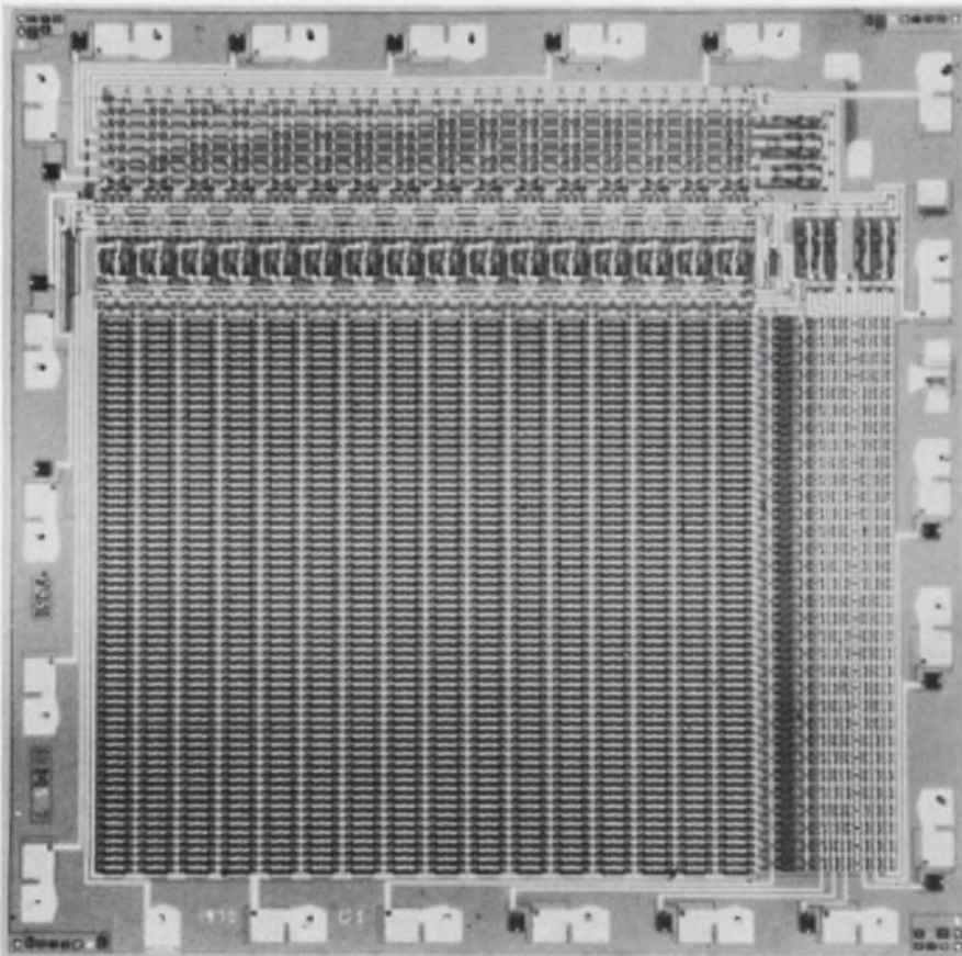
The only single-transistor-per-cell memory array to reach the commercial market so far is General Instrument's RA92048 dynamic, MOS, 2048-bit RAM. Other MOS firms are using a similar design approach.
