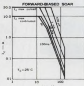
1. SINGLE DIFFUSED MESA (linear SOAR I_{s/b} )
