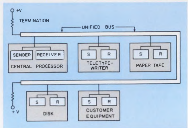
1. Error-free operation of a digital system depends heavily on the proper design of a "unified bus" that interconnects the various system components.
