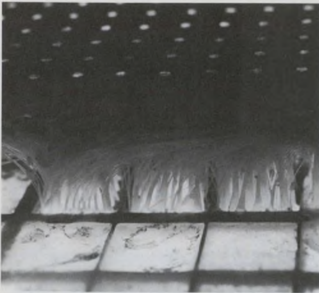
3. Fiber optic bundles in Quadri Corp.'s new memory carry light from gallium arsenide LEDs to photosensors exposed to the bit pattern in a photographic mask. The
