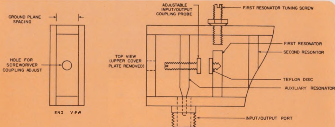
Capacitive probe allows fine adjustment of input/output coupling in interdigital bandpass filter.
