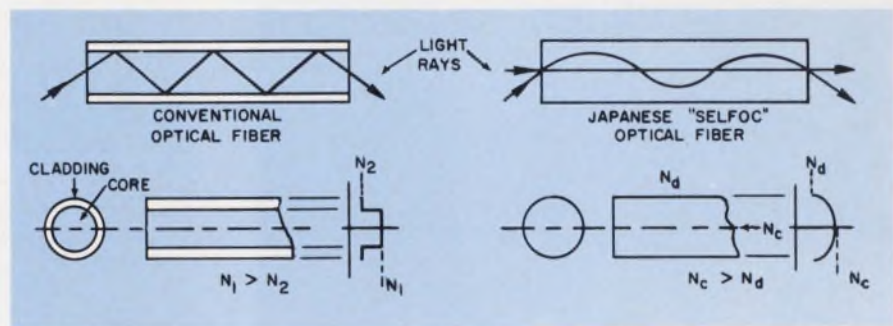
1. The conventional optical fiber has a core surrounded by a cladding of lower refractive index. The Selfoc fiber has a refractive index of continuous variation, with a maximum at the center and minimum on the outside.
