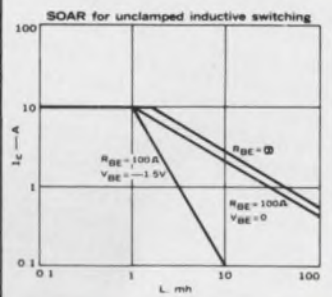
3. TRIPLE DIFFUSED PLANAR (excellent inductive switching E_{s/b} )
