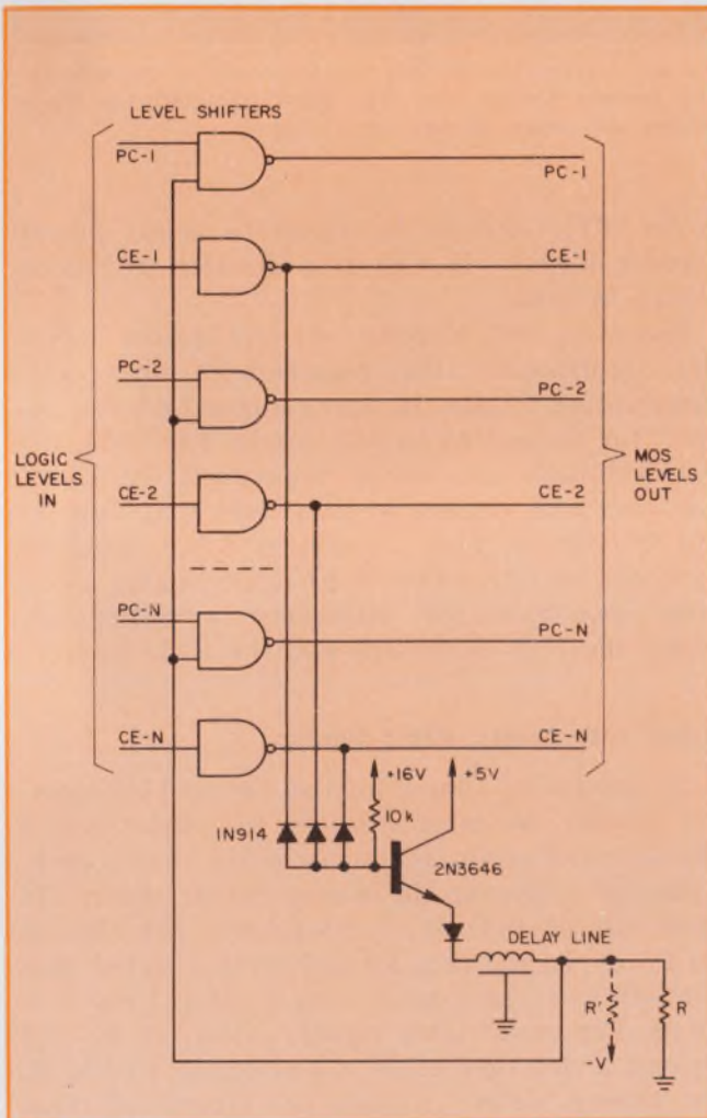
4. Timing generator reduces the number of gates in the path. The "c" enable (CE) turn-on pulses at the 1103 output are delayed and used to turn off the precharge (PC). All CE and PC pulses in the array connect to an OR circuit to actuate the PC timing from the actual CE pulse in operation.
