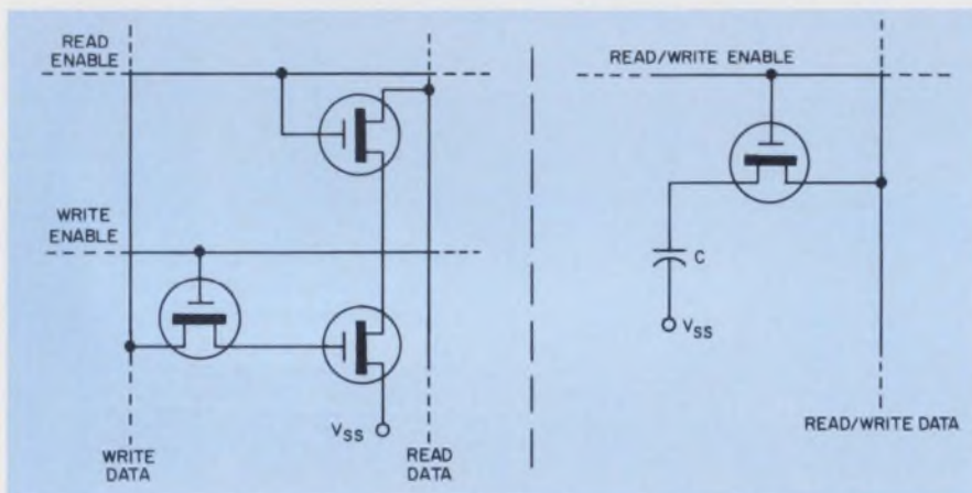
1. A comparison of the design of the Intel 1103 memory cell and the single-transistor cell shows that not only is there one transistor vs three but also only one I/O line instead of the two in the 1103 cell.
