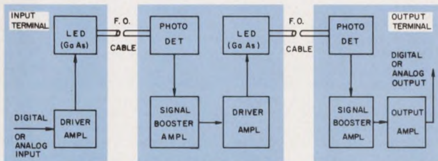
5. A proposed fiber optics communication system using repeaters to overcome losses in the fibers. The data or analog signals are applied to a modulator-driver amplifier feeding a gallium-arsenide LED.
