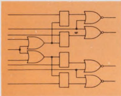
MC10133 Quad Latch — Consists of four bistable latch circuits with D type inputs and gated Q outputs. Latch outputs are gated, allowing direct wiring to a bus. All four latches may be clocked at one time with the common clock, or each half clocked separately with its own clock. Useful as a temporary storage element in high speed central processors, accumulators, register files, digital communication systems and instrumentation.
