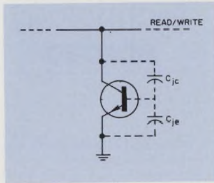
2. The Bell Laboratories bipolar cell is the simplest of all in basic design.
