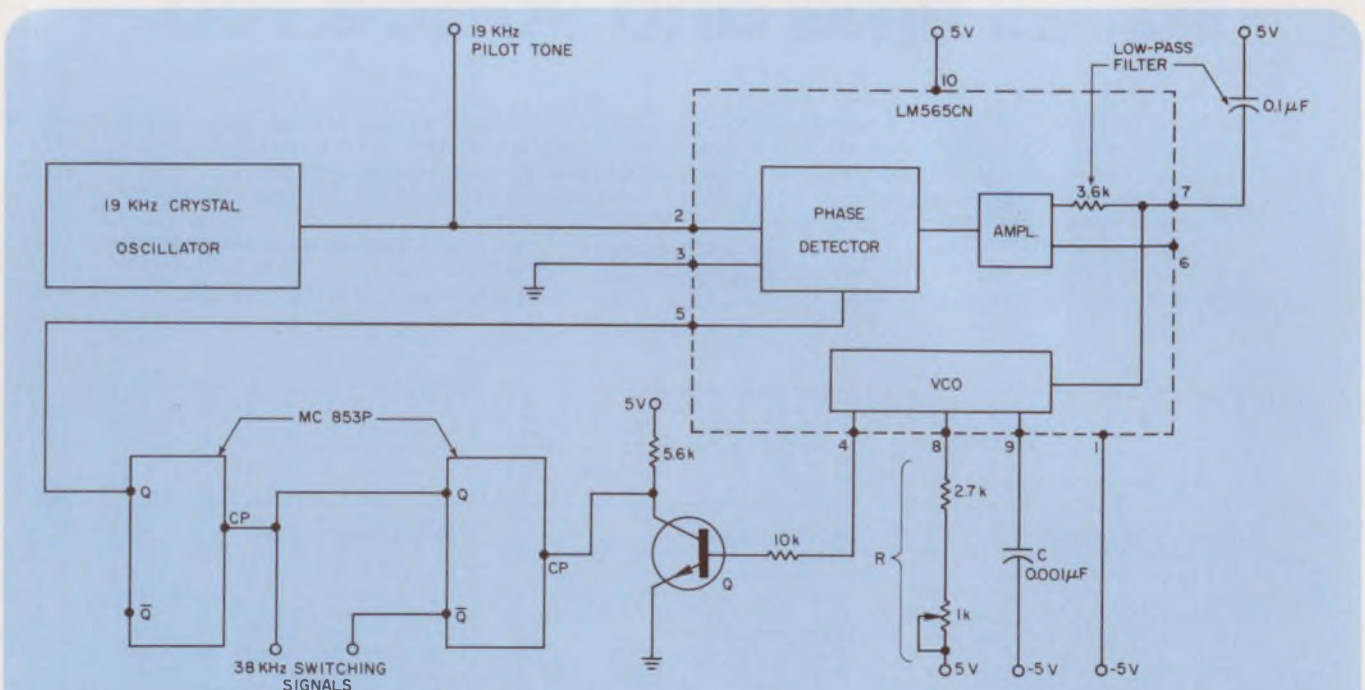
An integrated PLL, the LM565CN, driven by a 19-kHz crystal oscillator, is used as a frequency multiplier. Use of the PLL insures that the 38-kHz
