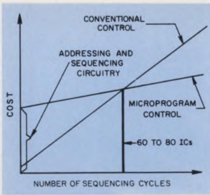
3. The cost per-sequencing-cycle of conventional control rises four times as fast as microprogram control.
