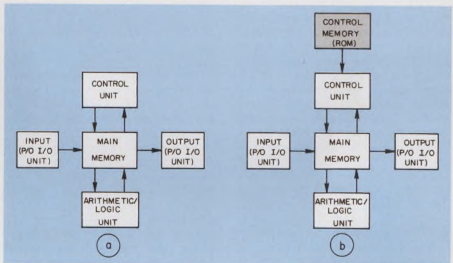
1. The significant difference between a conventional computer (a) and a microprogrammed computer (b) is in the addition of a control ROM.
