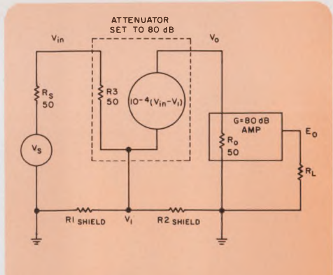
1. Gain equals attenuator setting when V_{in} = E_o in this standard test setup. The attenuator is shown in equivalent circuit form.
