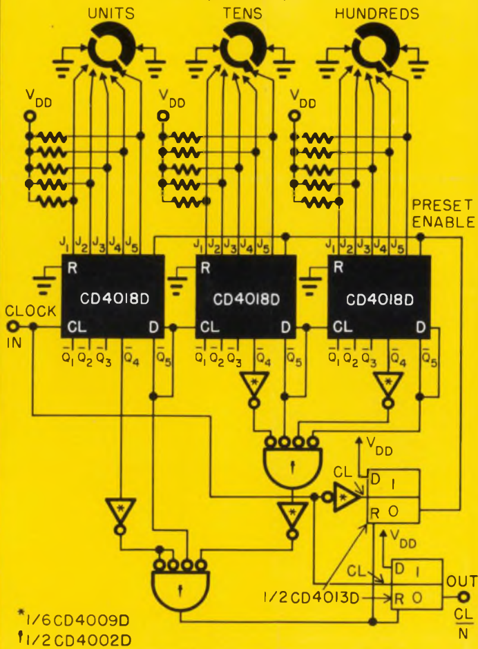
3-DECADE PROGRAMMABLE DIVIDE-BY-"N" COUNTER (N=2 TO 999)
