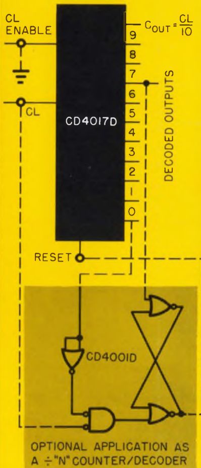
DECADE COUNTER/DIVIDER PLUS 10 DECODED OUTPUTS
