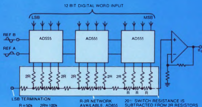
12-BIT MULTIPLYING D/A CONVERTER
