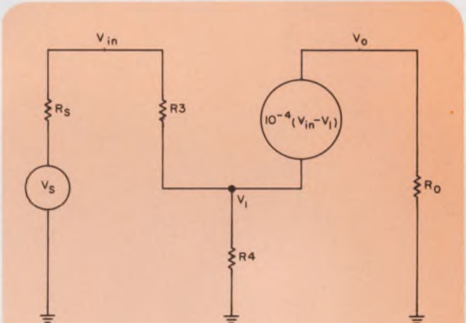
2. Parallel cable shield resistances are redrawn as R_4 to simplify circuit analysis. An R_4 of only 0.001 \Omega can cause a 1.6-dB error when measuring 80 dB.
