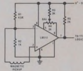
b. Detector for Magnetic Transducer
