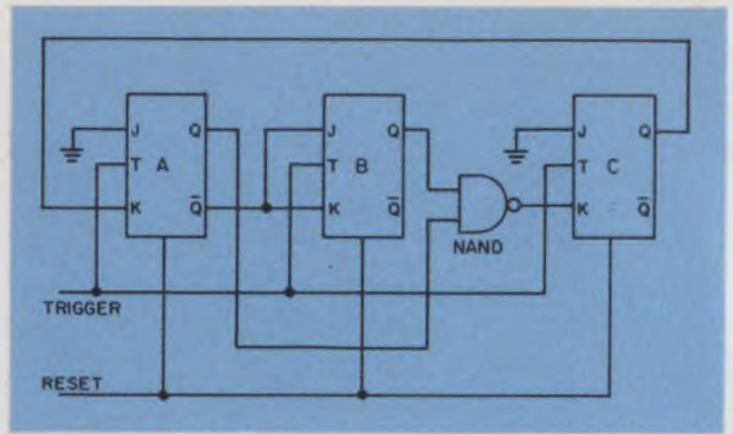
5. The counter schematic is derived directly from the Boolean expressions of Fig. 4.
