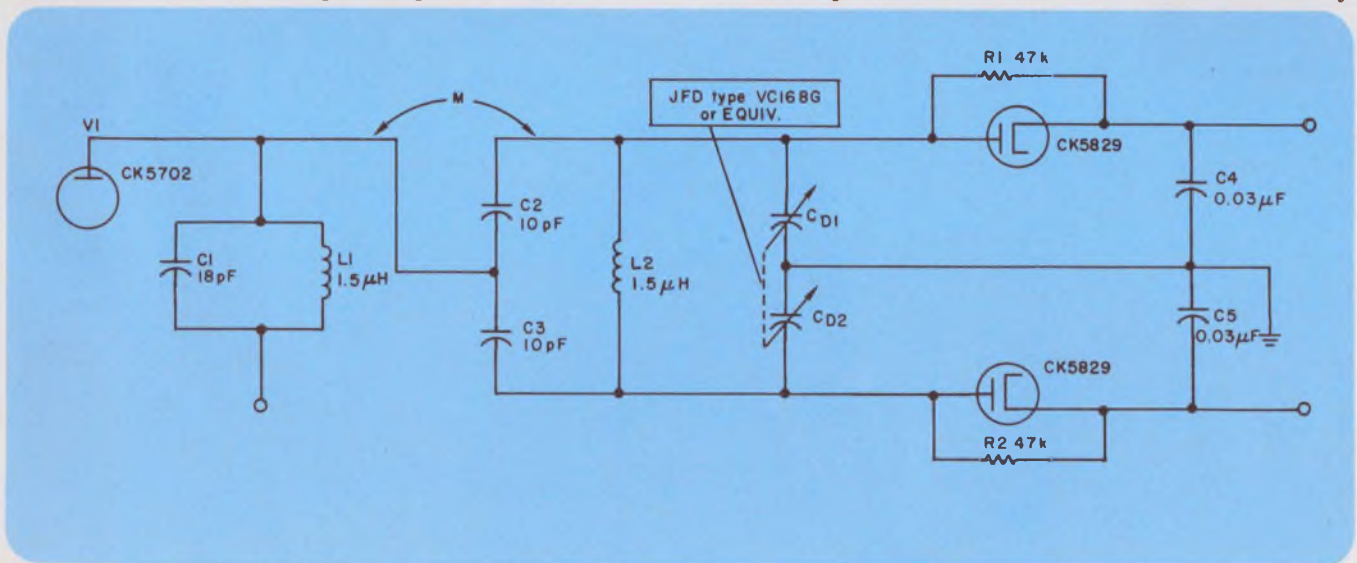
Discriminator with differential capacitor permits slope adjustment to close tolerances.
