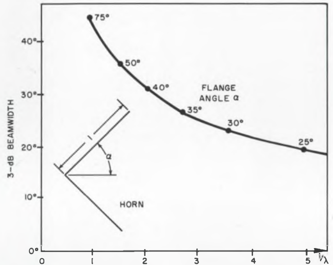
Curve for minimum weight in an H-plane waveguide-fed sectorial horn. The 3-dB beam width is measured in the plane containing the horn flare. The curve can also be used for the H-plane diagram of pyramidal and biconical horns.
