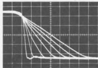
0.3V/cm, 5 ns/cm
