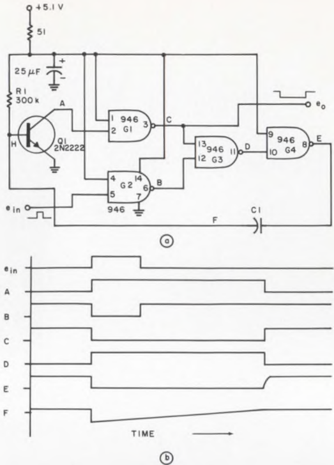
100-ms to 10-s pulse widths are obtained from this simple monostable (a) using DTL quad dual-input gate and a high-beta, low-leakage transistor. Circuit action is described in (b).
