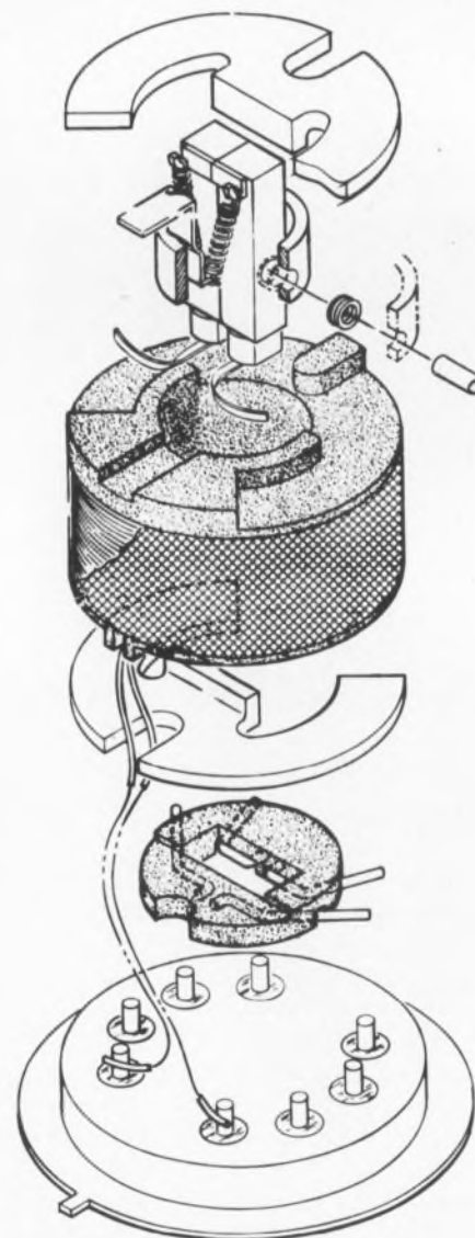
This exploded view of the TO-5 shows how the parts are arranged to achieve a 1 A relay in a can.
