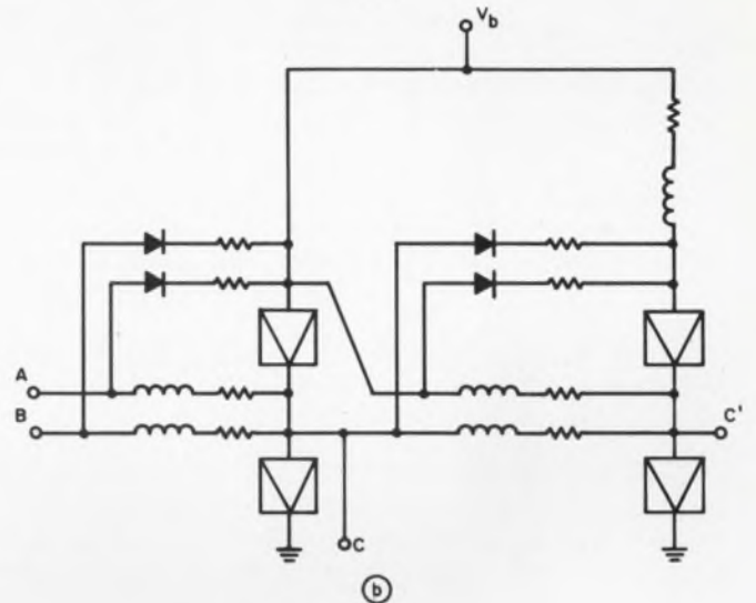
6. Half-adder with carry can be built with only two actrons. The truth table describes the operation.
