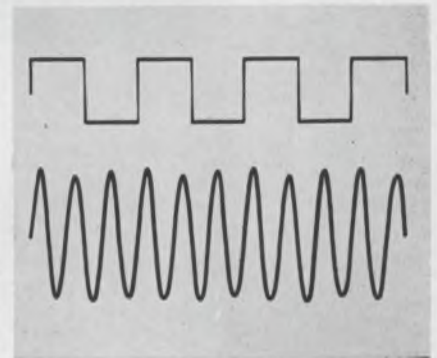
RECORDING ILLUSTRATES gain and selective response of Model 3342, in minimum band-pass operation, to a 0.01 Hz square wave. Output consists primarily of third harmonic component of input.
