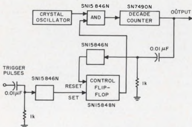
A constant-width negative pulse is generated for each trigger pulse. The accuracy of the circuit is a function solely of the crystal oscillator.
