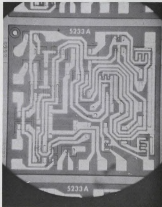
5. A practical integrated-circuit threshold gate under development at RCA indicates the possibility of a 50% cost reduction. This figure is obtained by comparing all production costs, including interwiring of the packages.
