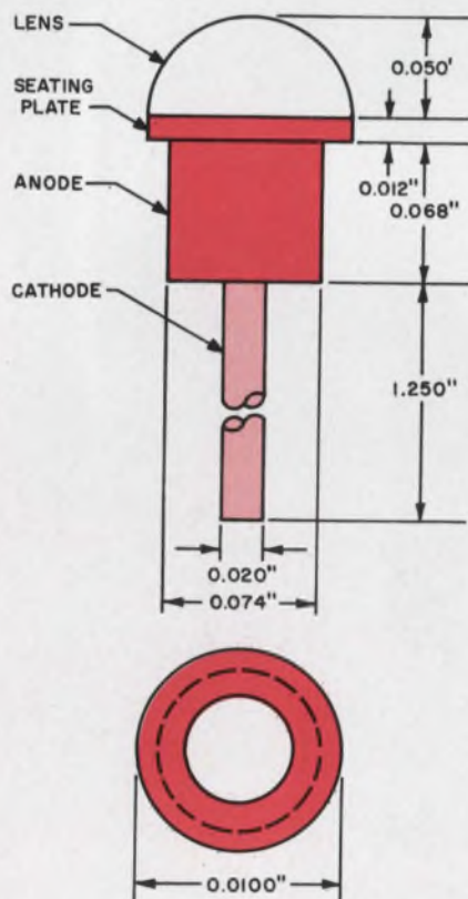
LEDs can produce 450 fL at 50 mA using gallium arsenide phosphide.
