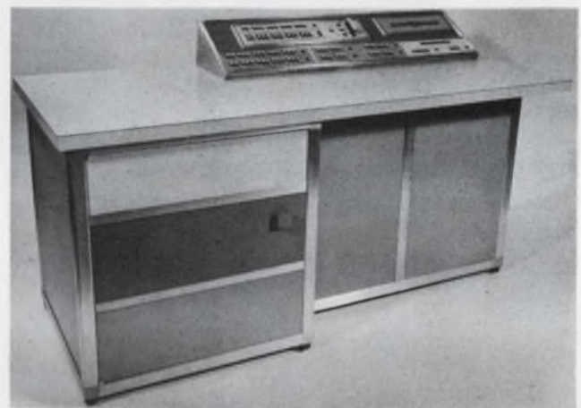
3. Gate reduction possible through the use of threshold logic was demonstrated in the design of this small, general-purpose computer built in 1964 at General Electric Research Laboratories. The results are summarized in the Table in terms of the gate requirements.
