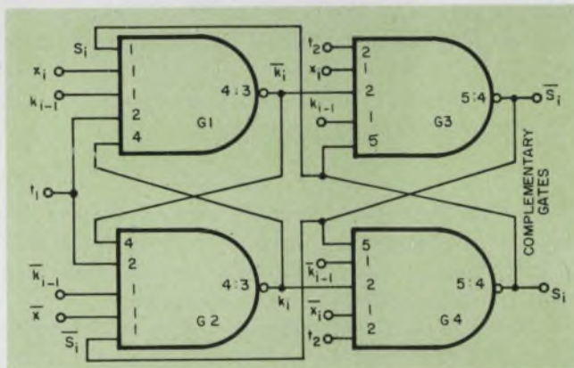
4. A simple accumulator is based on the two-gate adder circuit of Fig. 2a. Gates G 1 and G 2 form the carry flip-flop while gates G 3 and G 4 form the sum flip-flop. The circuit operates in two clock periods. During the first clock period (t 1 =1 and t 2 =0), the carry is computed by G 1 and G 2 and stored in the carry flip-flop while the sum flip-flop is unchanged. During the second clock period (t 1 =0 and t 2 =1) the carry flip-flop is unchanged and the sum is computed by G 3 and G 4 and stored in the sum flip-flop.
