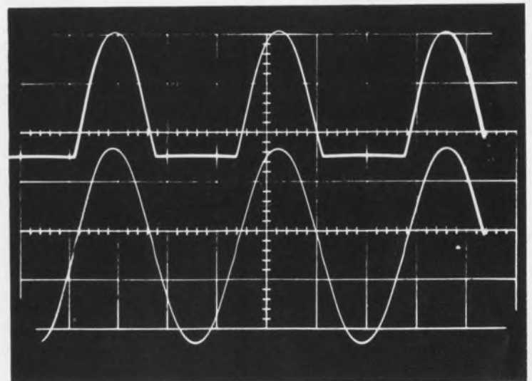
1. High-current and low-distortion core driver is possible with a single class-B stage (a). Test results appear in the table and current waveforms in (c). Even lower distortions can be obtained with the circuit (b).
