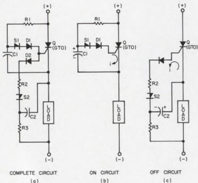
Square-wave generator circuit (a) is turned on and off by the action of Q, which is a gate turn-off SCR. The ON operation is shown in (b) and the OFF operation in (c).
