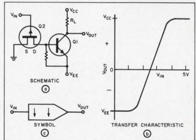
3. One J-FET and one transistor (a) amplify and shift levels (b) in response to a low-level input. Note the new logic symbol (c), with the arrows of Fig. 1 used to indicate the signal polarities when the driver is ON.
