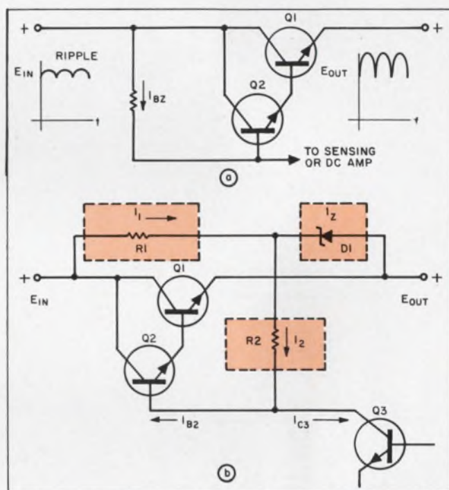
3. The preregulator filters ripple current from the input supply. The ripple is amplified by the series control element Q1 (a). Resistors R1 and R2 together with Zener diode D1 (b) make up the preregulator.
