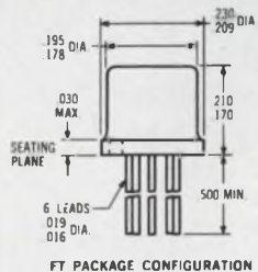
FT PACKAGE CONFIGURATION
