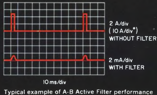
Typical example of A-B Active Filter performance
