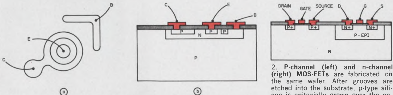
1. Lateral pnp transistor showing top (a) and representational cross-sectional (b) views. This one is made with existing semiconductor processes and no additional fabrication steps.
