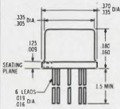
2N PACKAGE CONFIGURATION
