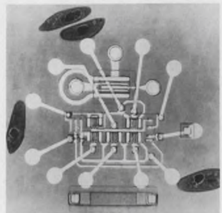
Paramecia, single-celled animals, dwarf the small-geometry transistors that make up this high-speed logic circuit with a switching speed of 400 ps, that was developed by IBM Components Div. researchers.
