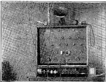
Note honeycomb coils used in this set.
