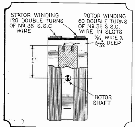
Q. 406. A baby coupler particularly adapted to compact sets is illustrated in detail above. Additional data is given in the text.
