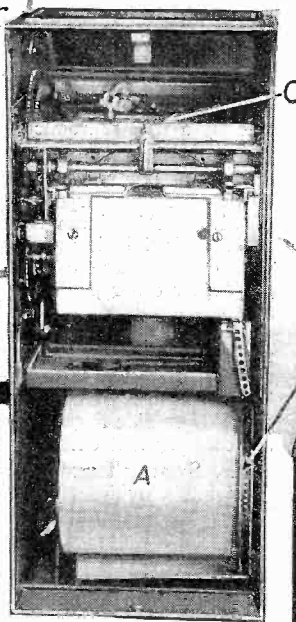
A new device for office use that makes paper cups individually as needed, has recently been placed on the market. No manipulation on the part of the operator is necessary other than the pressing of a button and the turning of a crank. The complete operation is otherwise automatic.
