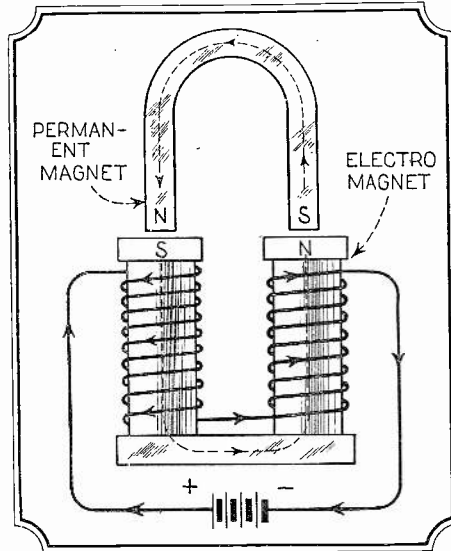
Permanent magnets are made by magnetization by a large electro-magnet as above.
