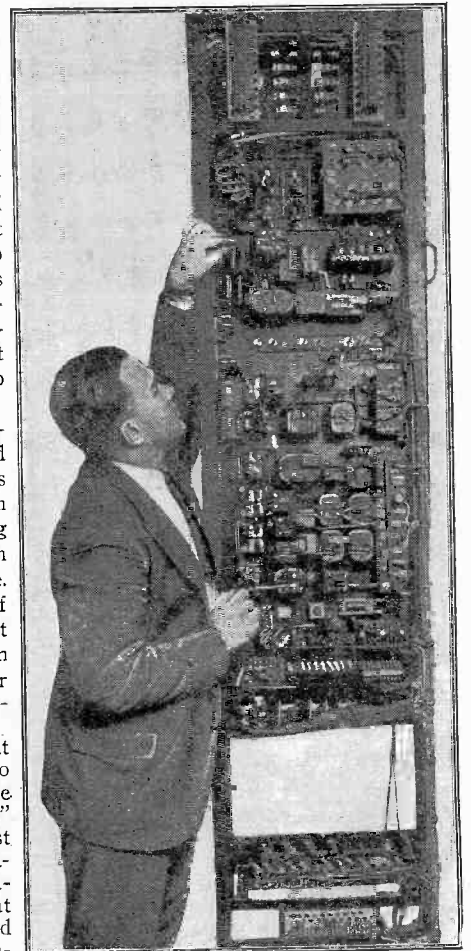
A rear view of the control panel with its various metallic shields removed is shown directly above. This is the same panel that Mr. Maresca is shown in front of in the photograph on the extreme left-hand side of this page.
