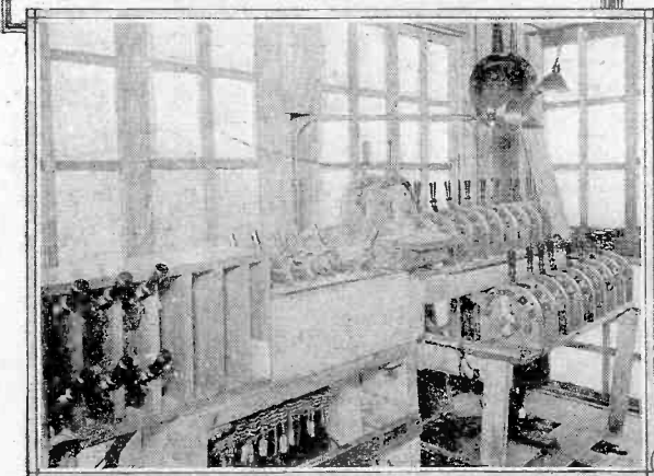
7 At the extreme left of Fig. 7 the controls are shown which enable the operator to apply the skates illustrated in detail in Fig. 5. Some of the other controls serve to manipulate the switches for selecting the track upon which the car is to be placed while the remainder actuate the retarders.
