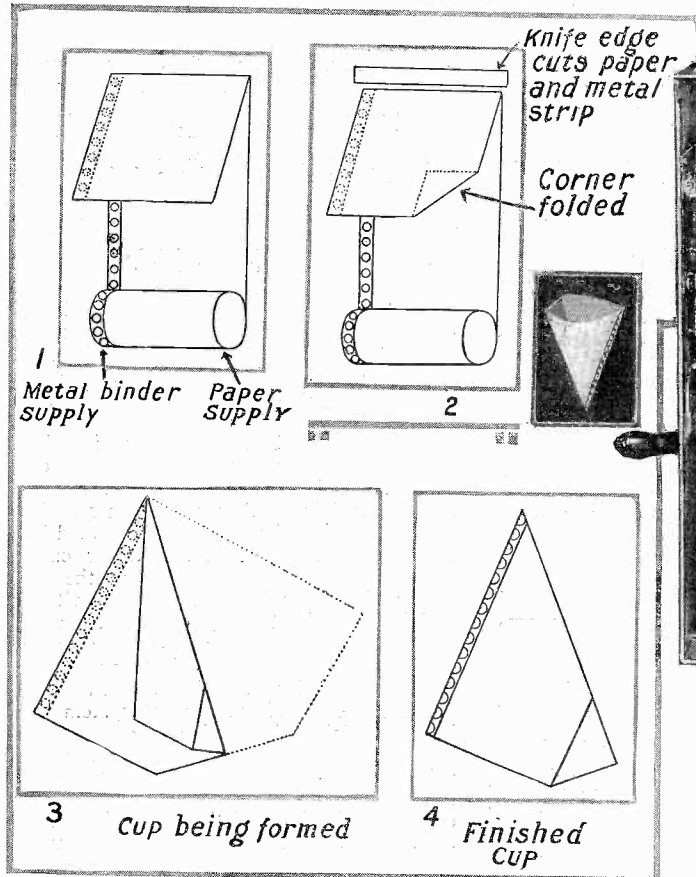
The four main steps in the forming of a paper cup are shown above and the shape of the finished product may be seen in the insert. The paper roll and metal binder supply are side by side and are fed up through slots to the position shown in 1. The paper is then cut and one corner folded over so that the edge will not cut the mouth of the user. An arm carries the paper over as at 3 and a crimping part produces the result as at 4.
