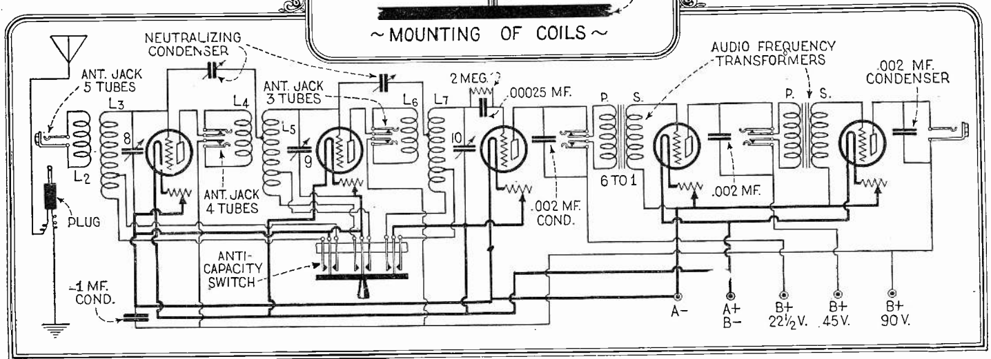
The complete circuit diagram shown above illustrates all of the connections for this six-in-one receiver; the antenna and ground are connected to a plug
