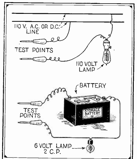
Two simple yet handy test circuits are shown in the illustration directly above.
