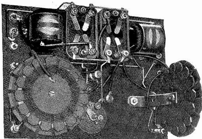
Note the very compact arrangement of the instruments used in this two-tube portable receiver. The writer has had wonderful success with this set and you can duplicate it by following instructions.
