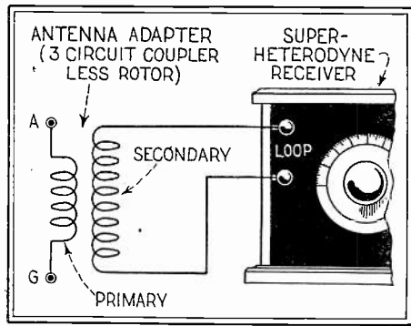
Q. 399. An antenna adapter for use with super-heterodynes is simple to hook up as shown in the above illustration.
