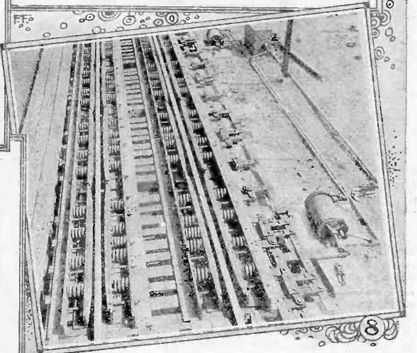
8 In the general view of one of the car retarder sections of this switching system that is shown directly above, the electro-pneumatic release and applicator can be seen to the right of the track. The heavy springs and friction bars of the retarder are also plainly shown.
