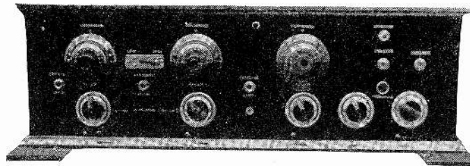
A front view of this rather simple yet very efficient and flexible five-tube receiver is shown in the photograph directly above. Note the wave-length change switch that is located between the first and second dials. A plug and jack arrangement makes it possible to use from one to five tubes on any desired wave-length between 200 and 600 meters.
