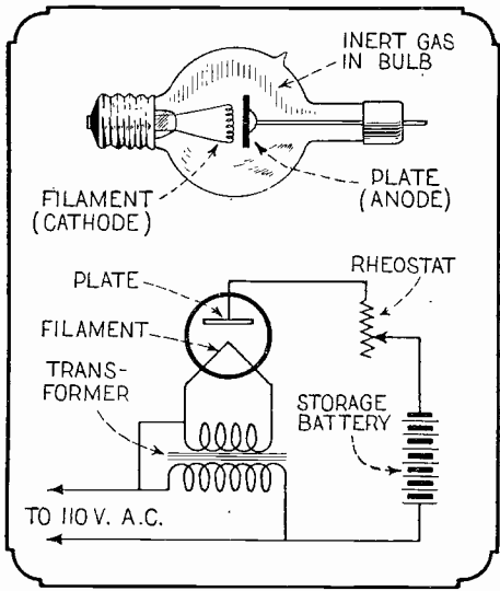
A view of a rectifier bulb and the circuit used with the same are shown.
