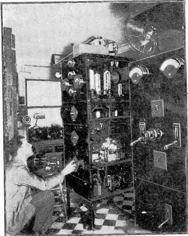
The photograph above shows Gilson V. Willets, manager of station WRNY, tuning the transmitter of that station preparatory to going on the air. The screens are removed from the sides of the transmitter frame in order to show the enormous tubes used. A wave-meter is at Mr. Willets' side.
