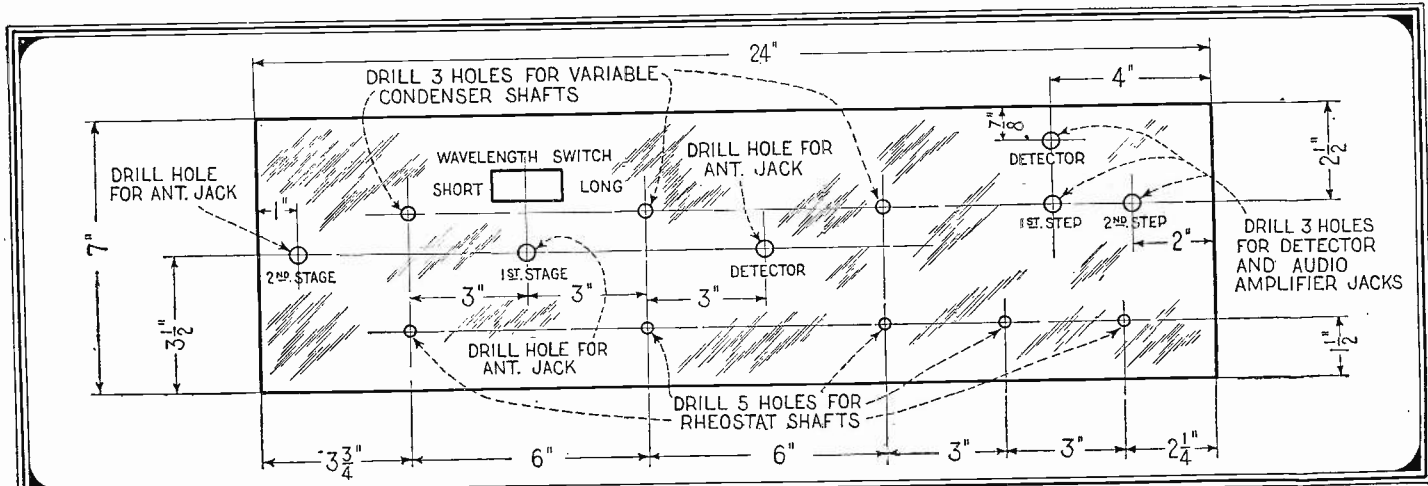
From the panel layout given above, you can readily make up your own panel and lay it out in the best possible manner. The panel that the author used
