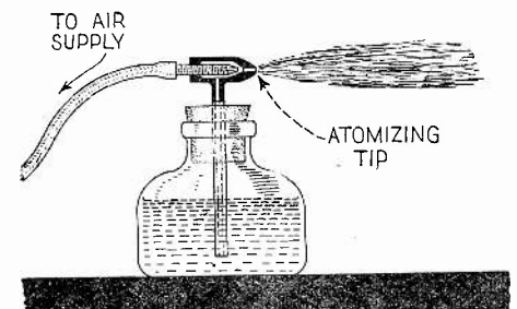
An atomizing burner is shown in cross-section above. See text for description.
