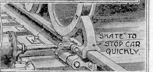
5 Fig. 5 above shows how a "skate" may be applied to the wheels of a car that has run wild. These skates are distributed throughout the yards and are automatically released. The portion on top of the rail is pushed ahead of the car, stopping it.
