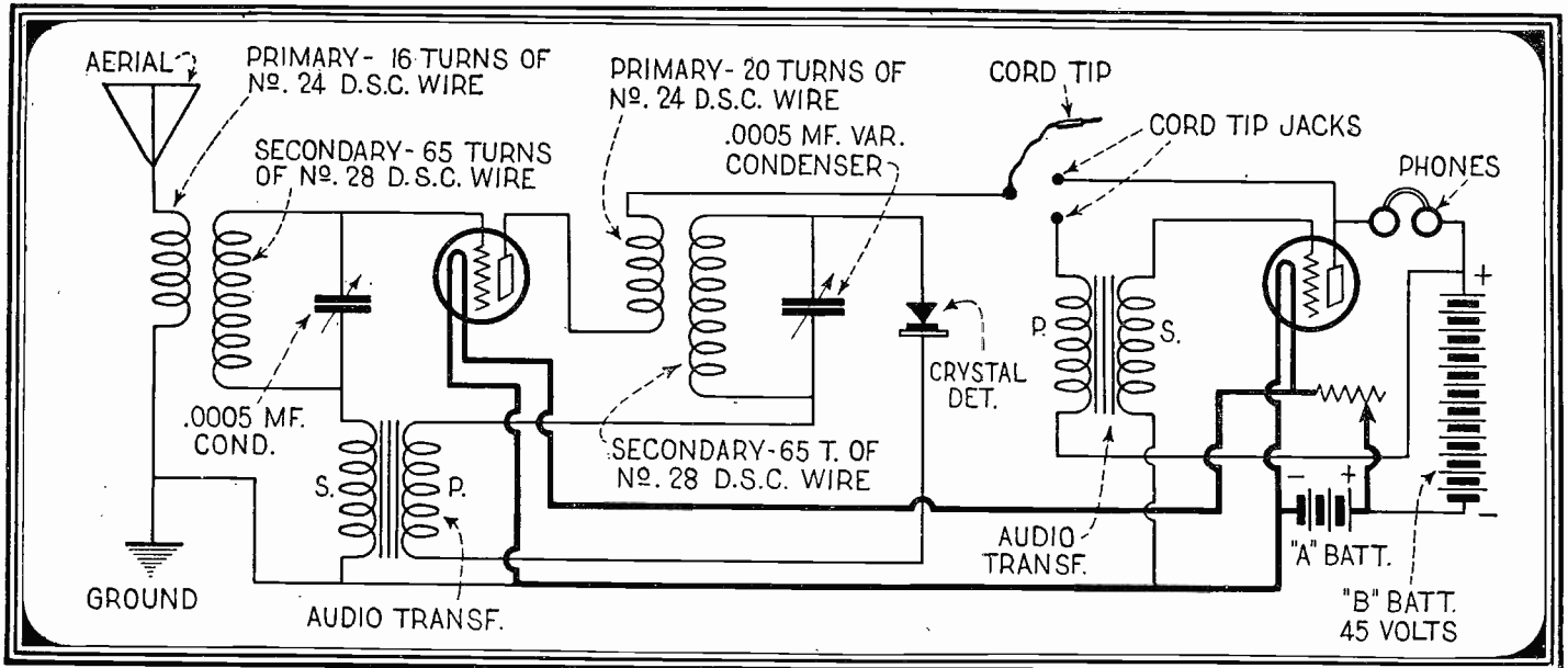
The circuit diagram of this highly efficient reflex circuit which, without any fixed by-pass condensers, gives excellent results, is shown directly above.
