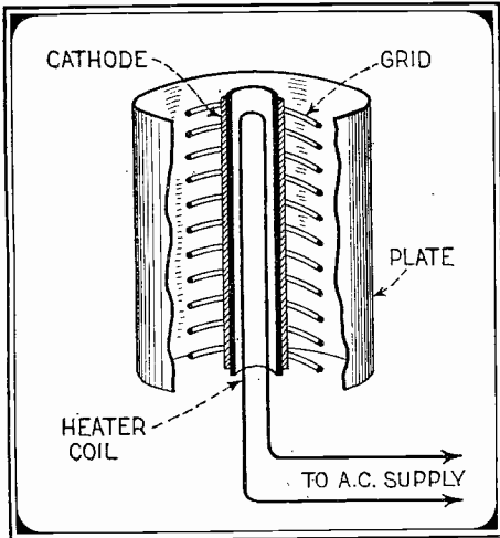
Q. 407. This diagram shows in simplified form the internal construction of a new vacuum tube that operates on alternating current.
