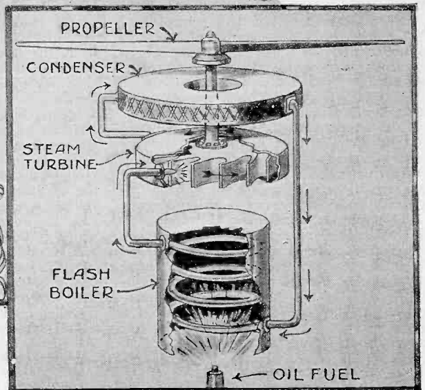
As shown in the two illustrations directly above, this new helicopter can alight in water when necessary, as the pneumatic landing cushions support it on water or land. Right: Details of power plant simplified.
