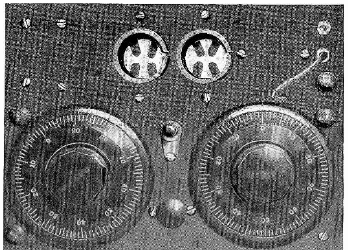
The front panel view of this set shows the plug and jack arrangement enabling the last tube to be cut out when not desired. Note the socket mounting and the position of the crystal detector.
