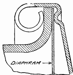
Loud speakers with adjustable diaphragms are most valuable because of their adaptability to various and changeable conditions. Illustrations at left and above show one type to be attached to a phonograph.
