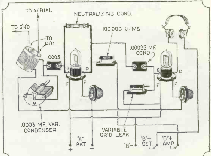
Neutralization can be applied not only to inductively coupled stages of radio frequency, but to resistance coupled amplifiers as well.
