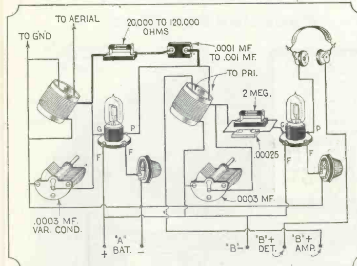
Later work by Ferrand who evolved the above, improved neutralized tuned radio frequency amplification. The idea is to introduce resistance in the circuit which has a decided tendency towards preventing oscillations. It must be remembered that an oscillatory circuit which has a high impedance introduced will not oscillate. If a resistance were likewise introduced in the plate circuit directly, a serious loss in signal strength would result.
