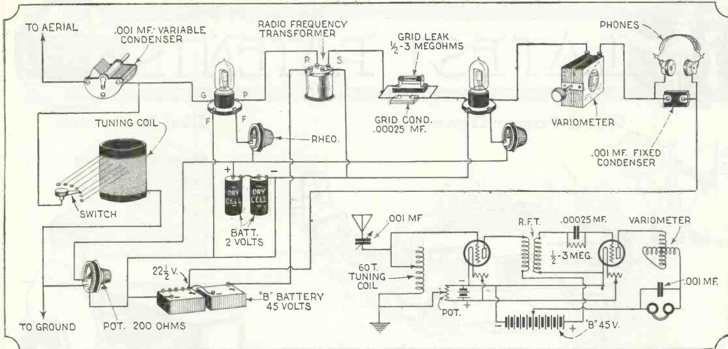
(Q. 313) The low capacity tubes such as the WD-12s work very efficiently as radio frequency amplifiers. The circuit shown is that of one stage of radio frequency and detector with regeneration. A stabilizing potentiometer is also employed.
