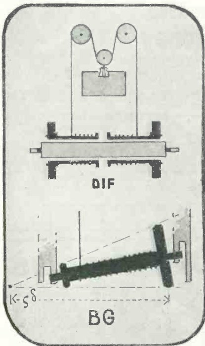
The picture above shows Hero's differential gear at "Dif" which works without a fixed radius, similar in principle to ours of today; while "BG" illustrates a fixed radius of the bevel gear.
