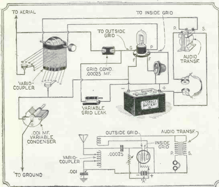
The wiring diagram of the set shows the new four element tube and the connections to it. Two concentric grids are contained within; by carefully adjusting the variable grid leak, maximum amplification can be obtained. This circuit is regenerative.
