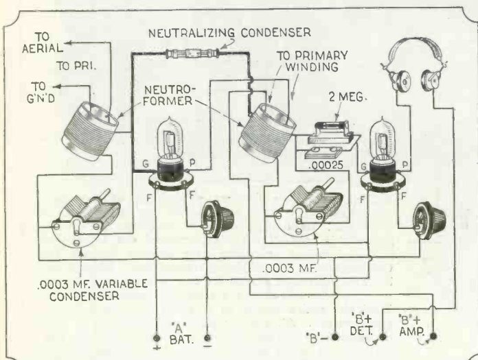
The original Hazeltine method of neutralization is depicted in the above diagram. It is known technically as condenser compensation.
