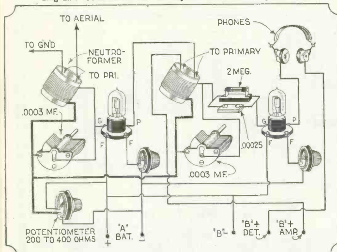
The fact that regeneration may occur in a radio frequency amplifier circuit is not a detriment, but what really is the objectional feature is the fact that self oscillation may be set up. Especially is this true where the plate circuit is tuned. Referring to the above diagram, the plate circuit is tuned inductively by the condenser across the secondary of the neutroformer. However, by the judicious use of a potentiometer, trouble is alleviated.
