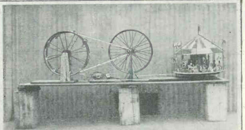
By connecting the various pieces of apparatus or toys by means of string belts the whole affair can be operated with a small toy motor. Above is shown a sort of toy circus ground set up on boxes and the various mechanical toys installed upon it. The motor may be seen between the two upright wheels at the left of the merry-go-round. The belt to the merry-go-round simply passes around the outside of the bicycle wheel. The wheel in the center of the picture is set on two wooden uprights, the axle of the wheel being fastened to it. Each of the toys is built in a unit to itself and can be moved independently of the others in the collection, thereby giving a means of adjusting the tension on the connecting belts.
