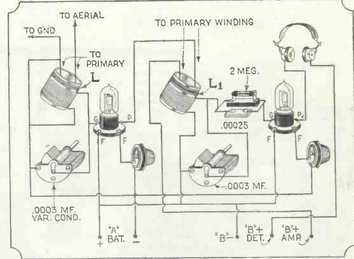
A more recent innovation in neutralized tuned radio frequency circuits is the introduction of a so-called compensating coil, which is an inductive closed circuit L and L 1 in the proximity of the coupling transformers. Its effect is to highly damp by means of its inductive effect, any tendency towards the creation of oscillations. The method is not very effective over a great wave-length range, but for a given band, works quite efficiently.
