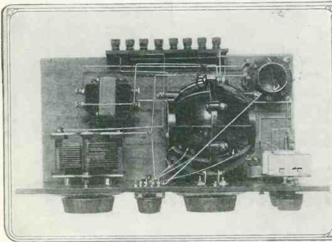
The above top view illustrates the arrangement of the various parts employed. The variocoupler has 60 turns on its primary, which is tapped at every 15 turns. In addition a .001 variable condenser tunes the primary circuit to resonance with the incoming wave.
