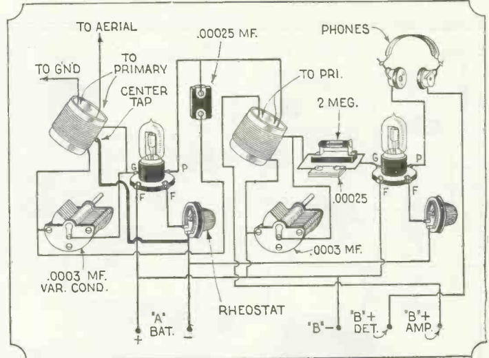
The Rice method of neutralization where the filament terminal of the tube is connected to a point which divides the inductance of the secondary circuit into two equal parts, is shown in the above diagram. This method, that of differentiation, is analogous to the Wheatstone Bridge. It was one of the first evolved in the attempt to obtain maximum regeneration without having trouble by encountering unwanted oscillations.
