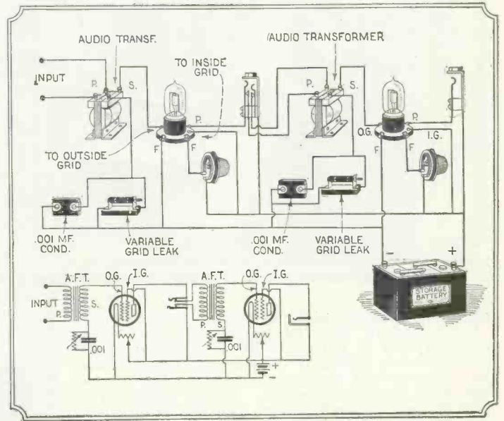
To increase the volume, a two-stage amplifier using Solodyne tubes is added in the same manner as the ordinary amplifier unit. The outstanding feature is the omission of the "B" batteries, thus affording tonal quality that cannot be obtained even with the resistance coupled amplifier.
