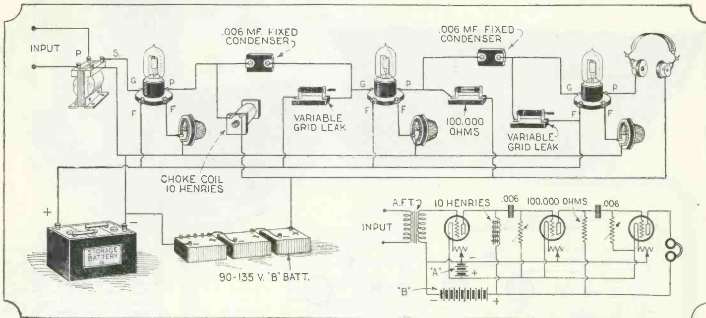
(Q. 308) The ideal audio frequency amplifier is shown herewith. As the grid potential in the succeeding stages of audio frequency amplifiers becomes greater than the tube can efficiently handle, distortion is the inevitable result. This circuit eliminates such distortion to a marked degree and it is the best practical arrangement.
