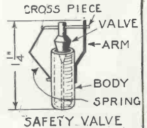
The detail of the safety valve is shown below. The piece of lead forming the valve is cut or filed as shown and fits into the top of a brass pipe which is soldered to the boiler top. The supporting spring can be made of brass wire.
