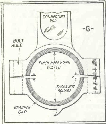
If the bearing is allowed to run in such condition as shown in sketch F and G, the bearing will soon wear and become noisy again.
