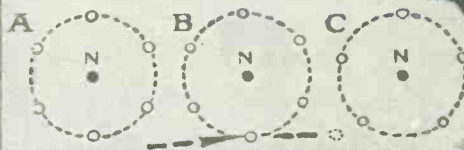
Immediately above is shown graphically how the bombardment of the mercury atoms tears away one electron, thus forming gold. N is nucleus, A mercury, C gold, with electrons rearranged.
