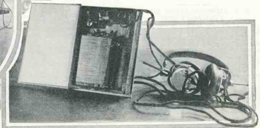
The complete crystal set is clearly depicted in the photograph at the right. The tuning coil is composed of 80 turns of No. 22 S.C.C. A slider alongside of it readily tunes it.
