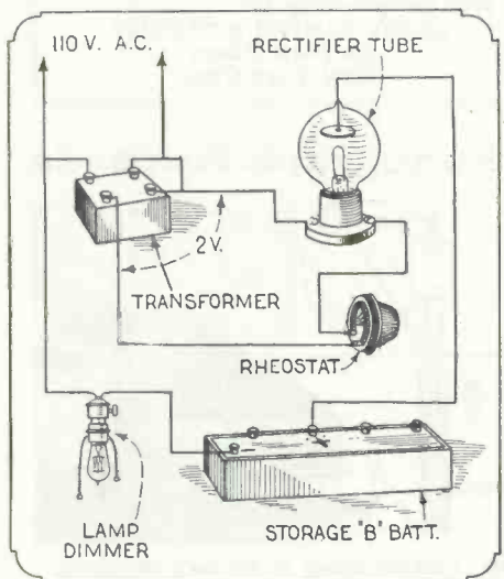
(Q. 315) The necessity for a special transformer in conjunction with a rectifier bulb for charging a 90 volt "B" battery is eliminated by the use of a small toy transformer of at least 50-watt capacity, giving two volts at the secondary.
