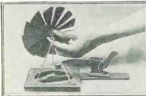
The vane wheel which acts as the heat motor is cut from light tin and is suspended on a wire shaft above the hole in the base through which the heat which operates the motor
