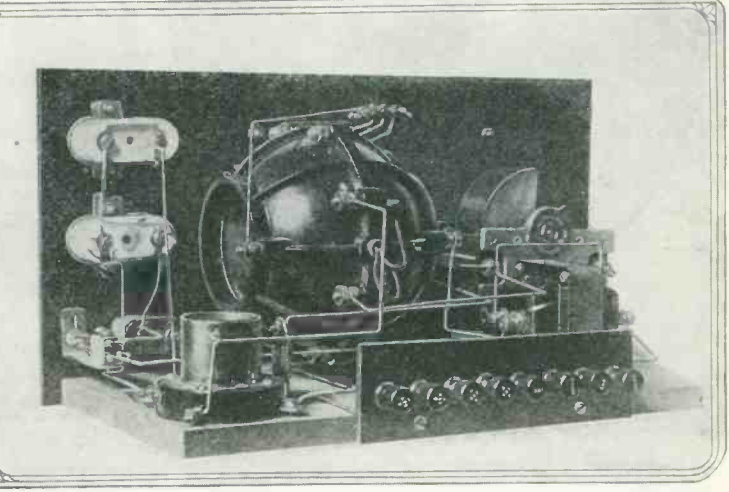
All the binding posts are conveniently racked on a bakelite strip attached to the baseboard. The wiring is direct as much as possible and is of heavy bus wire. A 4 to 1 ratio transformer is used in the capacity of an R.F. choke and affords greater amplification.
