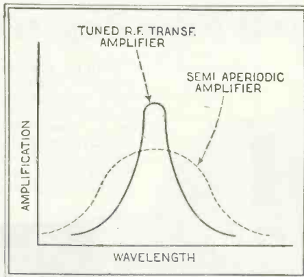
(Q. 311) A graphic representation of the characteristics of both tuned and untuned R.F. transformers is shown herewith. The fact is clearly brought out that higher amplification over a narrower band of wave-lengths can be obtained with tuned R. F.
