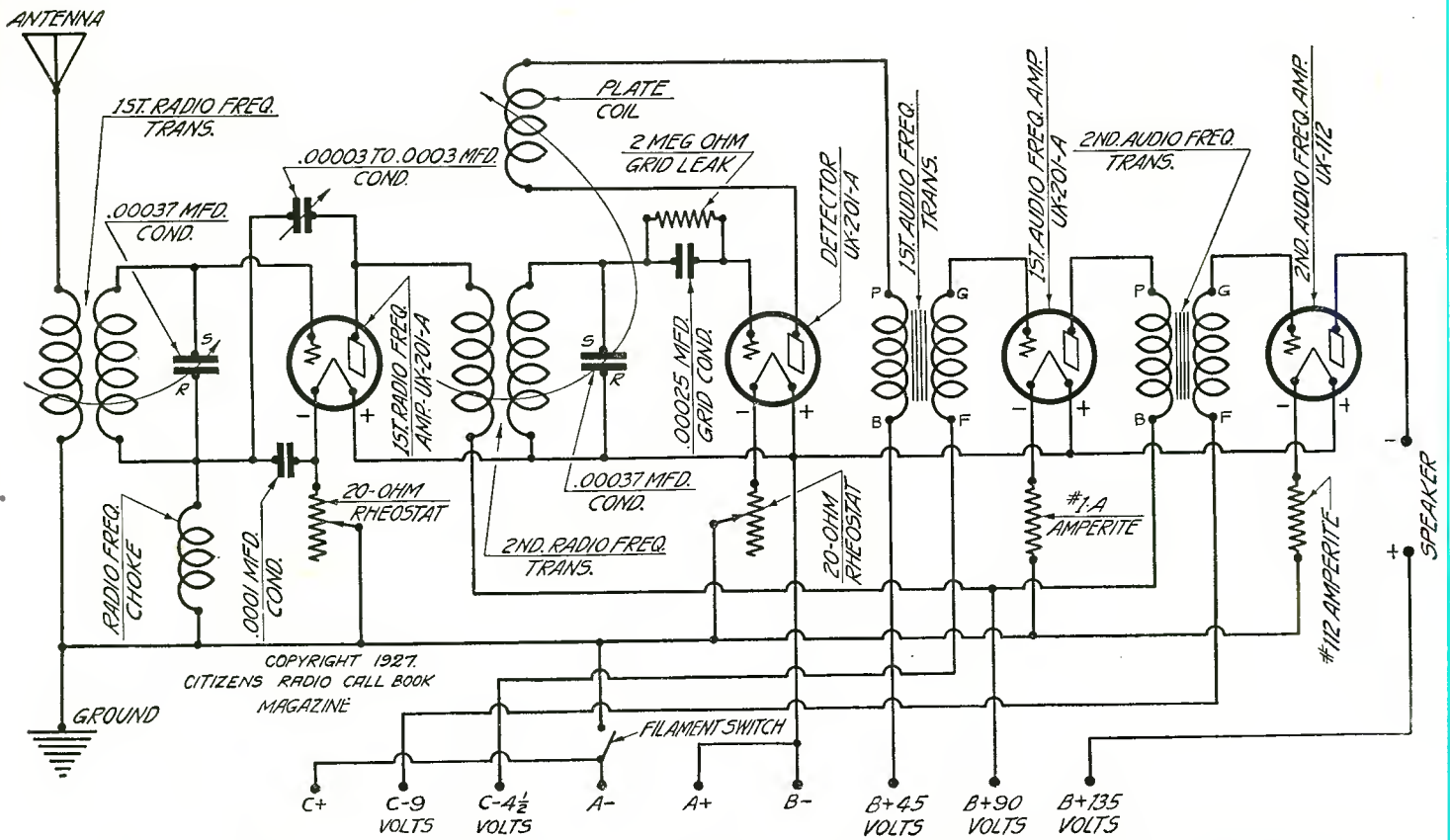
Figure 5. Professional set builders and others who are thoroughly acquainted with construction work may wire the receiver from the schematic above
