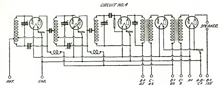
Figure 9. Above is shown a non-regenerative tuned r. f. receiver, which may be changed from a five to a six tube set by the use of different audio units
