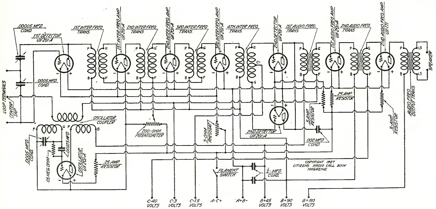
Figure 5. This type of diagram tells the electrical story of what will happen in a receiver. Familiarity with radio is required for reading a schematic circuit, whereas no such experience is required for following connections shown in Figure 7
