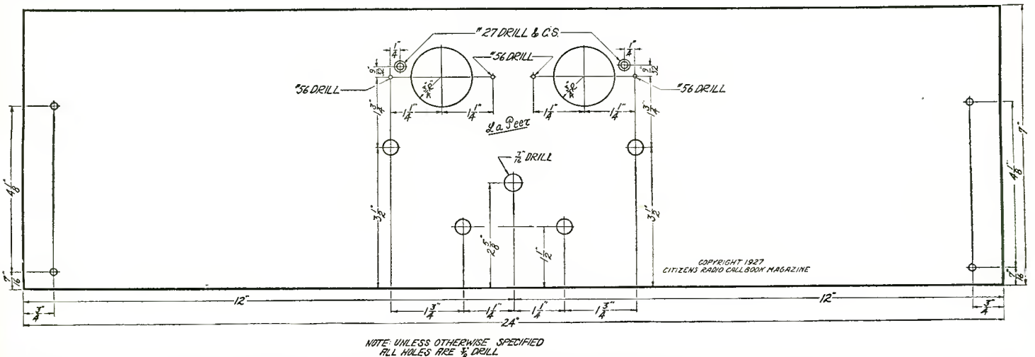
Figure 4. On account of the amount of drilling necessary for using the Remler drum dials, it is recommended that builders secure panels already drilled and engraved, which will greatly simplify their work
