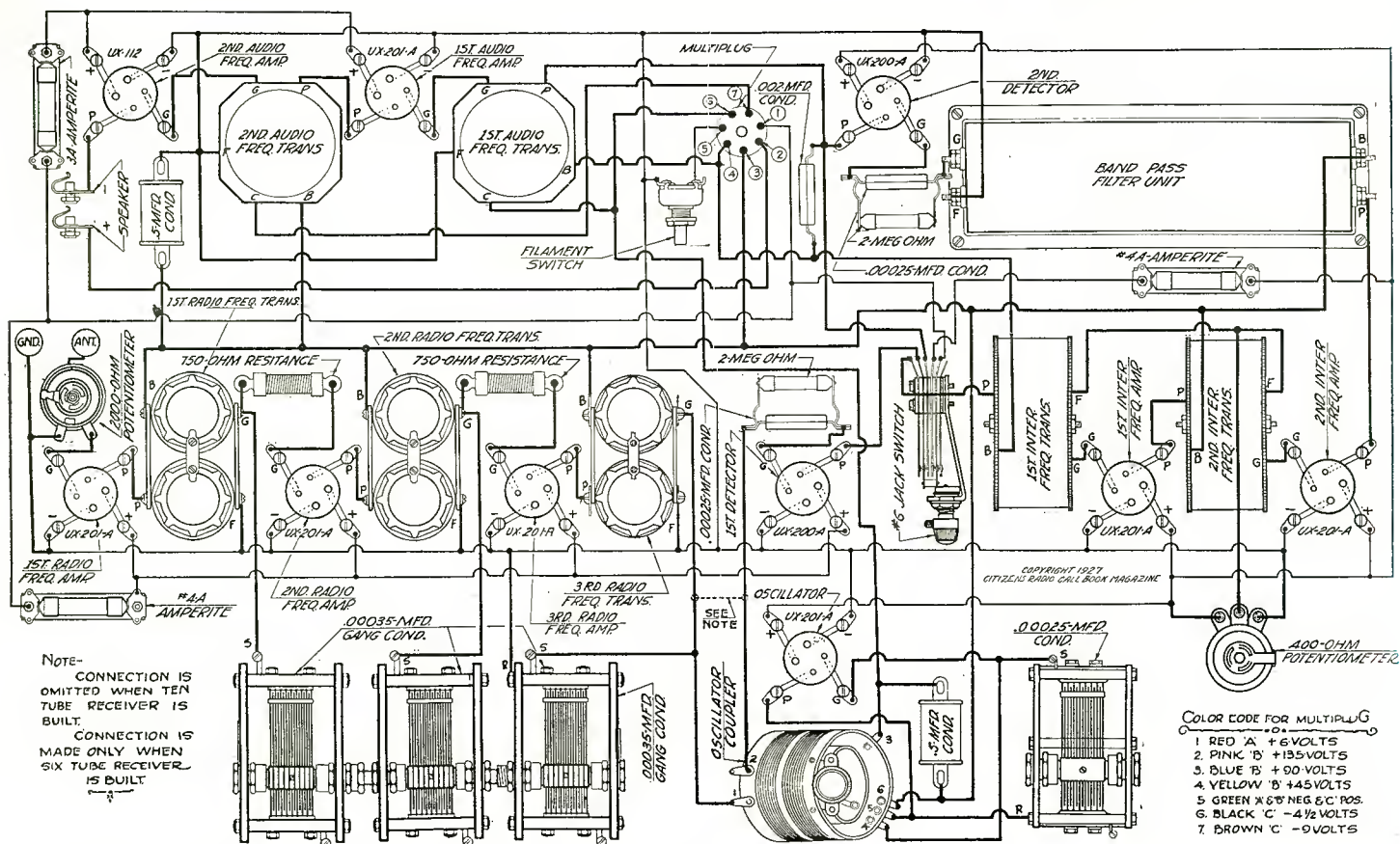
Fig. 7. Depicted above are the proper electrical connections to make for wiring of this powerful receiver. Always check your work against the diagram to make certain no errors have been made
