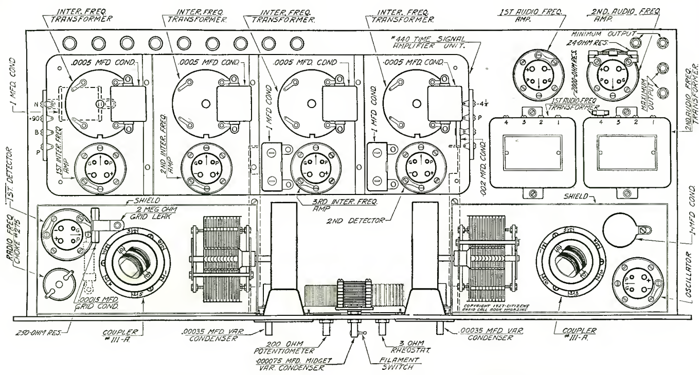
Fig. 4. Baseboard layout of the super described in the accompanying article is shown in the sketch above. Wiring should be done by reference to the schematic diagram, Fig. 3
