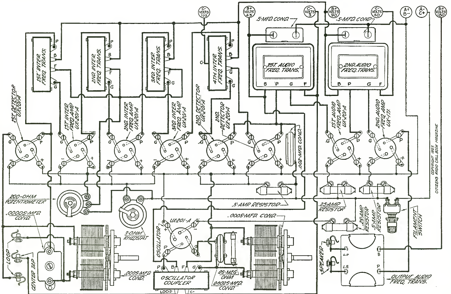
Figure 7. Graphic illustration shown above gives all necessary details for completely wiring this receiver. Be sure to check your work against this for any possible errors on your part
