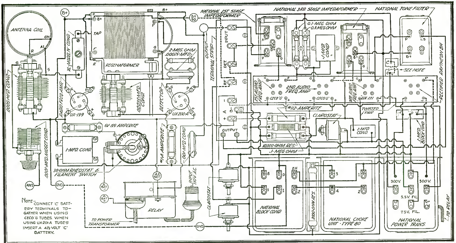
Figure 4. The graphic illustration shown above is a condensed one and represents the correct connections to be made for both the receiver and the power amplifier
