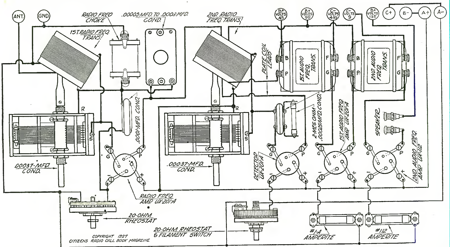
Figure 7. This graphic illustration should be followed by the newcomers in radio and all connections should be made in strict accordance with this diagram
