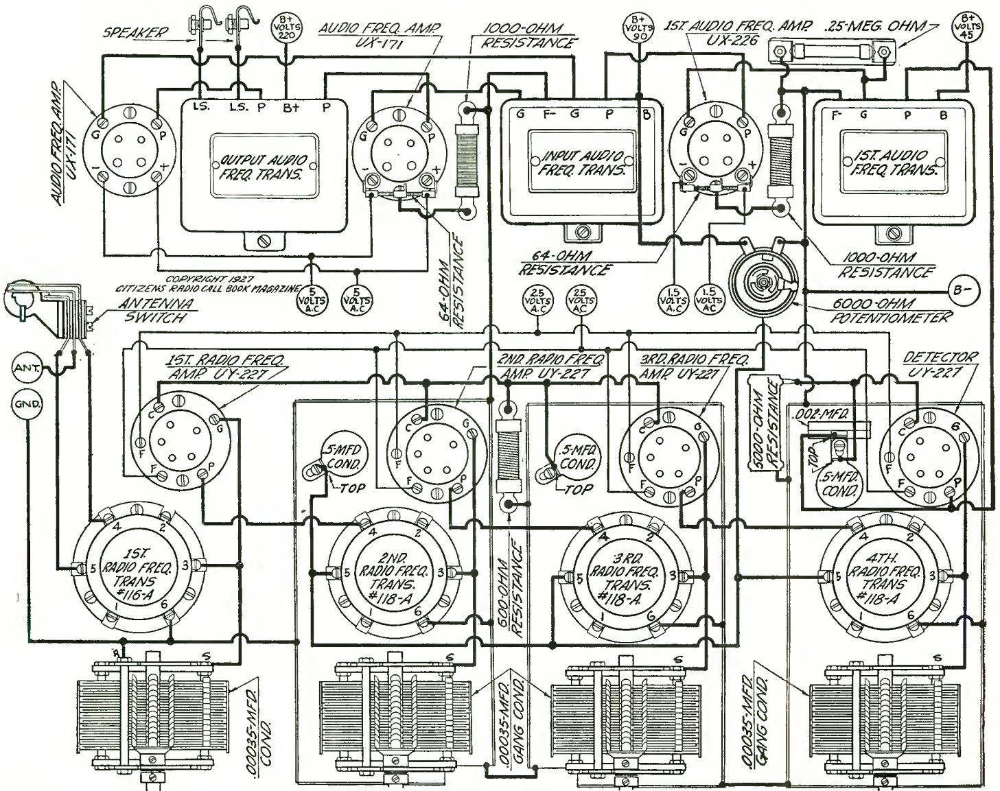
Figure 5. Readers who are not confident enough to wire by a schematic diagram should make use of the graphic illustration prepared for this efficient receiver
