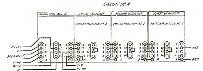
Figure 10. Audio unit No. 2 together with a first, second and third Vari-unit will give a five tube combination, while a six tube may be secured by using an audio unit No. 3 instead of No. 2
