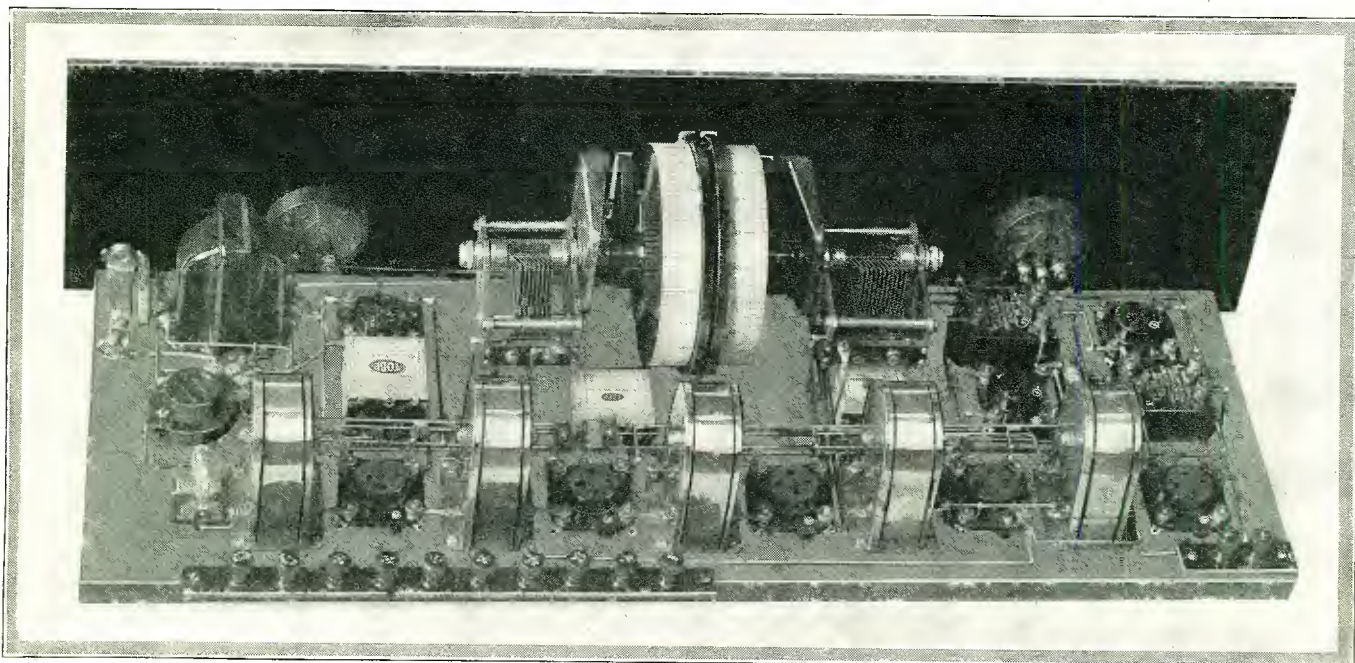
Fig. 2. Rear view of the Madison-Moore International One Spot Receiver is shown in the accompanying photograph
