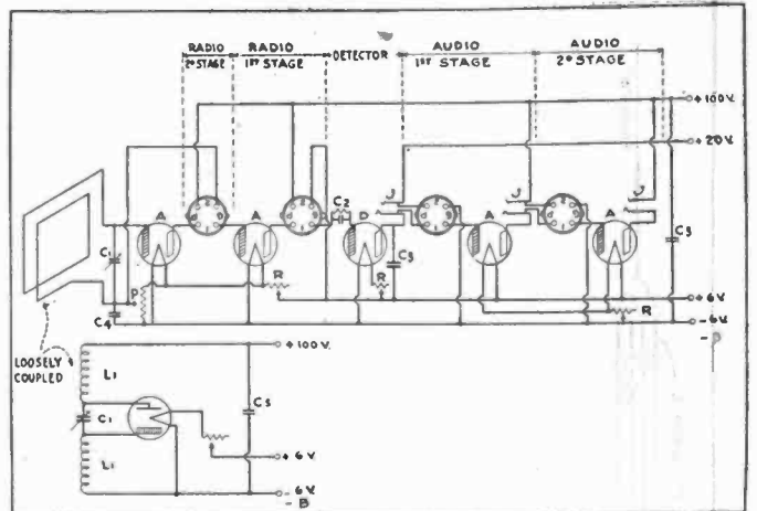
Super heterodyne with radio and audio frequency amplifier.
