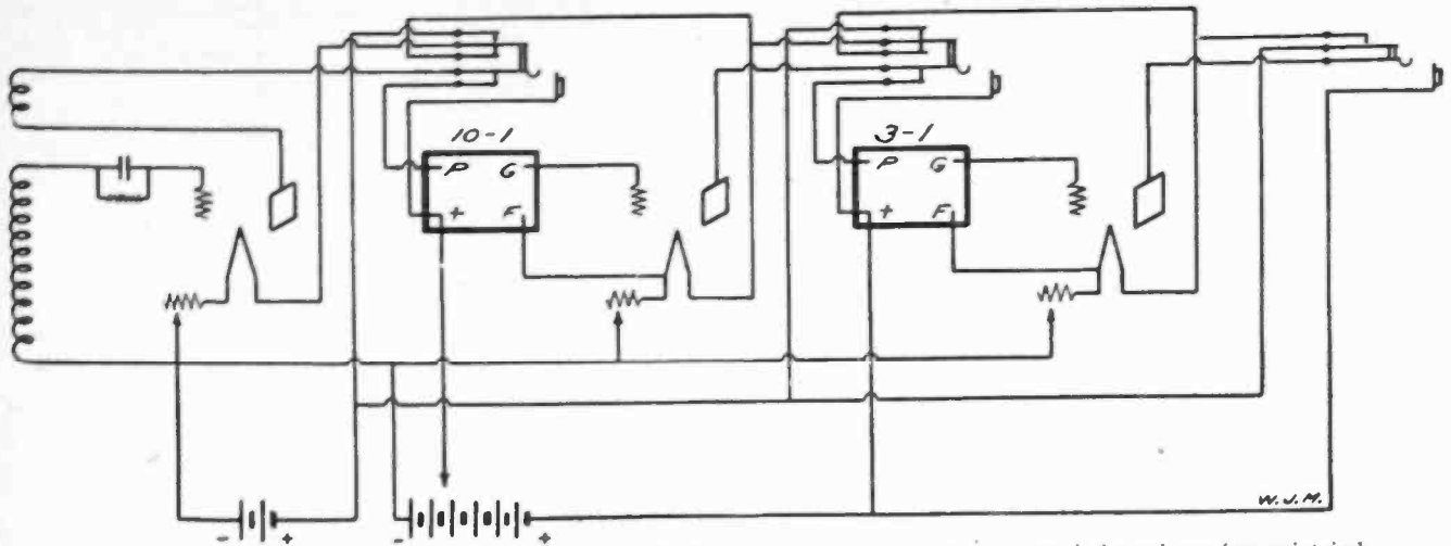
Parts consist of: The usual receiving apparatus, two audio frequency transformers, two six point jacks and one four point jack.
