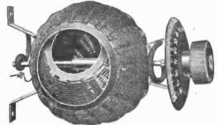
Basketball Variometer 2606 New Price $4.50. The most efficient Variometer on the market. Shaft 3/16 in. diameter. (Fasten small piece of sleeving over end for knob with larger hole.)
