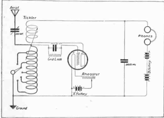
Single Circuit Regenerator.
