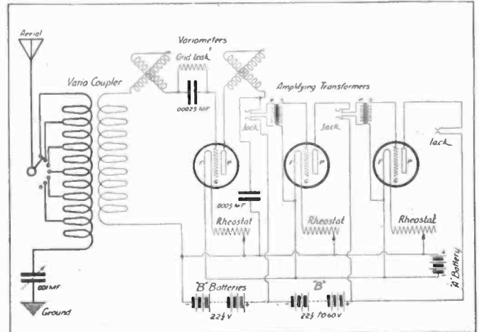
Regenerative Receiver with Two Step Amplifier.
