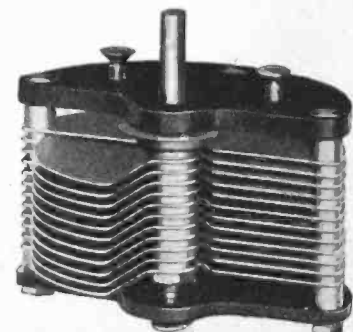
“UNITED” VARIABLE CONDENSERS Without Vernier Dial Assembly
