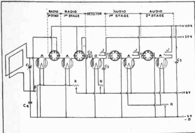
Loop receiver with two stages radio, detector and two stages audio frequency amplification.
