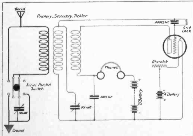
Honeycomb Coil Receiver.
