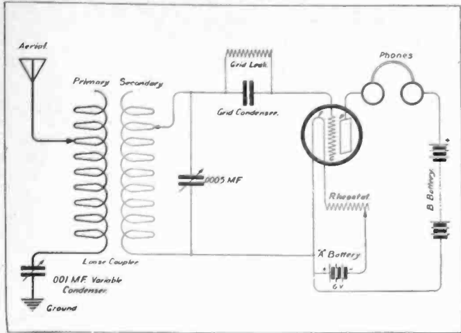
Plain Audion Circuit.
