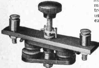
Vernier Variometer 2610 Easily mounted to any panel. Dimensions 3x1 1/2 x 1 1/2 in. Leads provided for quick connection. Price $2.50
