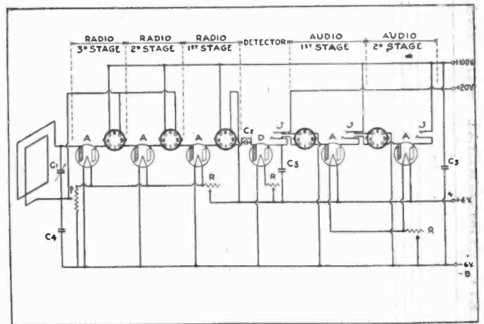
Loop receiver with three stages and two audio frequency amplification.
