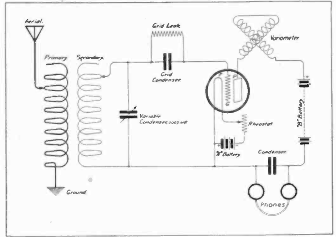
Loose Coupler with Feed Back.
