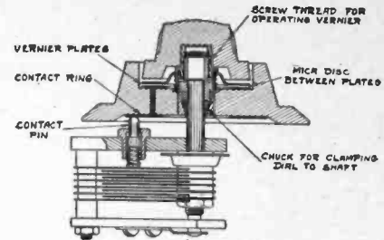
“UNITED” Vernier Dial Assembly
