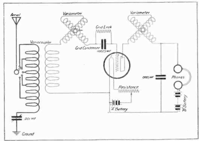
Standard Regenerative Receiver.
