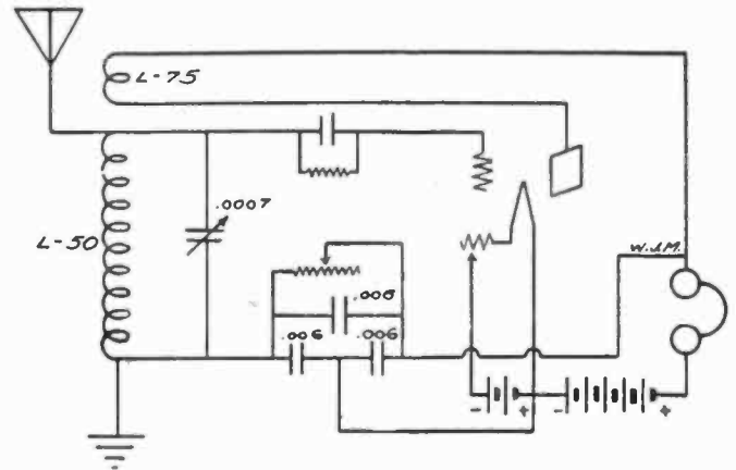
Parts consist of: Two honeycomb coils, one variable condenser, four fixed condensers, one fixed and one variable grid leak, tube and socket, one rheostat, head telephones, "A" and "B" batteries.
