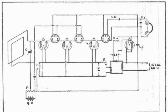
Loop Receiver using 60 cycle AC to operate filaments and plate voltages.
