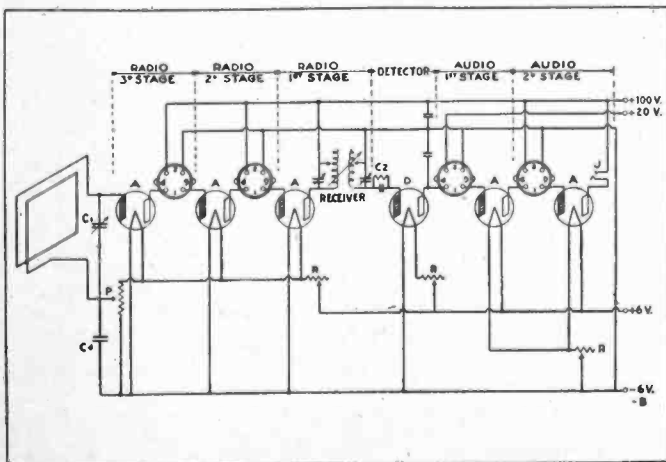
Loop receiver with variable radio frequency transformer.
