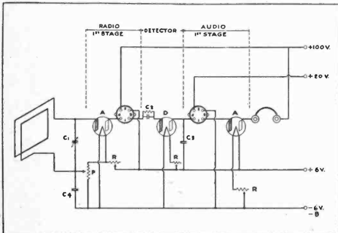
Loop receiver with one stage radio and one stage audio frequency amplification.
