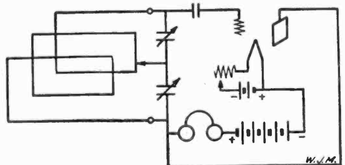
Parts consist of: Loop, two variable condensers, one fixed condenser, tube and socket, one rheostat, head telephones, "A" and "B" batteries.
