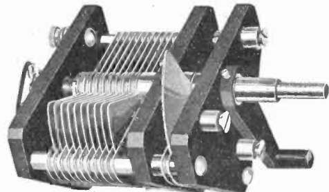
Waltham Variable Condenser Plain or Vernier "Built Like a Watch"
