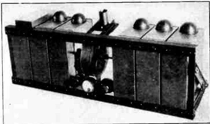
The interior of the new "800." The copper shielding for radio frequency stages and detector tube, and the steel compartment for audio frequency stages, all supported on a heavy angle-iron chassis, make this receiver a veritable electric cage.
