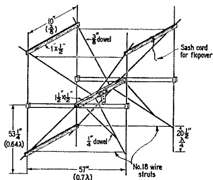
Fig. 1—Detail drawing of the lightweight flopover array described by W2WFB.
