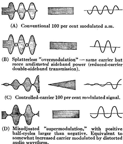
Fig. 1 — Amplitude-modulation waveforms.
