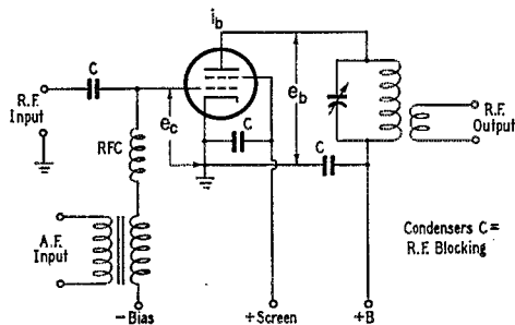
Fig. 2 — Basic circuit, ordinary grid-bias modulated amplifier.
