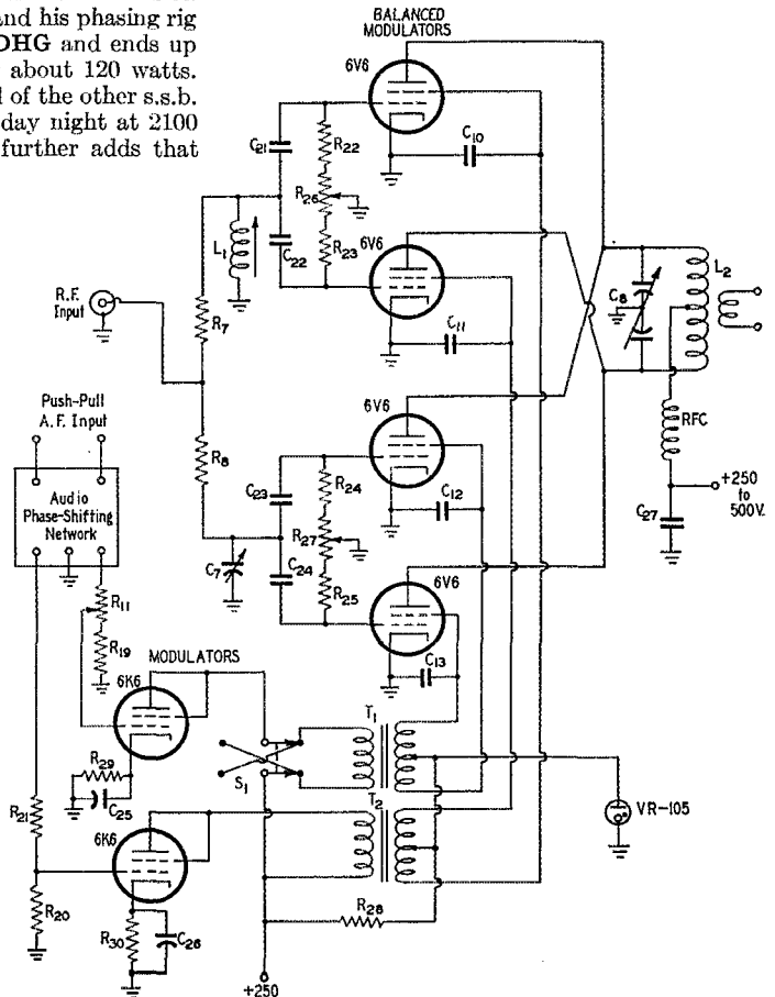
Fig. 1 — The revised W2UNJ s.s.b. circuit. All parts are the same as in the circuit shown in the August, 1949, QST or the 1950 ARRL Handbook , except as noted below.
