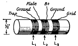
Fig. 5—Details of windings for the circuit of Fig. 4. Coils are spaced \frac{1}{8} inch.
