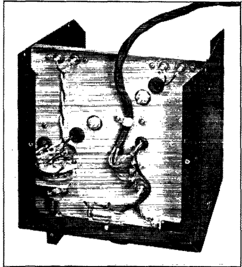
A bottom view of the converter. S_1 , the antenna-transfer switch, is at the lower left. Low-impedance antenna leads should be twisted loosely as shown. The three adjusting screws for the iron-core inductances protrude from the chassis on either side of the power cord.
