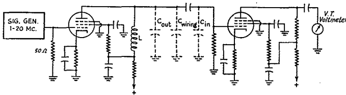
Fig. 7 — Test arrangement for determining inherent circuit capacity. Values such as cathode resistor, screen resistor, etc., are not critical; those suitable for resistance-coupled operation are in order. The total circuit capacitance, C_t is the sum of C_{out} , C_{in} and C_{wiring} . L is some known value of inductance; 50 \mu h. is a good choice. Resonance with C_t should occur at a frequency, F , near
