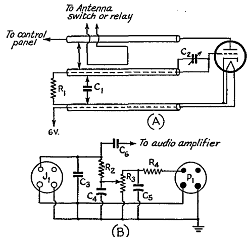
Fig. 2 — A shows the schematic diagram of the receiver proper. B is the superregenerative receiver control panel.
