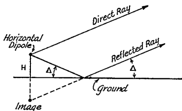
Fig. 3 — Reflection from ground.
