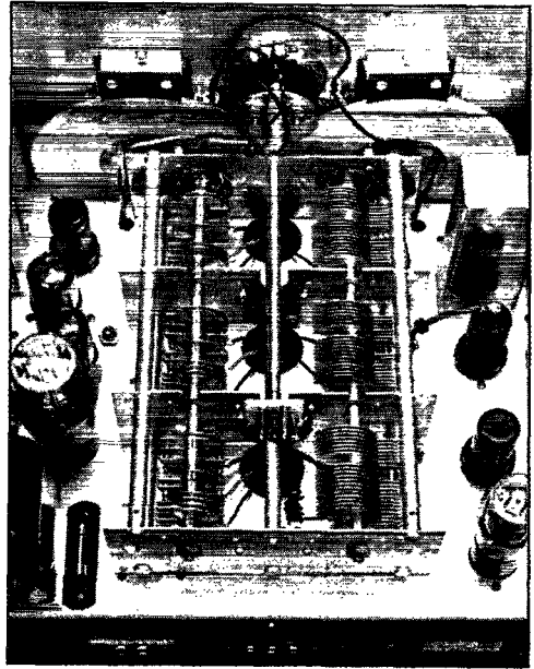
A top view of the HQ-129-X with the dust cover removed from the tuning-condenser assembly to show the main-tuning gang (right) and the bandspread condensers. The antenna trimmer condenser is in the center.
