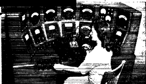
Extreme accuracy and flexibility of this Hytron master test station particularly fit it for quality control.
