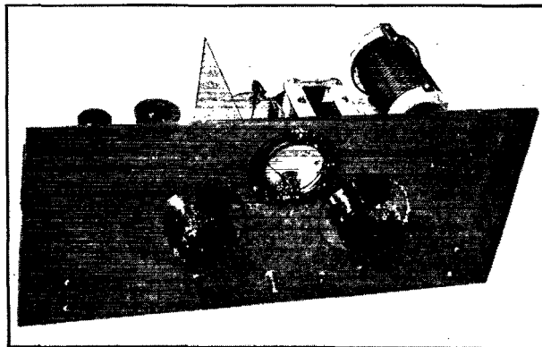
A two-tube medium-power transmitter. The panel is 8\frac{3}{4} inches high and the chassis measures 7 \times 17 \times 3 inches.
