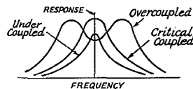
Fig. 3 — Response curves for various degrees of coupling.
