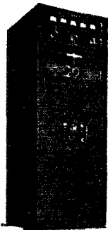
Collins 16F-9 —Nominal power output: 300 watts phone; 500 watts c.w. Frequency range: 2 to 18 Mc. Ten quick-shift frequencies.
