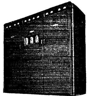
Collins 1000-C —Nominal power output: 2500 watts. Frequency range: 2 to 20 Mc. Additional a.f.-modulator & r.f. multi-channel sections available.
