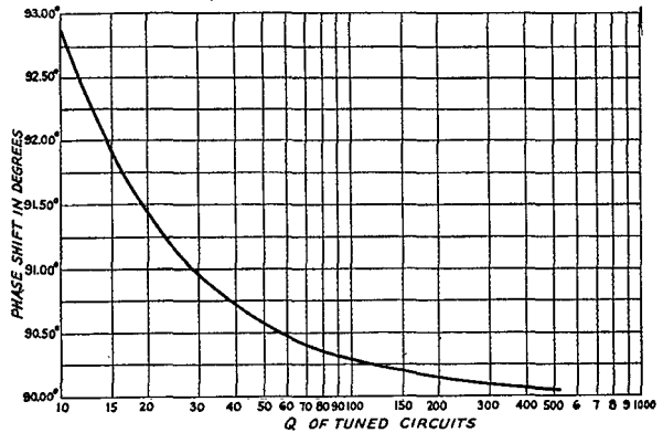
Fig. 8 — Graph of double-tuned-circuit phase shift at resonance vs. the Q of the tuned circuits from Eq. (19).
