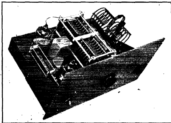
A push-pull amplifier using high-power beam tetrodes. The panel is 10½ inches high while the chassis is 13 inches deep, 3 inches high and 17 inches long for standard rack mounting.
