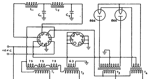
Fig. 4 — Circuit diagram of the a.c. supply for the modulator and last two transmitter stages of the WERS control transmitter.
