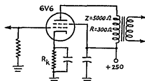
Fig. 2—Typical output-stage circuit with transformer coupling.
