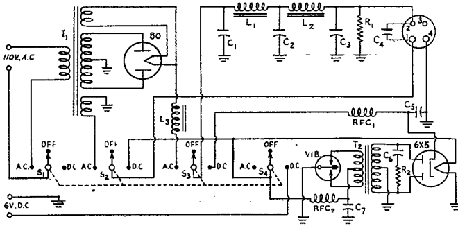
Fig. 3 — Circuit diagram of the combination a.c. and vibrator power supply for receiver, speech-amplifier and exciter stages.
