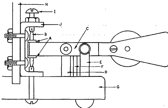
Fig. 2—Side view of electronic key movement, illustrating bearings and supports of moving parts. (A) Ears on lever A (see photograph) (B) Pivot spindle. (C) Keying lever. (D) Dot spring post. (E) Dash contact post. (F) Dot stop. (G) Key base. (H) Control panel. (I) Pivot screw. (J) Pivot support.
