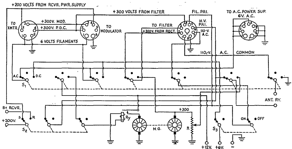
Fig. 5 — Circuit diagram of the control and junction panel used with the WERS control transmitter.
