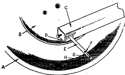
Fig. 1 — Device for driving a cutter head for home recordings. (A) Master pregrooved 12-inch blank. (B) Recording disc, 6½-inch diameter. (C) Cutter head and arm. (D) Cutting needle. (E) Drive bar. (F) Set screw. (G) Binding-post chuck. (H) Tracking needle.
