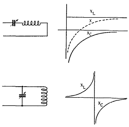
Fig. 2 — Methods of inserting reactance at the base, or tuning the antenna, with curves showing corresponding reactance variation.
