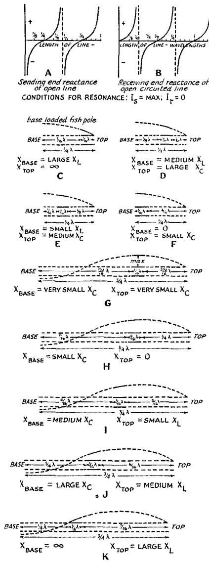
Fig. 1 — Showing how the current in a short antenna can be changed by insertion of various reactance values at the top, along with proper values at the base for tuning. Quantities are as follows: X_{\text{base}} reactance which must be placed in series with antenna at its base ( X_s of auxiliary line at the base). X_{\text{top}} reactance which must appear between top of antenna and ground ( X_r of auxiliary line at the top). X_r receiving-end reactance of line (reactance looking into the line toward the source of energy). X_s sending-end reactance of line (reactance looking into the line away from the source of energy). Reactance values are expressed relative to the surge impedance of the antenna, which for ordinary wire sizes may be taken as approximately 400 ohms. 1
