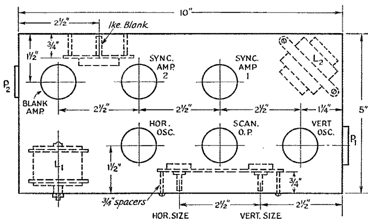
Chassis depth = 3" Socket holes 1 1/8" diam.
