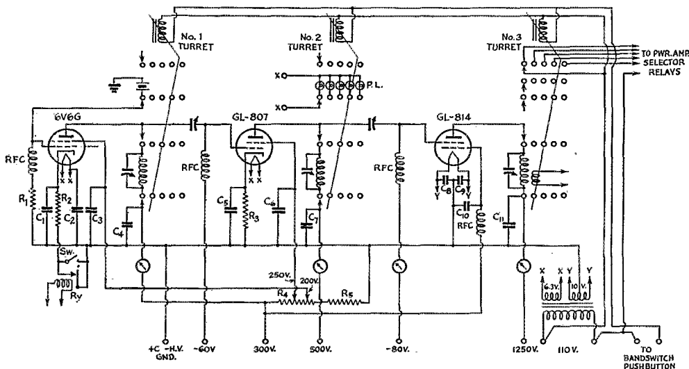
Fig. 1 — Circuit of the exciter with magnetic bandswitching. For simplicity, only one band is shown; circuits for the other four bands connect to the appropriate switch points.
