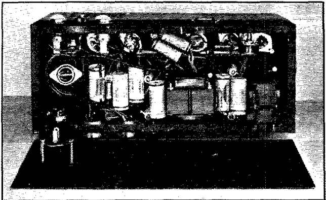
Transformers T_4 and T_1 (right) are mounted underneath the power supply chassis. Note that filter condensers connected in series are supported on stand-off insulators.
