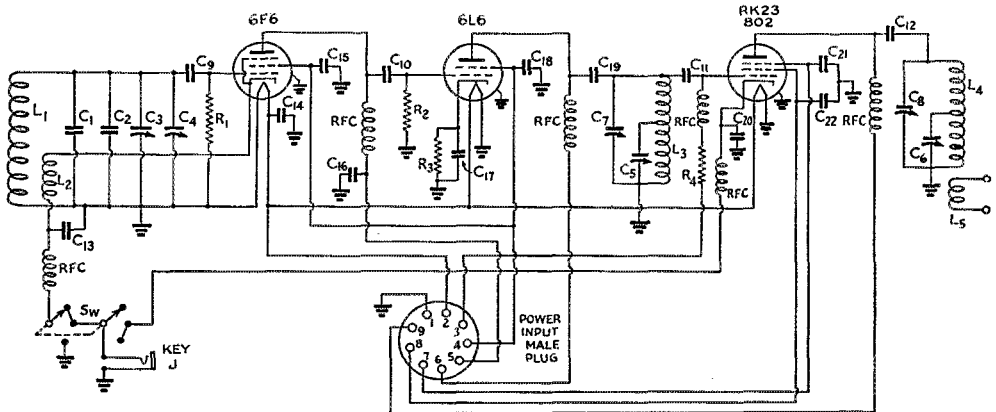
Fig. 1 — Circuit diagram of the e.c.o. exciter.
