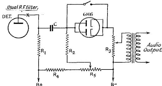
Fig. 1 — Circuit of series noise limiter as used with plate detector. R_1 — 0.1 meg. R_4 — 50,000 ohms. R_2 — 0.3 meg. R_5 — 50,000 ohms. R_3 — 50,000 ohms. C — 0.1 \mu f.
