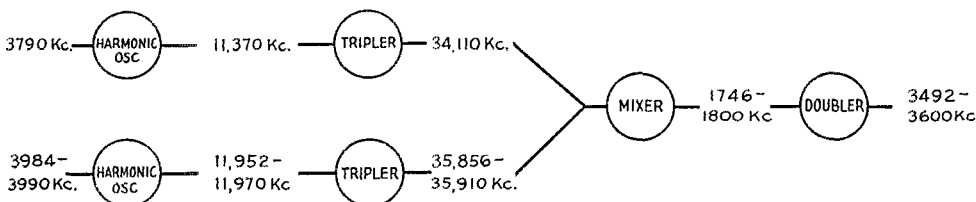
Fig. 1 — A block diagram illustrating the principle of extended frequency variation. The crystal frequencies shown are not the only ones that can be used — they were selected only as examples.
