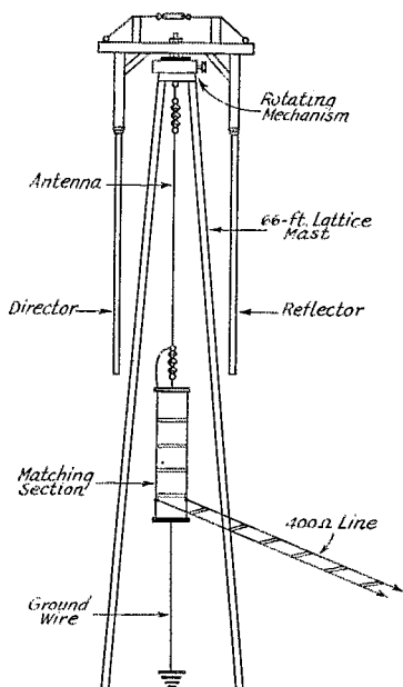
Fig. 2 — Simple 3-element rotatable antenna suggested by W4ANN. Approximate dimensions for a frequency for 14.2 Mc. are: Antenna — 32.9 ft. (0.475λ); reflector — 34.6 ft. (0.5λ); director — 32 ft. (0.46λ); matching section — 32.9 ft. (0.24λ); ground wire — 32.9 ft. (0.24λ); director spacing — 6.9 ft. (0.1λ); reflector spacing — 6.55 ft. (0.095λ).
