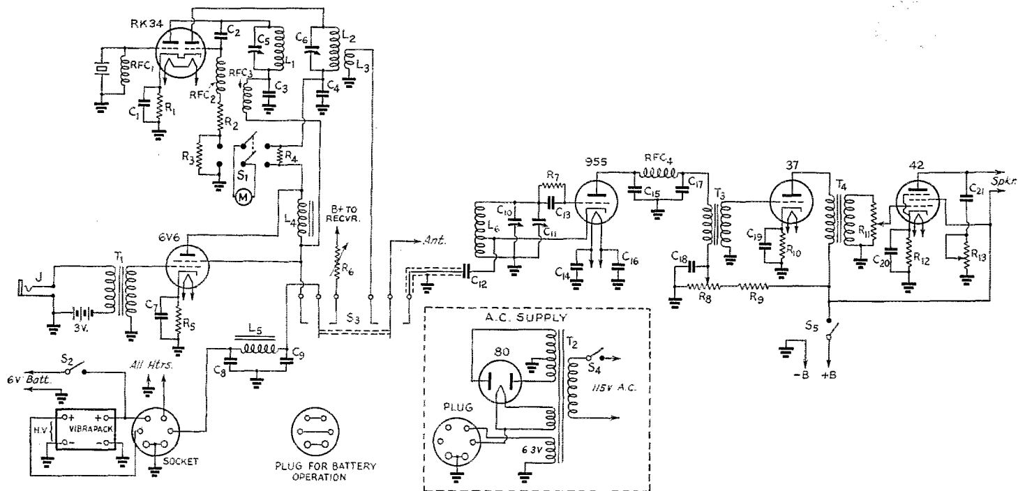
Fig. 1 — Complete circuit diagram of the 56-Mc. mobile station.
