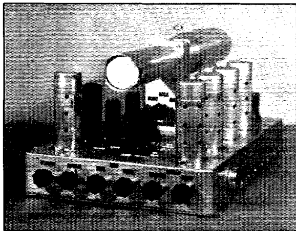
◆ The controls are readily accessible to the operator viewing the image on the monitor from this end of the chassis. The location plan of the tubes and controls is shown in Fig. 6. ◆
