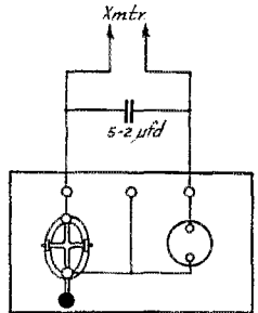
FIG. 4—USING THE CODE PRACTICE BUZZER IN A KEY-THUMP ELIMINATOR
