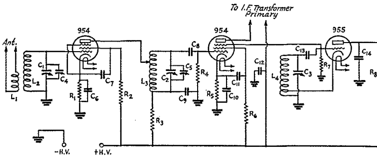
This unit is actually a conventional super-heterodyne tuning system with pre-selector, first detector and first oscillator. Suppressor injection is used in the first detector. Constants and adjustment details will be given in Part II of this article.
