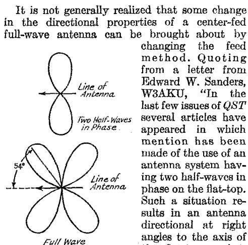
FIG. 1—HORIZONTAL-PLANE DIRECTIONAL CHARACTERISTICS OF TWO-HALF-WAVES IN PHASE (UPPER) AND FULL-WAVE (LOWER) ANTENNAS
