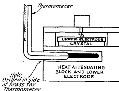
FIG. 2—THE ADDITION OF THE THERMOMETER FOR TEMPERATURE CHECKING
