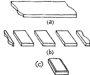
FIG. 5—EVOLUTION OF THE ROUGH BLANK FROM A SLICE CUT FROM THE CRYSTAL SECTION OF FIG. 3
