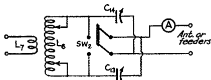
FIG. 2—WIRING OF THE ANTENNA TUNER C_{13}, C_{14} —300- \mu fd. variables (National Type TMS-300). Sw_2 —D.p.s.t. knife switch. A —Antenna ammeter, 0–2.5 amp. L_6 —24 turns No. 12 enamelled wire, turns spaced to occupy a winding length of 3 1/2 inches, coil diameter 2 inches, tapped as described in text. L_7 —2 turns No. 12 enamelled wire, diameter 2 1/2 inches. With Sw_2 open, tuning condensers are in series with L_6 , with Sw_2 closed, in parallel.
