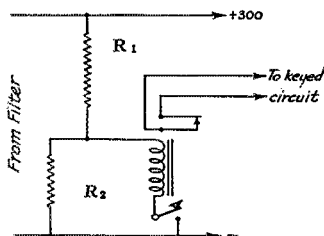
FIG. 6—POWER SUPPLY FOR THE KEYING RELAY FROM THE LOW-VOLTAGE POWER PACK
