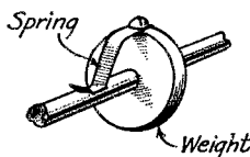
FIG. 7—A SPRING CLIP ON THE BUG WEIGHT MAKES RAPID ADJUSTMENT EASY
