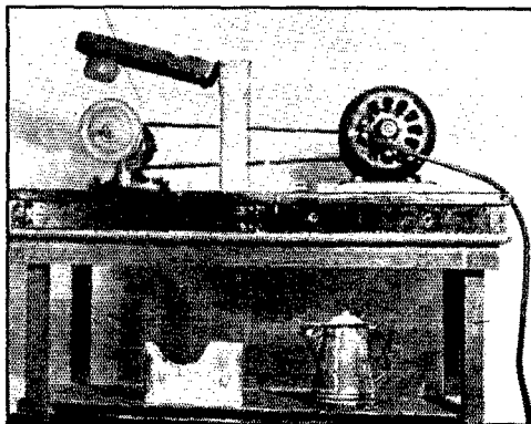
CRYSTAL CUTTING RIG BUILT BY THE AUTHOR AND WSIGF
