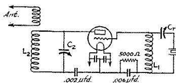
FIG. 2—THE "R" CIRCUIT
