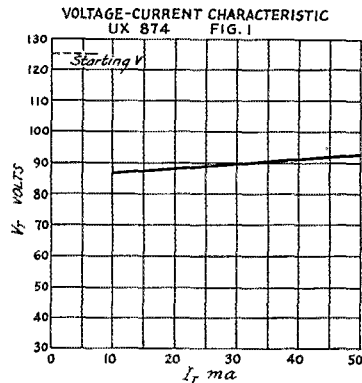
FIGS. 1 AND 3—VOLTAGE-CURRENT CHARACTERISTICS OF GASEOUS REGULATOR TUBES
