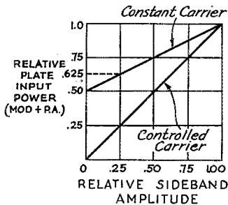
FIG. 4—POWER CONSIDERATIONS COMPARED FOR CONSTANT-CARRIER AND CONTROLLED-CARRIER SYSTEMS
