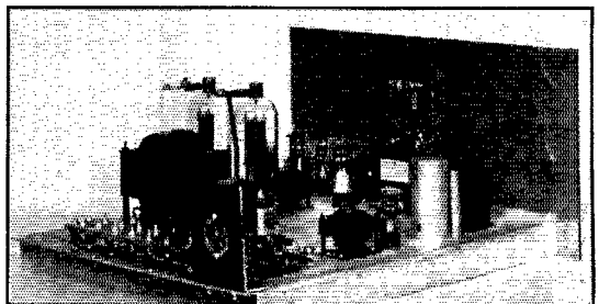
CLASS-B MODULATOR OF THE TYPE USED FOR CONTROLLED-CARRIER 'PHONE OPERATION AT W2DC
