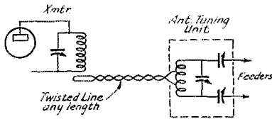
FIG. 5—LINK COUPLING BETWEEN THE TRANSMITTER AND ANTENNA TUNING APPARATUS
