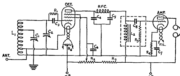
FIG. 1—CIRCUIT DIAGRAM OF THE TWO-TUBE RECEIVER
