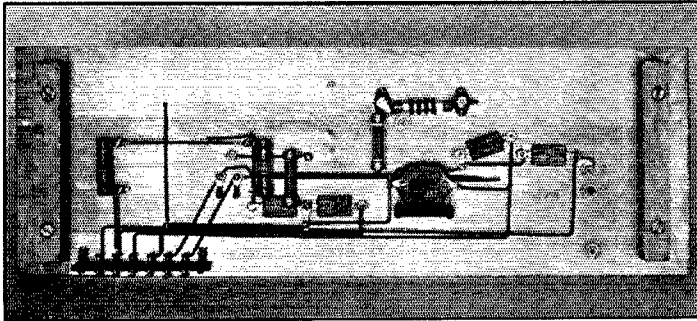
A SUB-BASE VIEW OF THE EXCITER UNIT Details of the wiring are given in the text.
