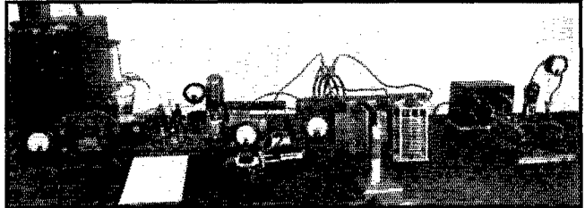
SPECIMENS ARE GIVEN RADIO-FREQUENCY TREATMENT BETWEEN THE PLATES OF THE TANK CAPACITOR ON THE PANEL OF THE 50-WATT OSCILLATOR
