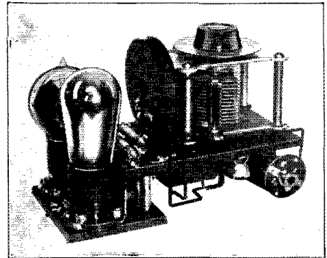
THE OSCILLATOR AND ITS ISOLATING AMPLIFIER
