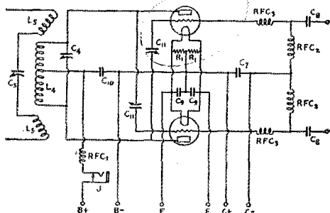
FIG. 7.—THE PUSH-PULL 1½-MC. MODULATED AMPLIFIER CIRCUIT
