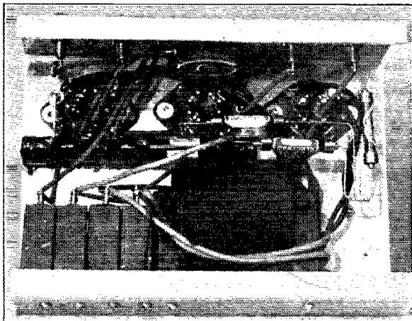
BENEATH THE BASE OF THE AMPLIFIER Transformer, condensers, and resistors are arranged compactly.
