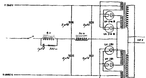
FIG. 2 THE PLATE SUPPLY AT W9BVH
