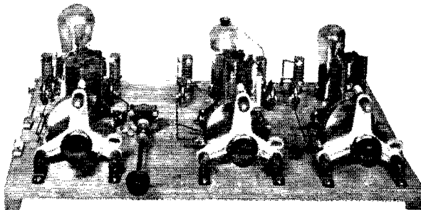
The above is an illustration of a breadboard layout employing one UY-227, one UY-224 and one UX-245 in a modern M.O.P.A. circuit. This transmitter was built by W2BNC, Brooklyn, New York, using REL parts.
