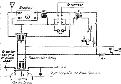
FIG. 1.—KEYING SYSTEM AT WSCEO
