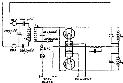
FIG. 3. — A METHOD OF ACCURATELY TUNING TUBES OPERATED IN PARALLEL
