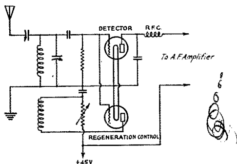
FIG. 2. — AUXILIARY TUBE FOR CONTROLLING REGENERATION
