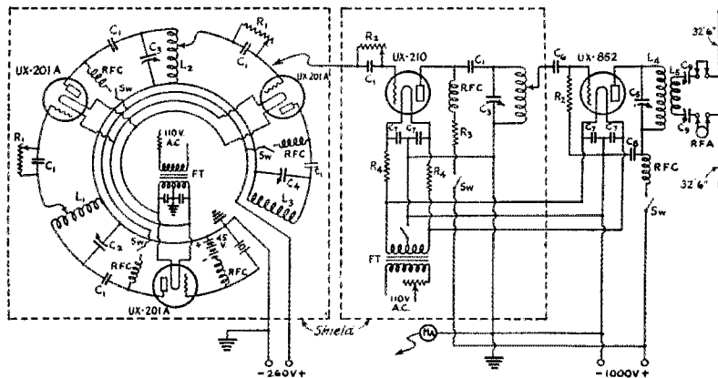
FIG. 1. — THE TRANSMITTING WIRING DIAGRAM OF THE TRANSMITTER AT W0BVH. NOTE THE ROMAN CANDLE EFFECT!
