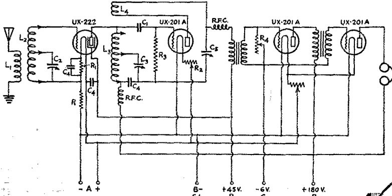
FIG. 3—ANOTHER ARRANGEMENT OF A FOUR-TUBE RECEIVER
