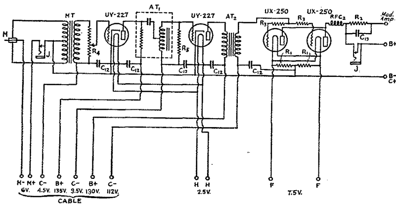
FIG. 5. — THE SPEECH AMPLIFIER AND MODULATOR
