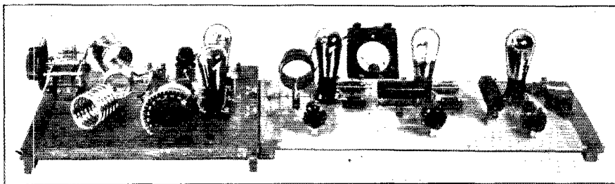
THE RADIO-FREQUENCY PORTION OF THE TRANSMITTER
