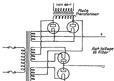
FIG. 3.—SINGLE-PHASE FULL-WAVE SERIES RECTIFIER CIRCUIT
