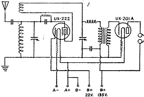
FIG. 4. — SPACE CHARGE DETECTOR
