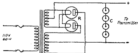
FIG. 2.—POWER SUPPLY FOR VOLTAGES UNDER 1100
