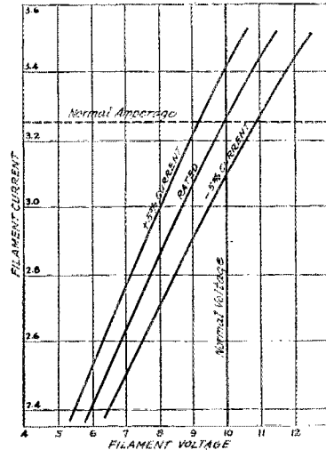
FIGURE 2. FILAMENT CURVES, SHOWING THE IMPORTANCE OF CORRECT FILAMENT VOLTAGE
