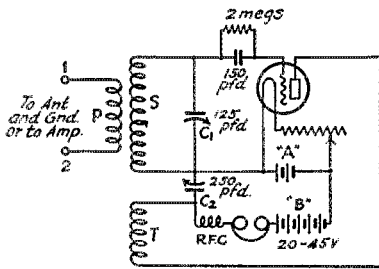
FIG. 1 THE REGULAR SHORT-WAVE RECEIVER
