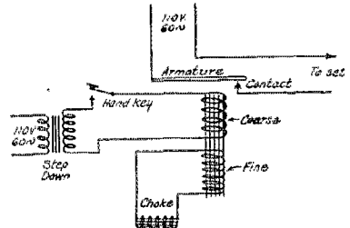
FIG. 3. USING A FORD GENERATOR CUTOUT AS A MAGNETIC KEY
