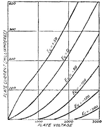
FIGURE 6. STATIC PLATE VOLTAGE-PLATE CURRENT CURVES WITH DIFFERENT GRID VOLTAGES
