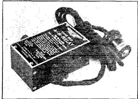
OUTER AND INNER VIEWS OF TYPE 595 JEWELL A-B-RELAY
