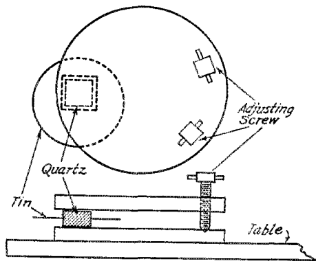
RIG FOR TUNING GRINDING FIG 4
