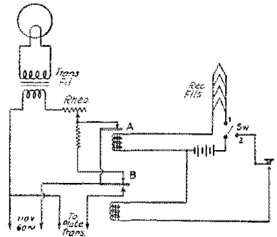
FIG. 5. A CIRCUIT TO KEEP THE A. C. CIRCUITS OFF THE OPERATING TABLE AND TO KEEP THE TRANSMITTING TUBES WARM
