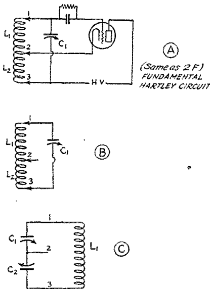
FIG 9A - HARTLEY & COLPITTS
