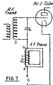
USUAL SERIES METHOD OF CONNECTING R. F. AND A. F. TRANSFORMER SECONDARIES TO A REFLEXED TUBE SHOWING THAT THE ROTOR OF THE TUNING CONDENSER CANNOT BE BROUGHT TO FILAMENT VOLTAGE
