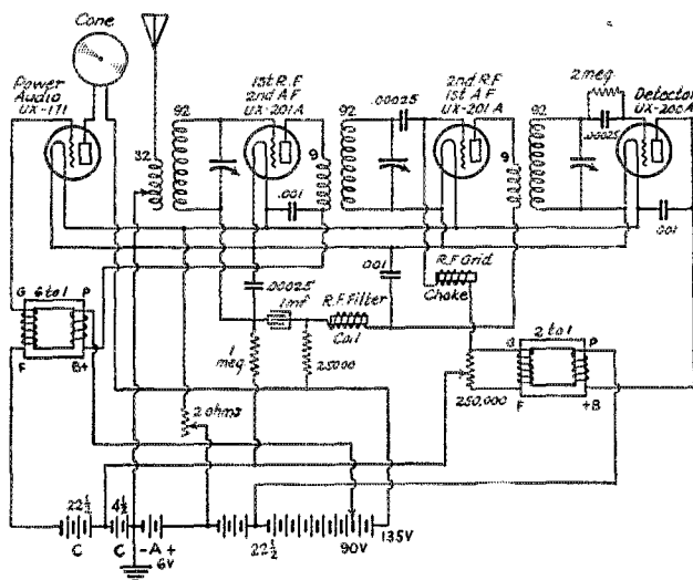
FIG. 3. THE CIRCUIT OF THE I. D. S. RECEIVER WHICH DIFFERS FROM THE NEW R.G.S. ONLY IN THAT THE LATTER USES A 2-GANG CONDENSER AND THEREFORE HAS A SMALL "MAKEUP" VARIABLE CONDENSER CONNECTED ACROSS THE THIRD VARIABLE CONDENSER. SEE FIG. 6 FOR DETAILS
