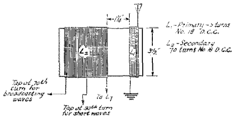
Tuner details, see Fig. 6 for connections of complete set. FIG. 4B
