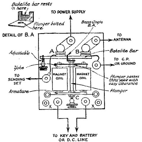
FIG. 1 THE LEACH BREAKIN RELAY
