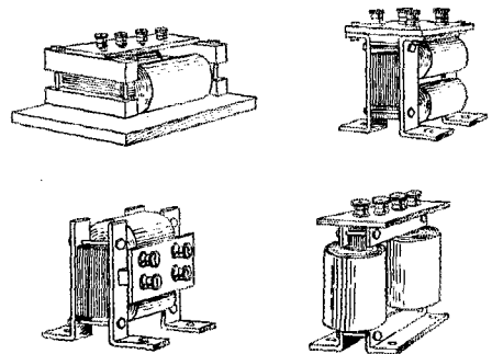
FIG. 8 WAYS OF MOUNTING TRANSFORMERS
