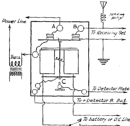
OPERATION—When key is closed, C opens first and disconnects detector B battery, then B short-circuits the tuner and finally A connects transformer to the line FIG. 2 CONNECTIONS OF LEACH BREAKIN FOR SPARK WORK.
