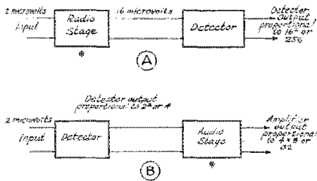
* These stages assumed to have voltage amplification of 8 per stage, counting tube and transformer. FIG. 1 WHY RADIO INSTEAD OF AUDIO
