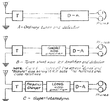
FIG. 2 THE SUPERHETERODYNE IDEA In all three diagrams T is a good tuner, D-A is a detector and audio amplifier.
