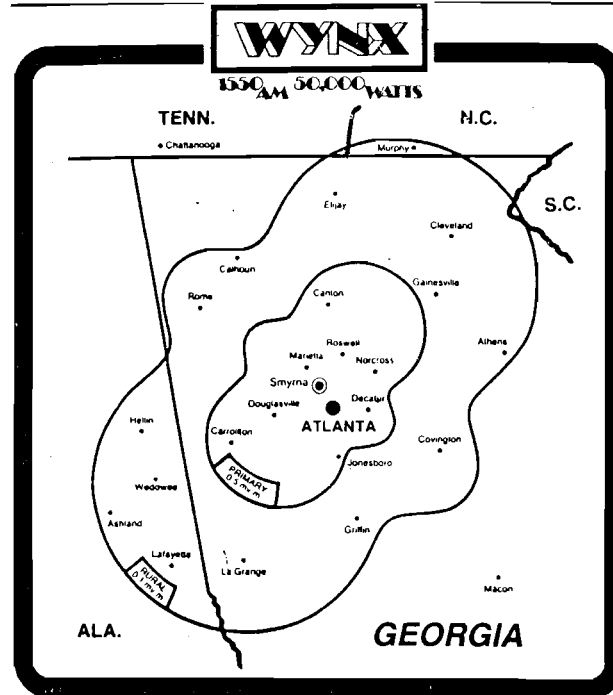
WYNX DAYTIME PATTERN - courtesy of General Manager Alan Karr
