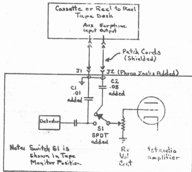
Modified Receiver Wiring
