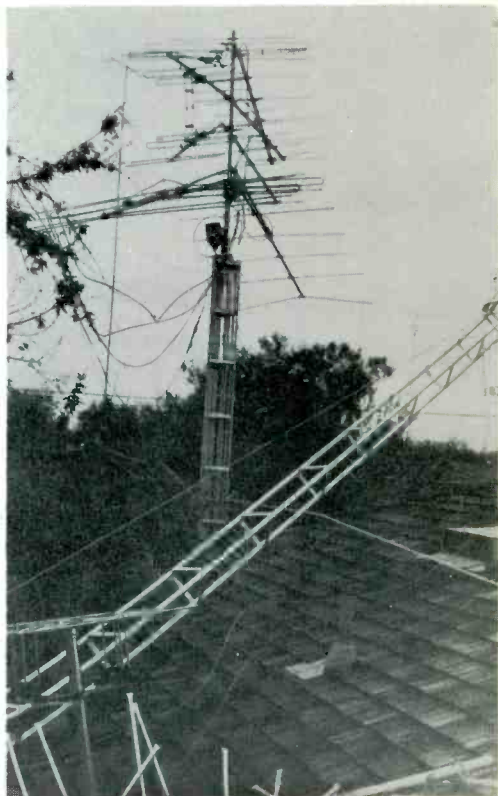
SMASHED YAGIS and cracked steel tower (in the background) were constant reminders of the dangers in 100 foot and up crank-up towers. Our advise—"when using crank-ups, stick to the 80 foot and down variety!"
