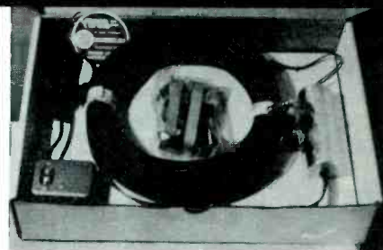
Shown—"Over the counter" Retailing Kit, includes attractive box with instructions, MBT/213 Transistor Amplifier, mounting hardware, remote power supply, stand-off insulators, 75 feet 300 ohm down-lead.
