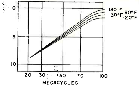
5b. TYPICAL THERMATIC SLOPE EQUALIZER RESPONSE
