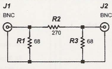
Fig. 5. 20 dB attenuator. R1 and R3 are 68 ohm 10 W carbon composition or non-inductive resistors. R2 is a 270 ohm 2 W carbon composition or noninductive resistor.
