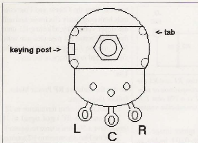
Fig. 2. Potentiometer designations.
