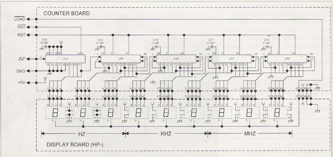
Fig. 5. Counter and display boards.
