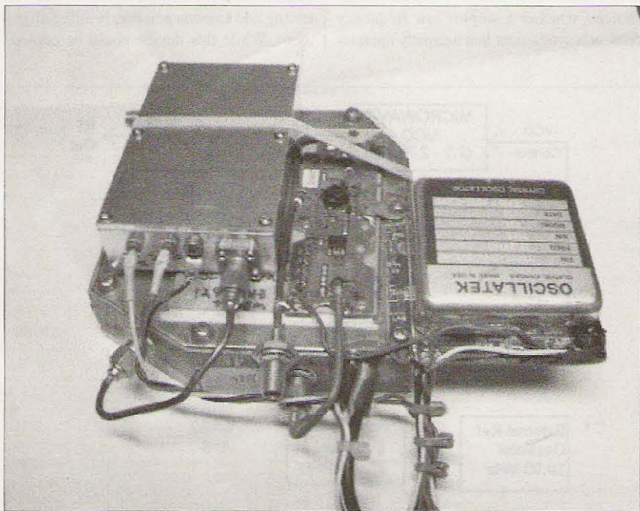
Photo B. Completed Texas Synthesizer mounted in heat sink metal compartment with 4x harmonic multiplier on top with another amplifier board for gain at divide-by-2 output. This unit can provide 1/2 LO output or 1,296 MHz, plus 2,592 MHz, multiply by 4 = 10,368 MHz. For band, very accurate band edge markers.
