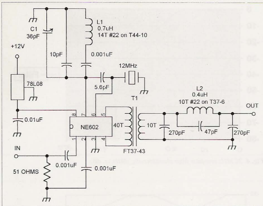
Fig. 2. Schematic of the range extender circuit.
