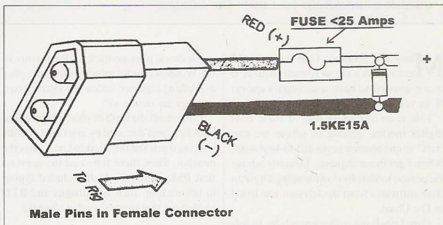
Fig. 3. The wiring pigtail from the transceiver.
