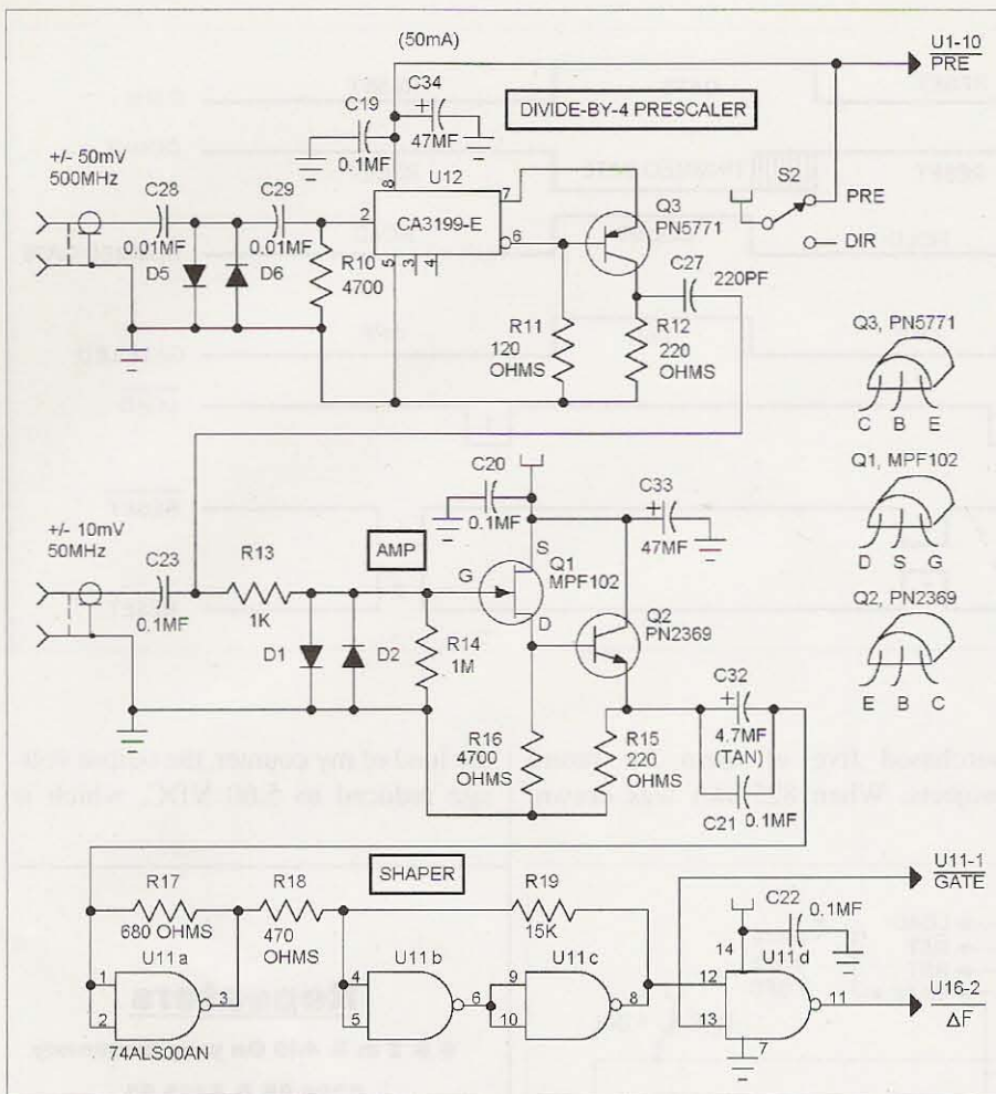
Fig. 3. Signal-conditioning schematic. References: HR, Feb. '78, pg. 28; 73, Dec. '78, pg. 107; Fairchild app. note 95H90. Note: In this article, the use of MF in schematics is meant to indicate \mu\text{F} .
