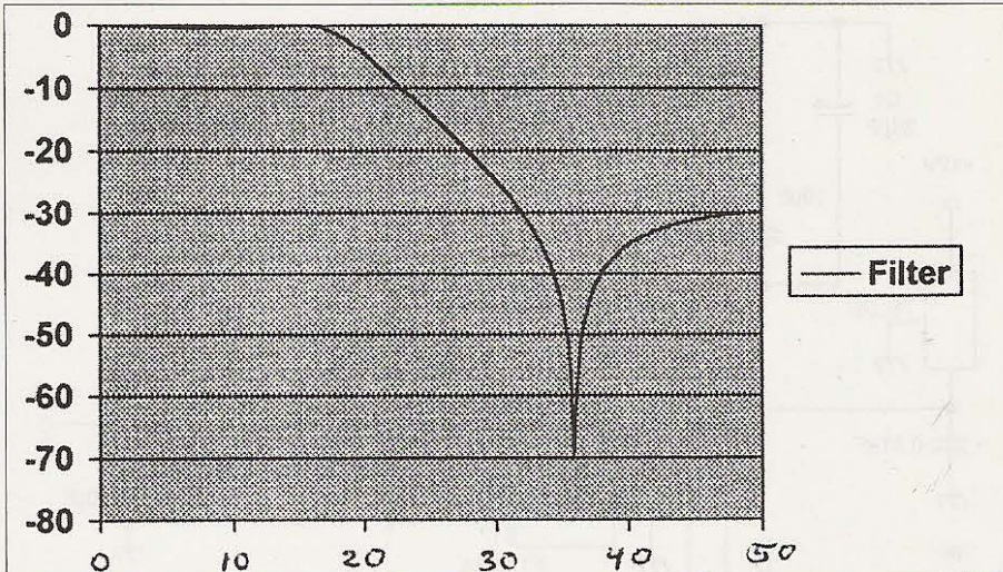
Fig. 4. 20 MHz low-pass filter characteristic (MHz vs. dB).
