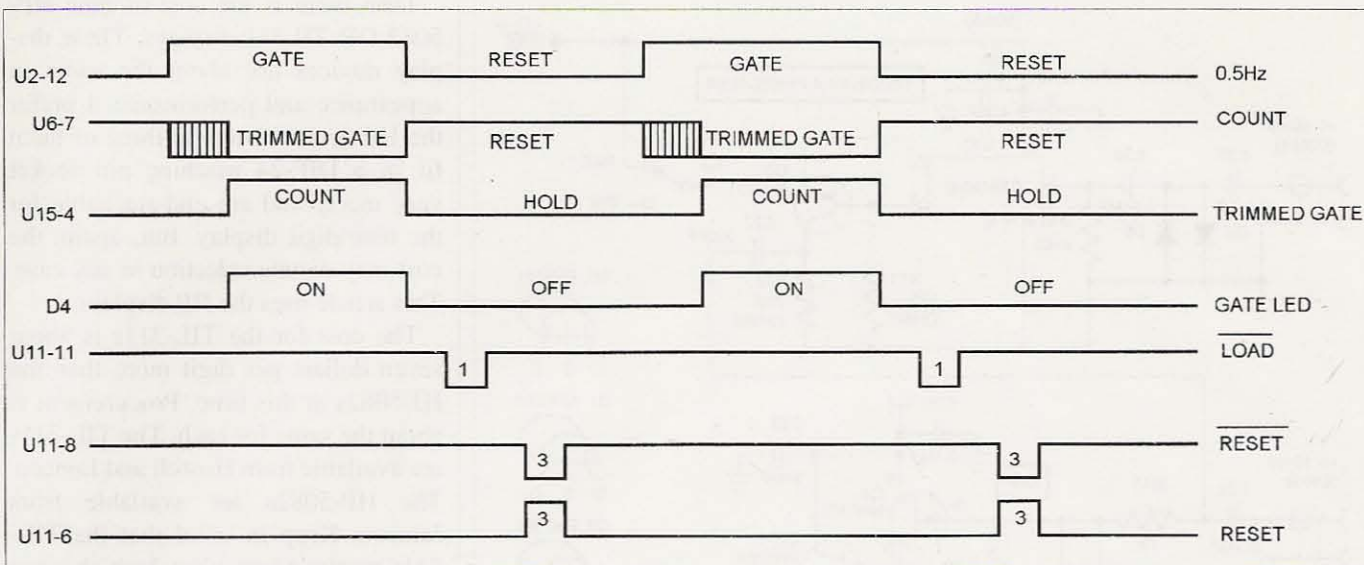
Fig. 1. Timing diagram.
