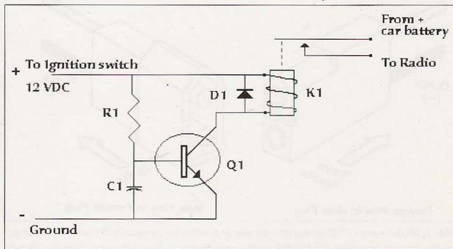
Fig. 1. Schematic.
