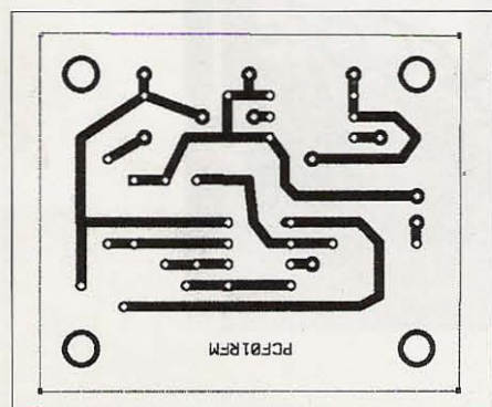
Fig. 3. Foil side of PC board.
