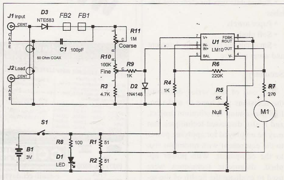
Fig. 1. Relative RF power meter schematic.
