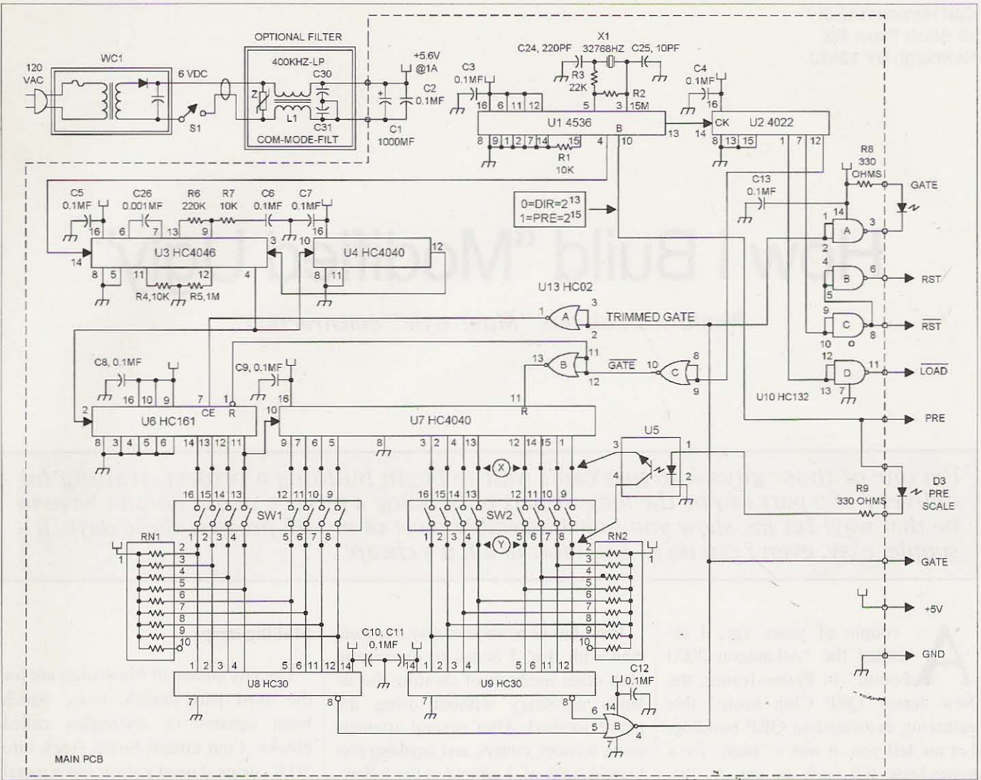
Fig. 4. Main PCB schematic. Note: After calibration of the prescaler, the switch position is used to get the same frequency reading as in the "Direct" mode. After that switch position is found to get the correct prescale number displayed, opto U-5 is used IN PLACE OF that switch position. When prescale is selected, the opto compensates for the toggle propagation delay of U-12. The fiddle factor!
