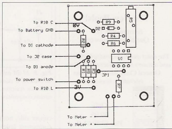
Fig. 4. Parts placement.
