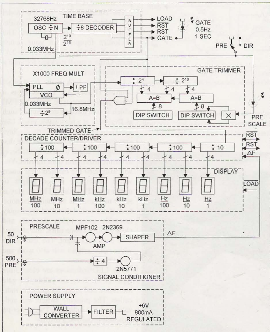
Fig. 2. Functional block diagram.
