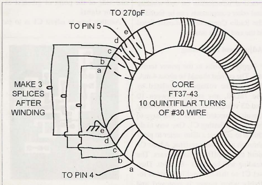
Fig. 3. Winding details for output transformer.
