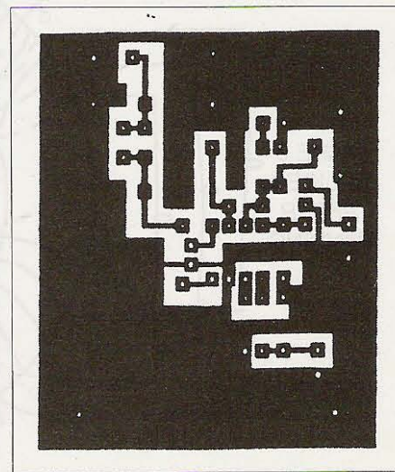
Fig. 6. Circuit board pattern, bottom view.
