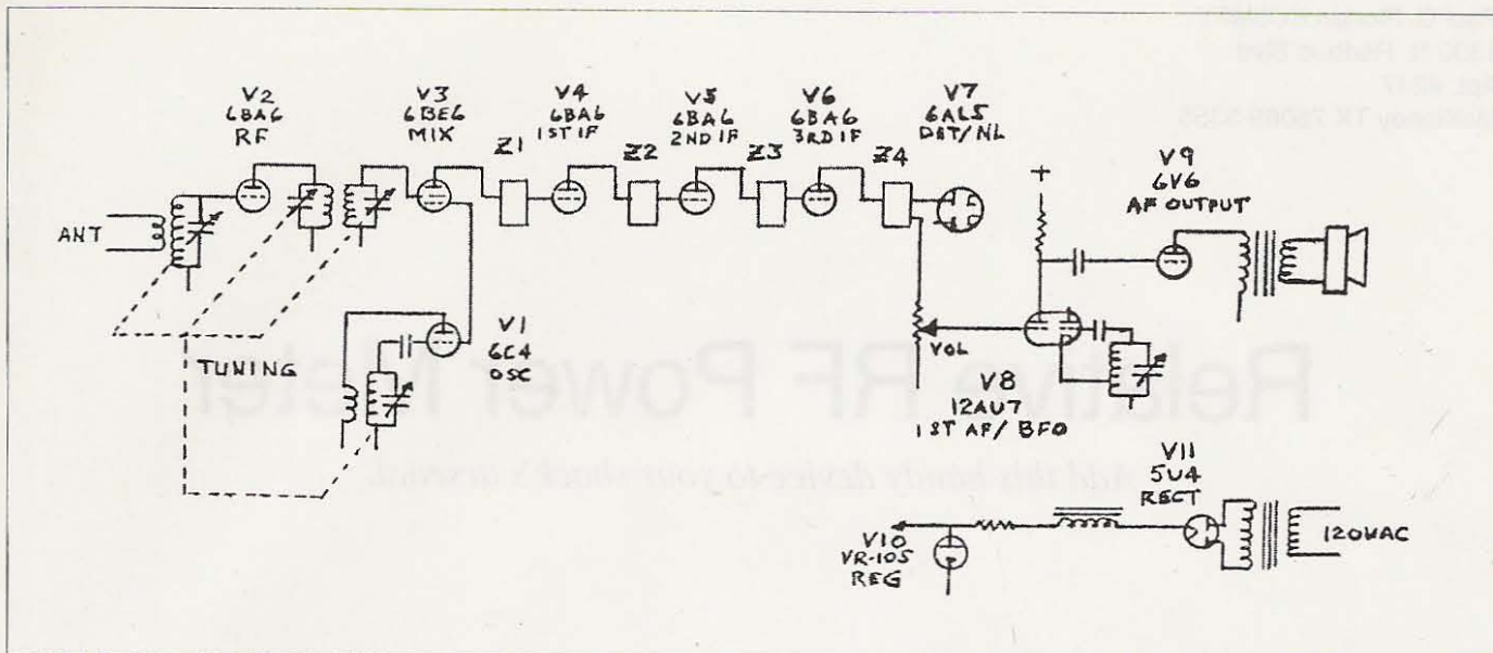
Fig. 2. Functional diagram showing the signal path through the HQ-140-X.
