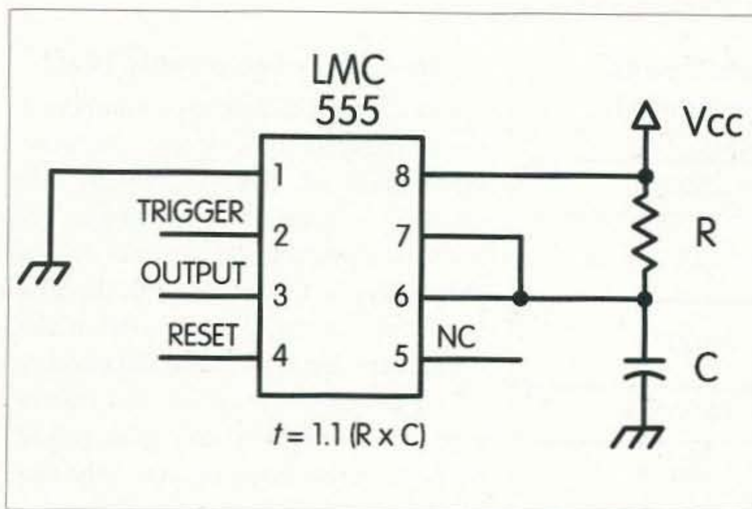
Fig. 1. Typical timeout circuit using LMC555.
