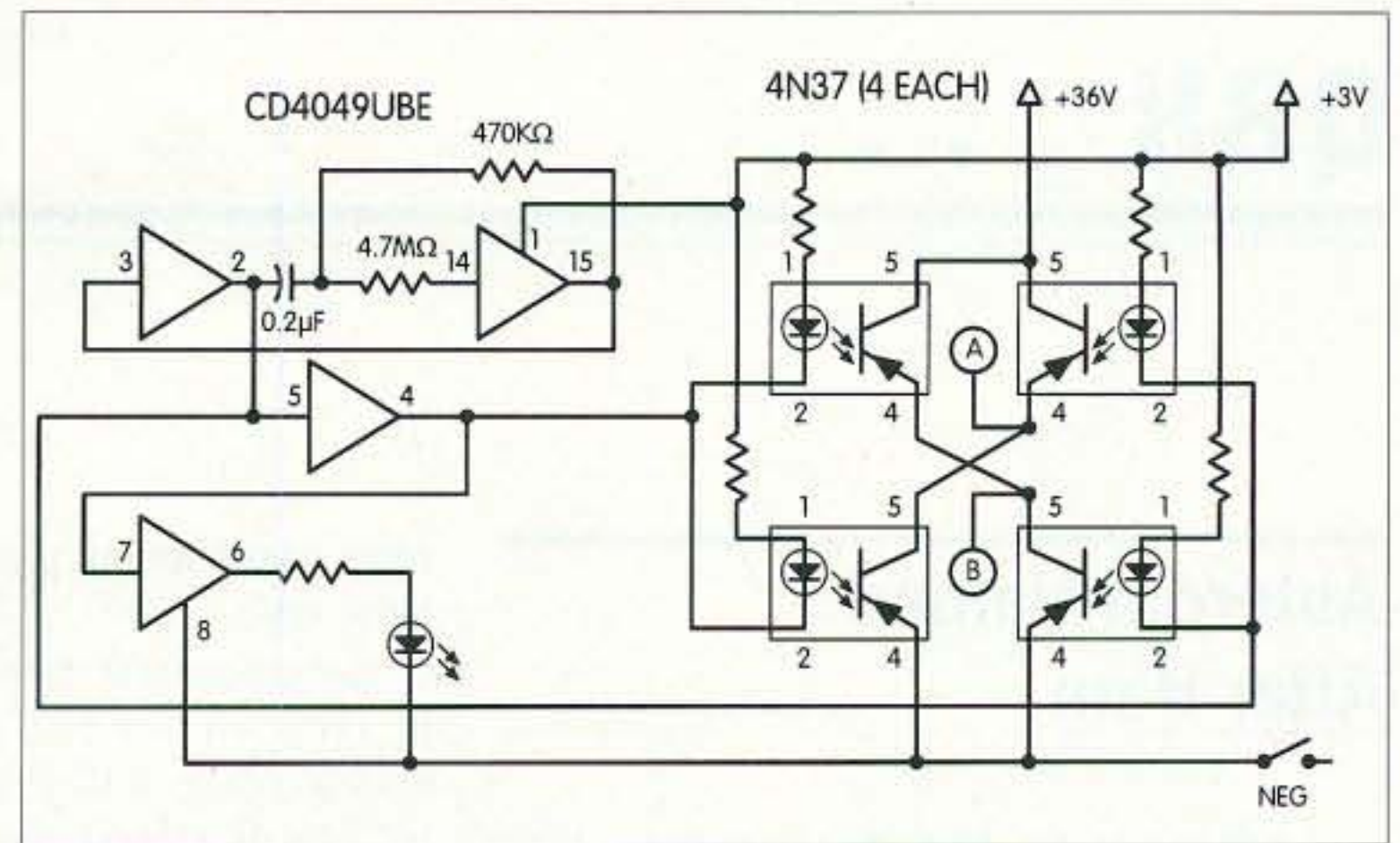
Fig. 2. Yet another "improvement" of the Bioelectrifier.
