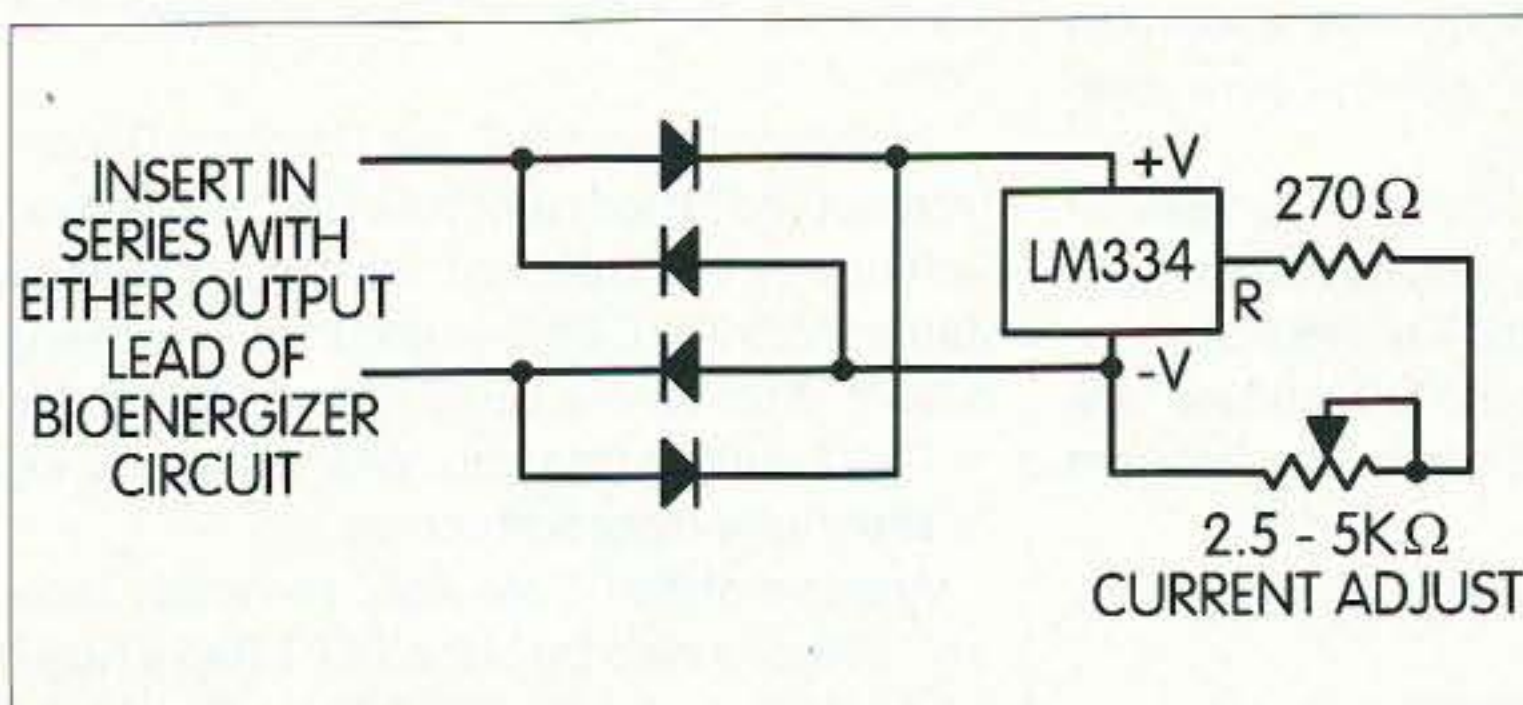
Fig. 1. Another "improvement" for Tom Miller WA8YKN's Bioelectrifier™.
