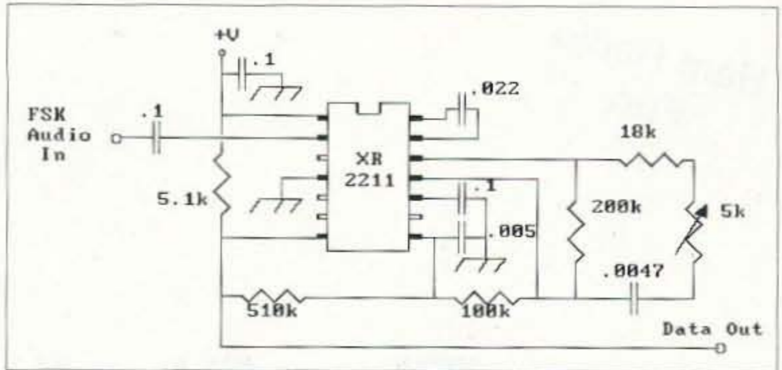
Fig. 1. XR-2211 RTTY demodulator.
