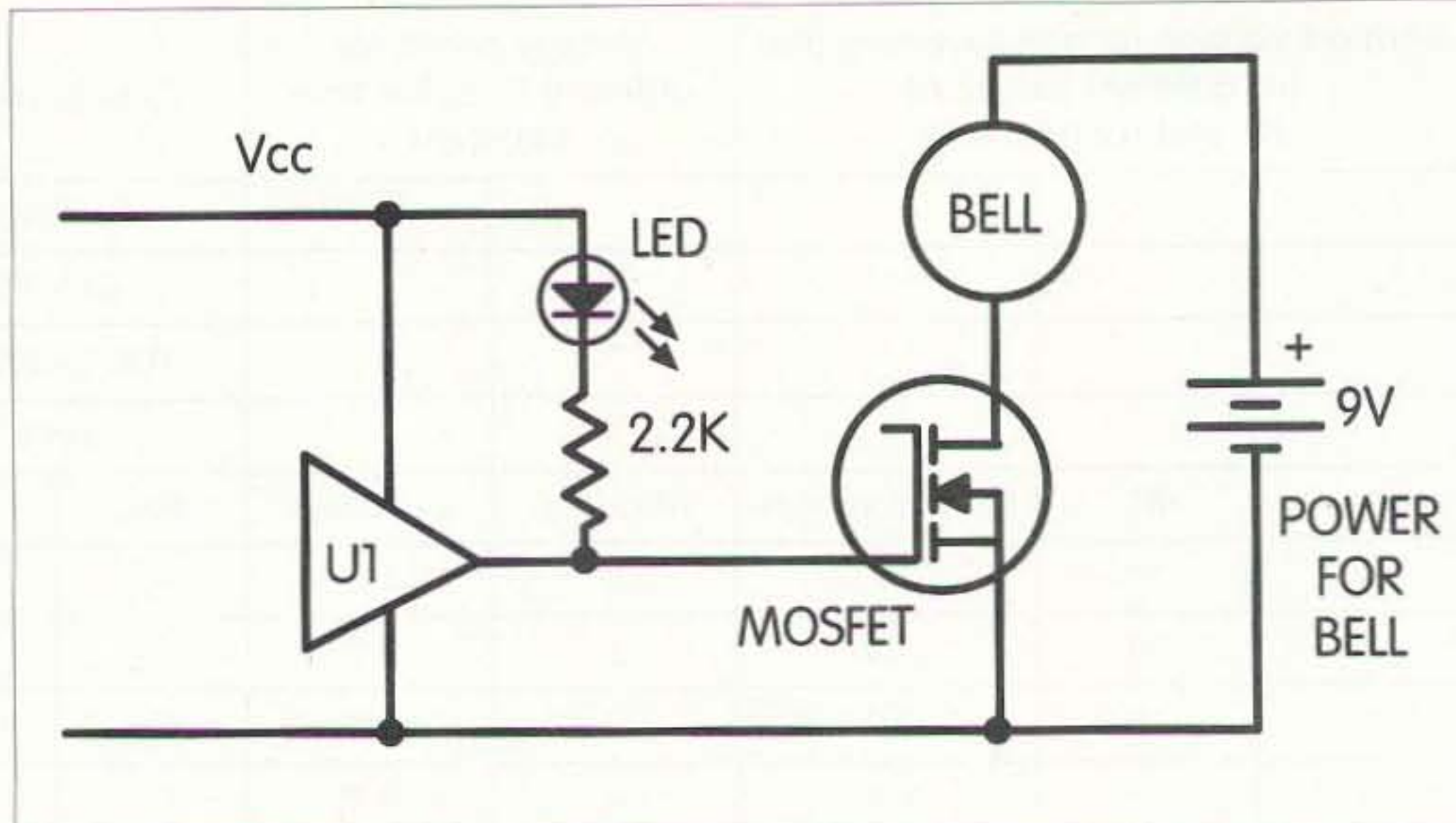
Fig. 4. Test setup for breadboard timing tests.
