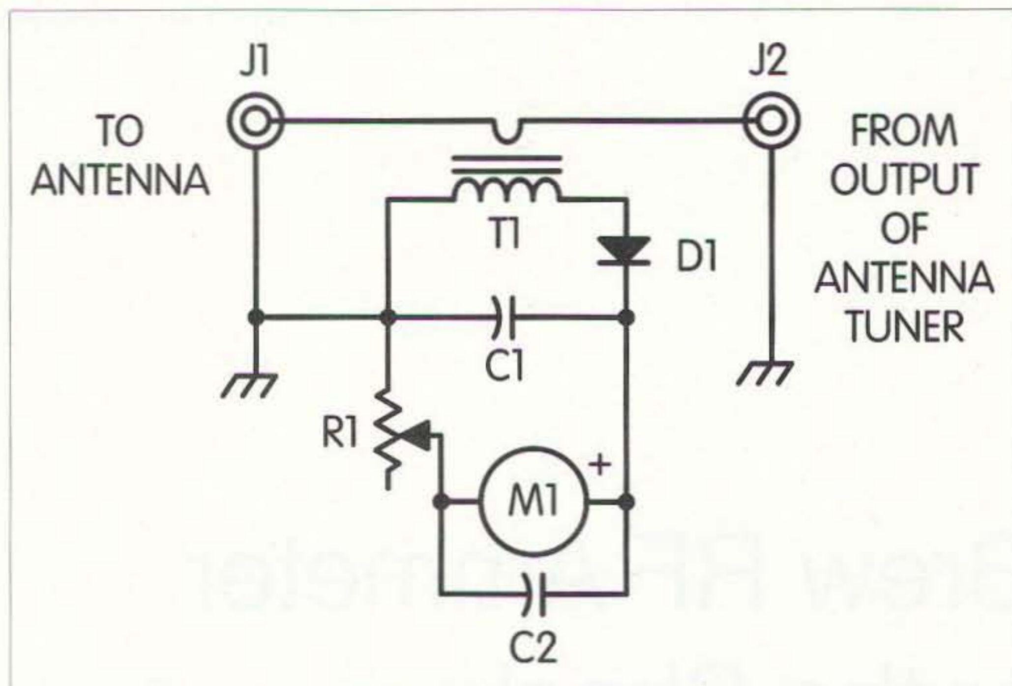
Fig. 1. Schematic for the home-brew RF ammeter.
