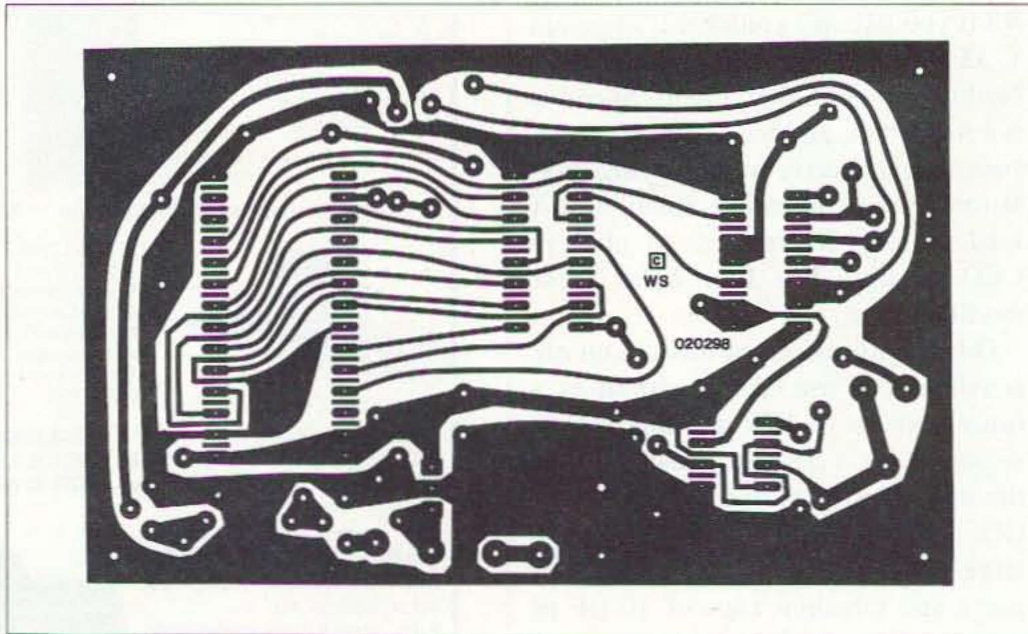
Fig. 3. Foil side of PC board (actual size).
