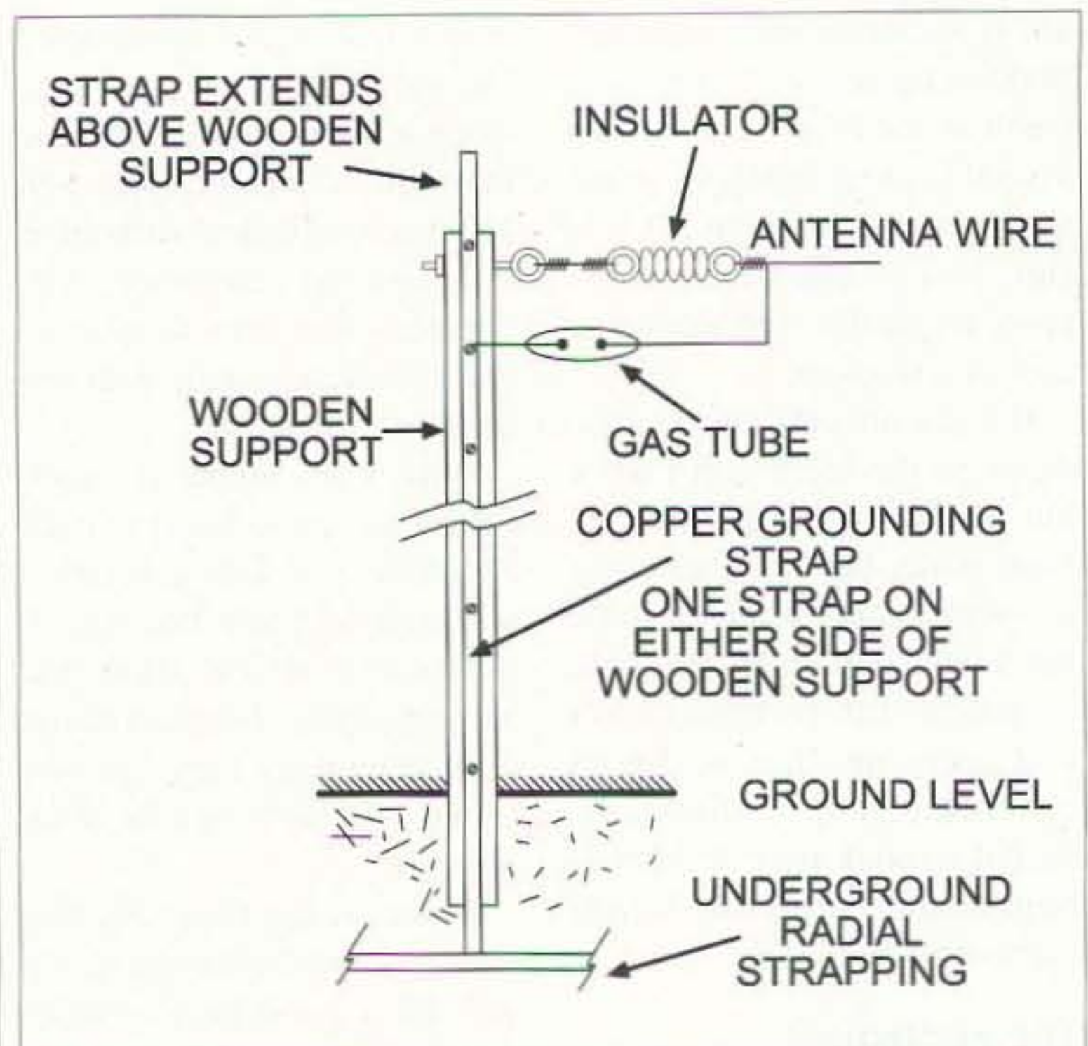
Fig. 1. One method of providing grounding protection for a wooden wire antenna supporting structure.
