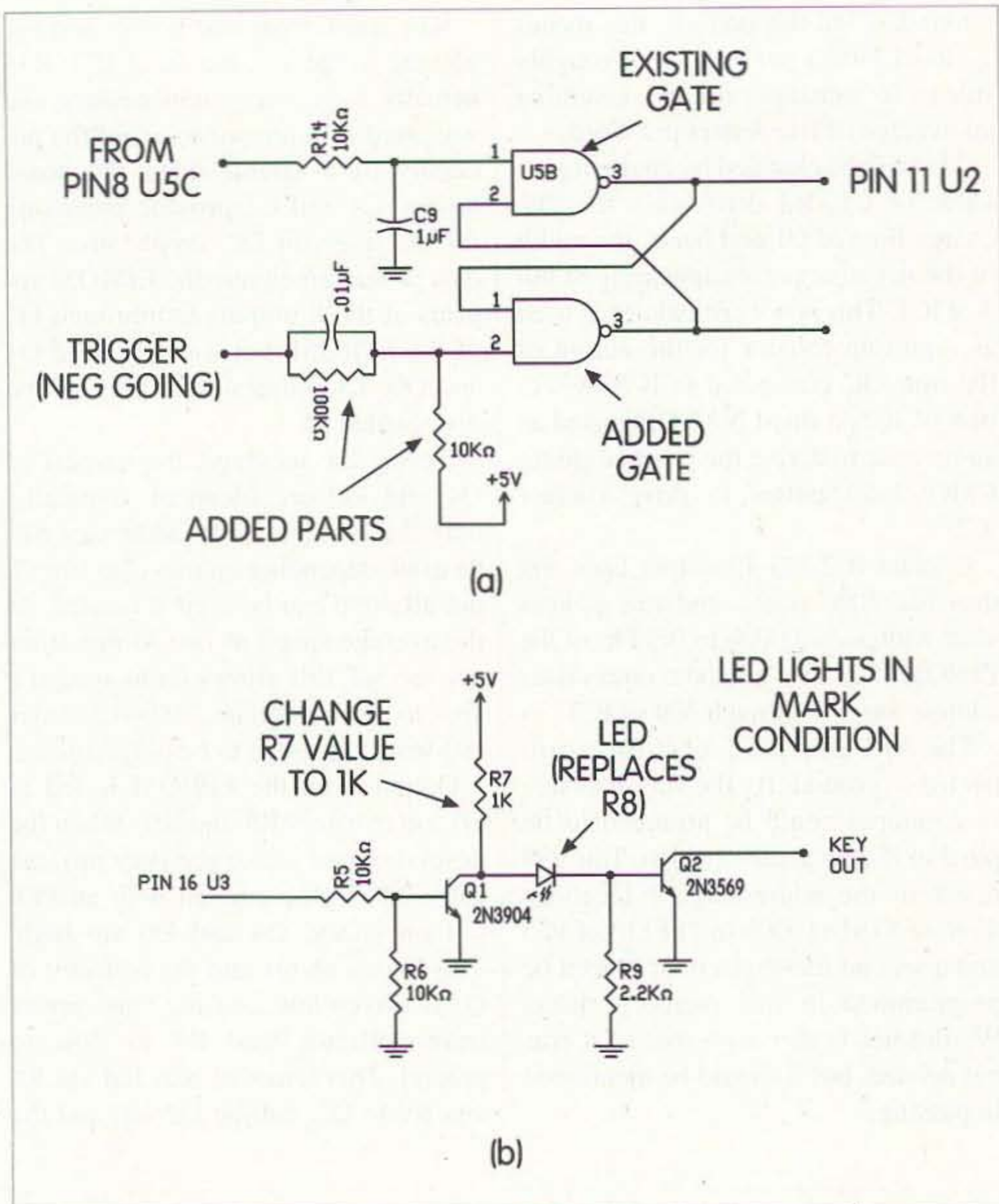
Fig. 2. Modifications. (a) One-shot. (b) Use of LED indicator.
