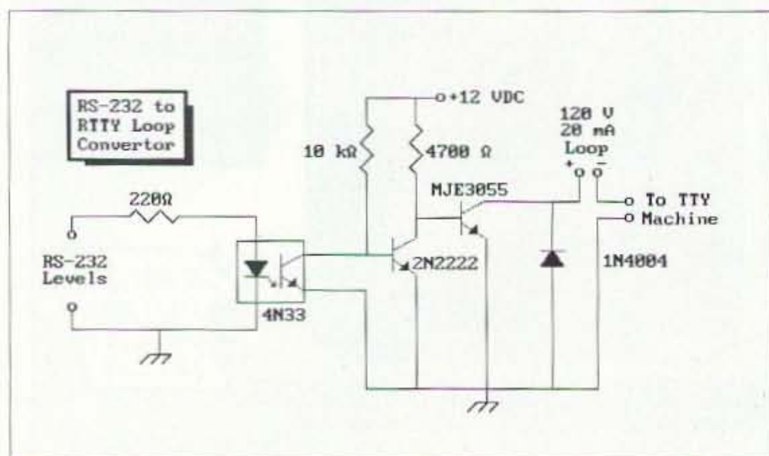
Fig. 2. RS-232 to TTY converter.
