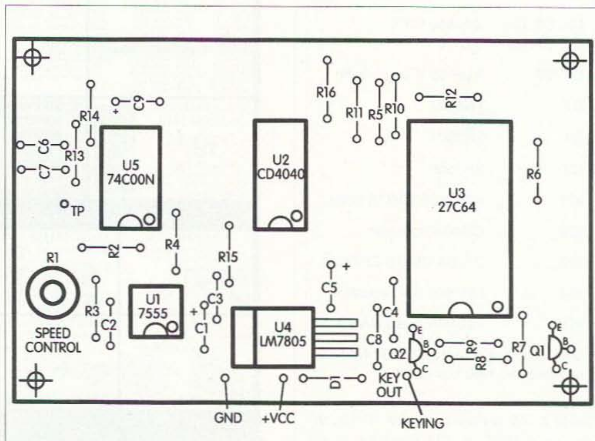
Fig. 4. Parts layout.
