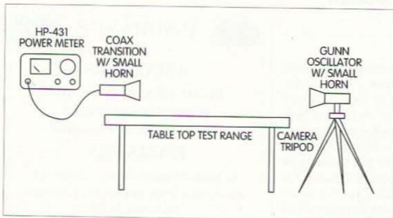
Fig. 1. Antenna test range constructed on a tabletop. The microwave power meter is located on one end and the test transmitter (10 GHz Gunn oscillator located on small camera tripod) is on the other end of the test range.
