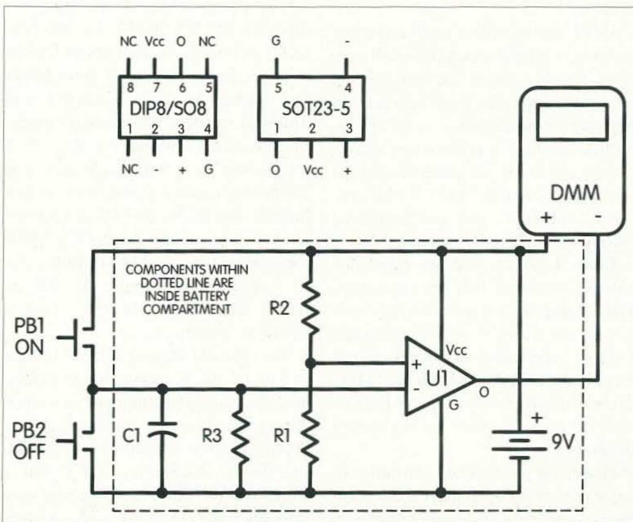
Fig. 2. Schematic of automatic shutdown switch.
