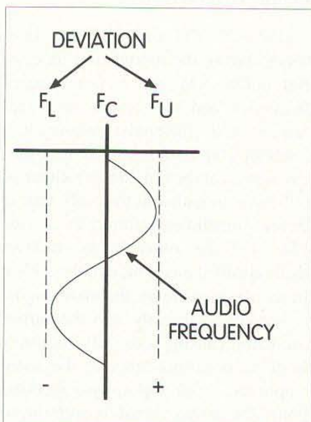
Fig. 1. Relationship of deviation to the audio voltage.
