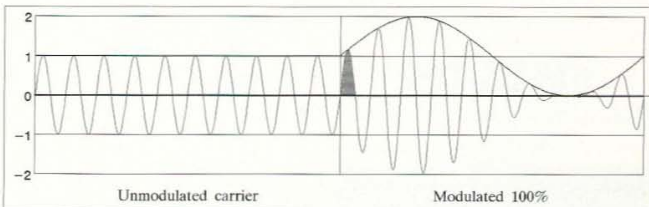
Fig. 6. Calculating the power of a 100% modulated carrier.
