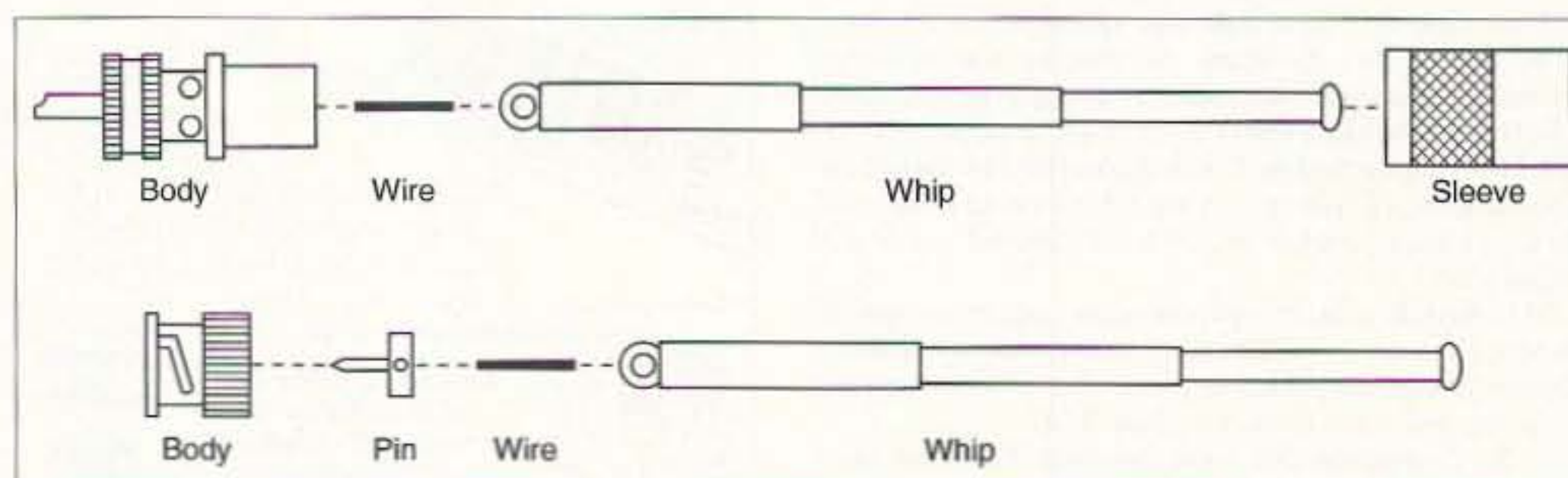
Fig. 1. Whip antennas, exploded views.
