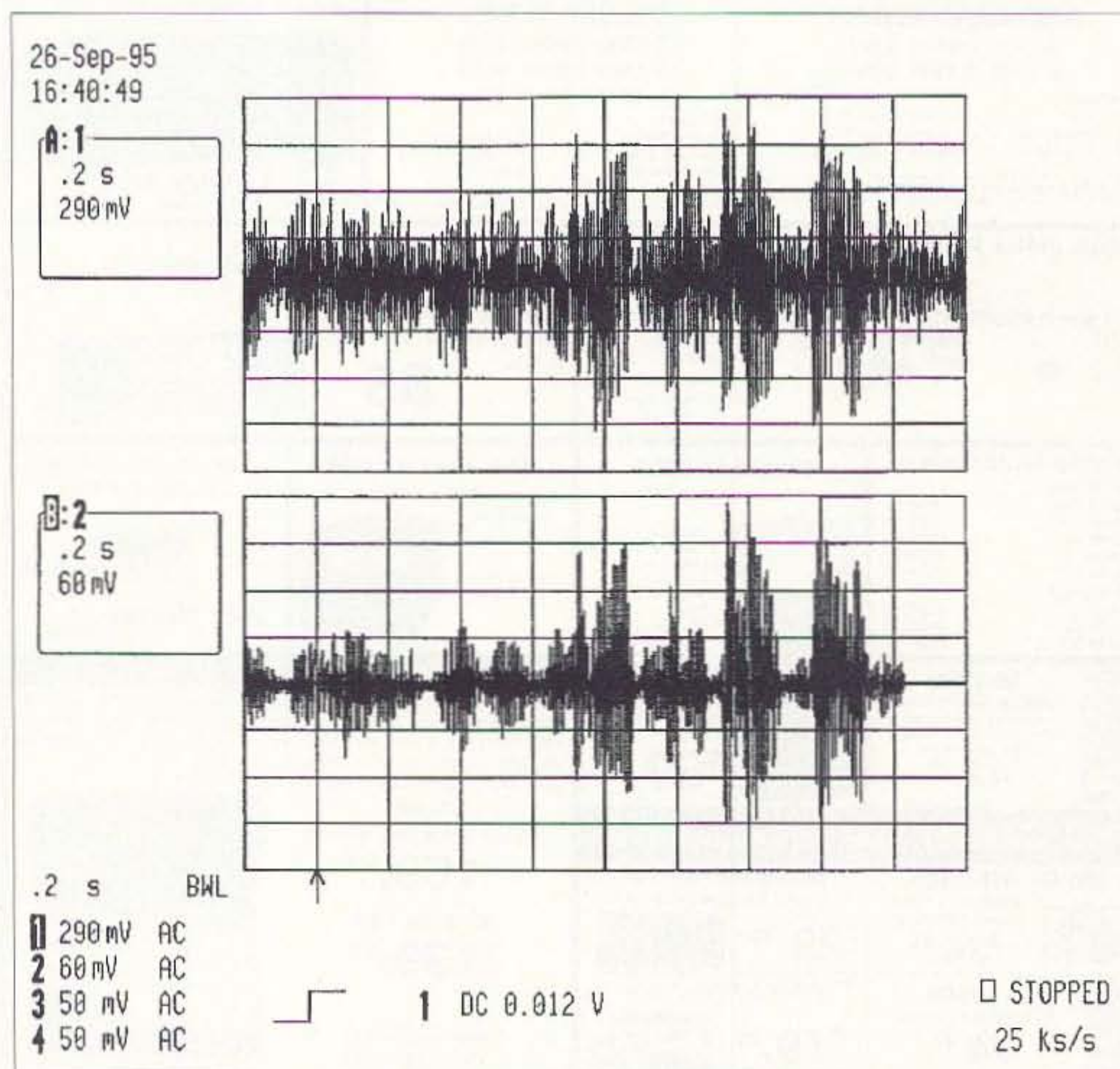
Fig. 1. The upper trace shows the unprocessed audio of a phone station in the noise. The lower trace shows the effect of the NIR-12, NIR mode only, NIR control set to 10 o'clock. The pattern displays amplitude on the vertical axis, time on the horizontal. The timing has been adjusting to compensate for the NIR-12's delay.
