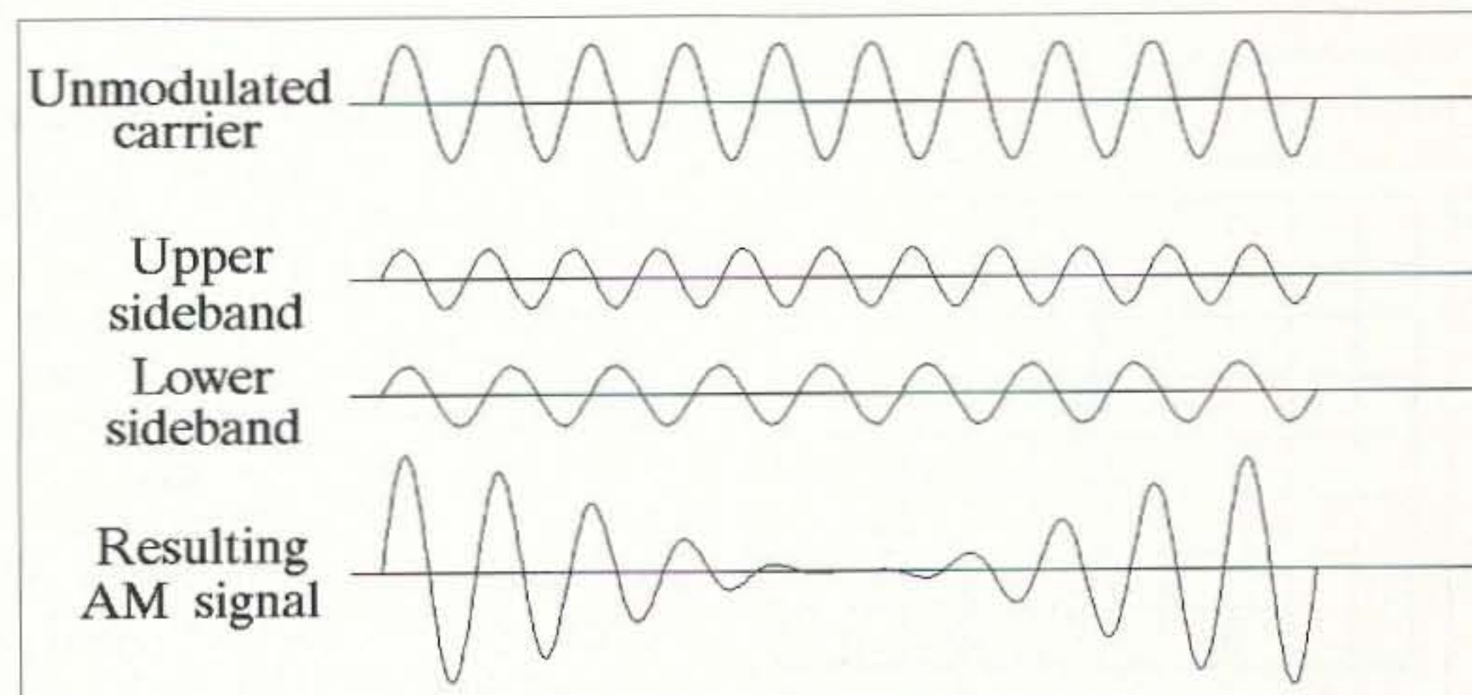
Fig. 3. The carrier and its sidebands.
