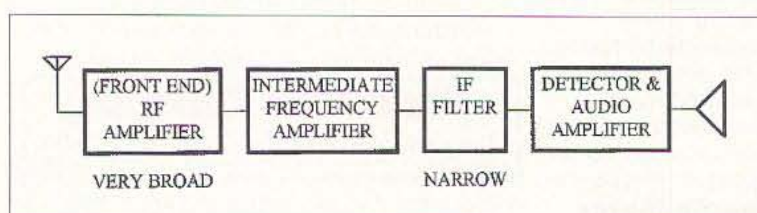
Fig. 1. Block diagram of a typical superheterodyne receiver. Selectivity is developed late in the circuit, in the IF filter. The earlier stages, especially the RF front end, are wide open to overload by strong adjacent signals and other noise.
