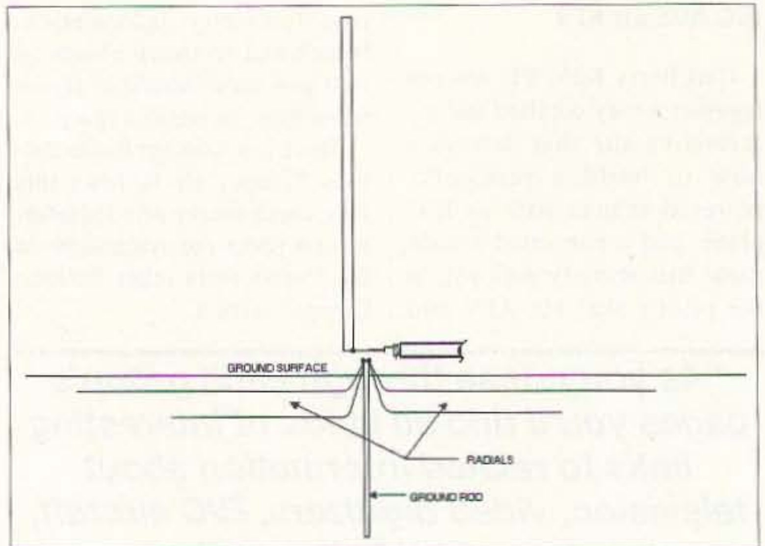
Fig. 2. Radial installation used with ground-mounted verticals (base insulator not shown).
