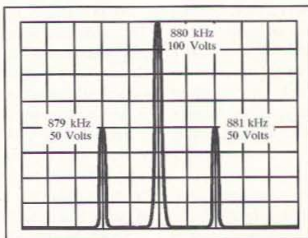
Fig. 2. 880 kHz carrier modulated 100% by 1 kHz.
