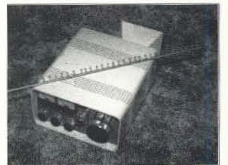
Photo B. The antenna on top of the rig is a 40-element loop yagi for 10 GHz. It measured 15.5 dBi at the Central States VHF Antenna Contest. (Photo courtesy of Kent WA5VJB.)
