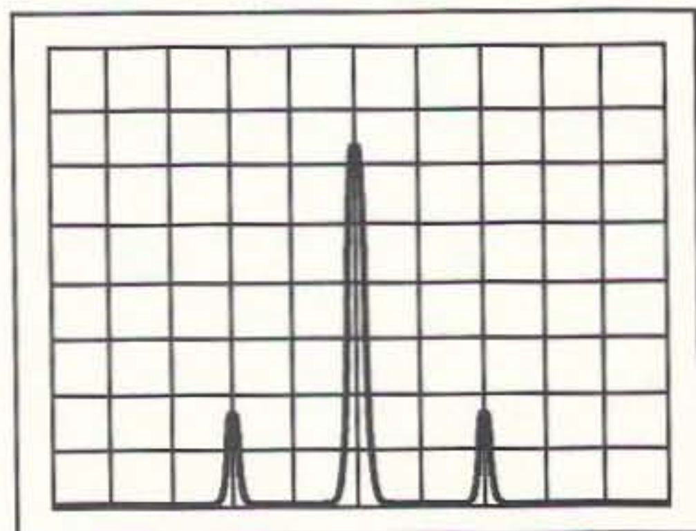
Fig. 4. What is the modulation percentage?
