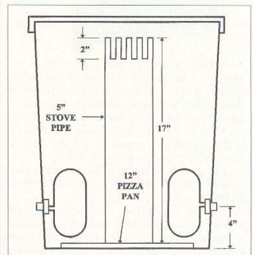
Fig. 2. Cross section of cavity, showing dimensions of inner conductor and placement of coupling loops.
