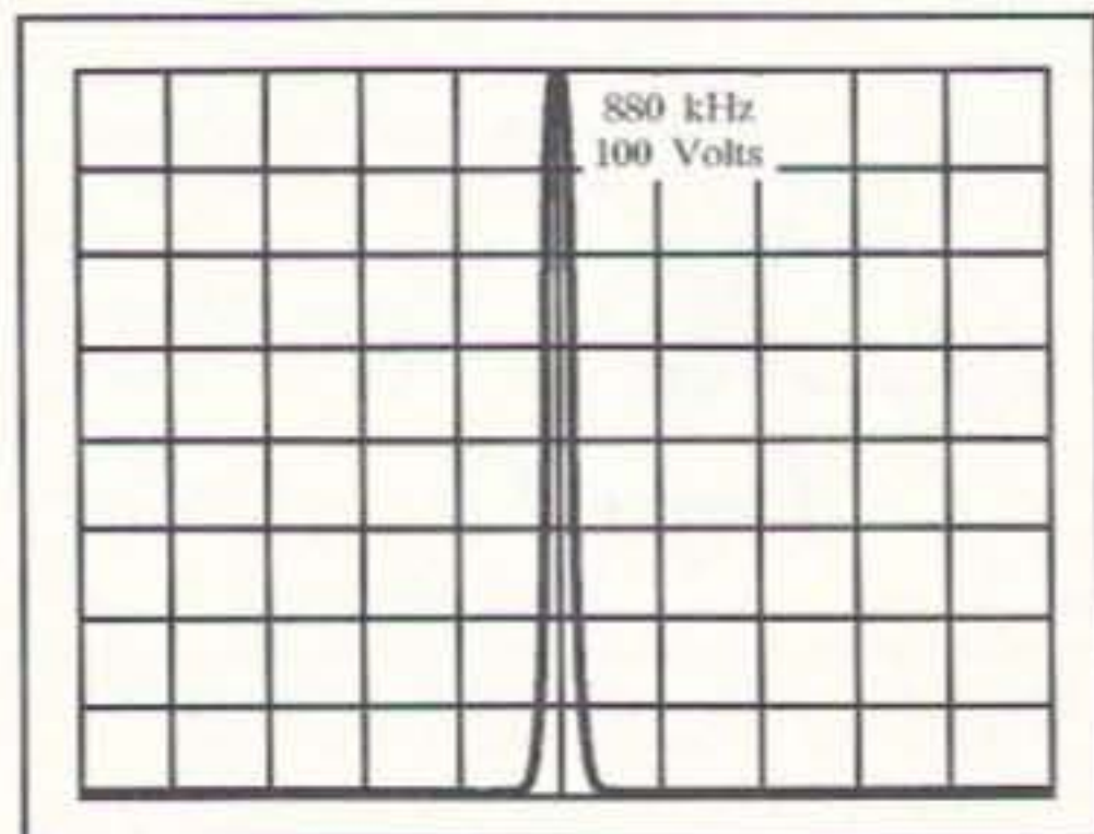
Fig. 1. An unmodulated carrier at 880 kHz.
