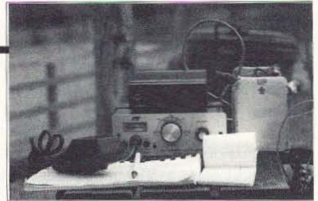
Photo A. AC4HF's portable setup, using the MFJ-9420 and a Radio Shack DSP unit. (Photo by AC4HF.)
