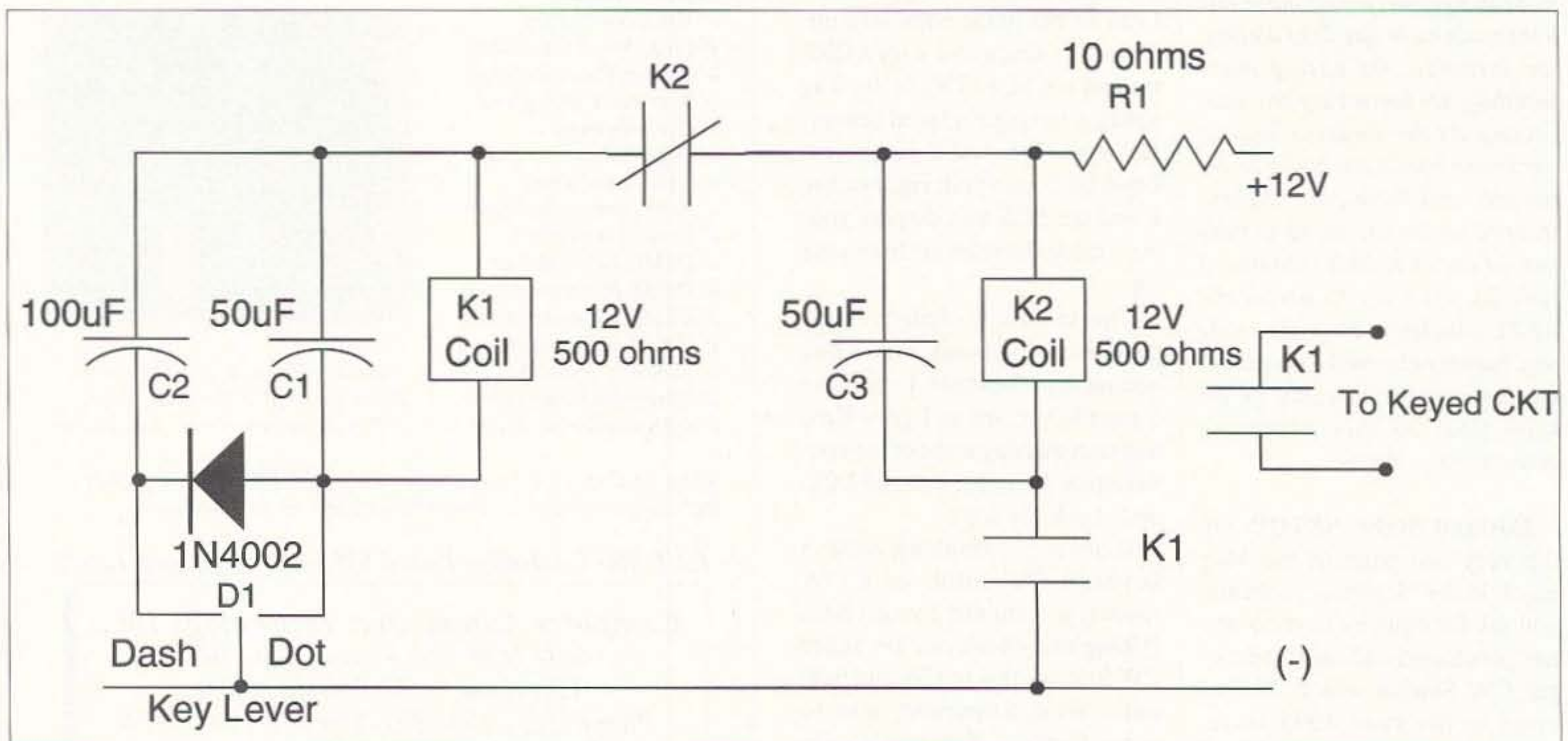
Fig. 1. Schematic for the JB Keyer.
