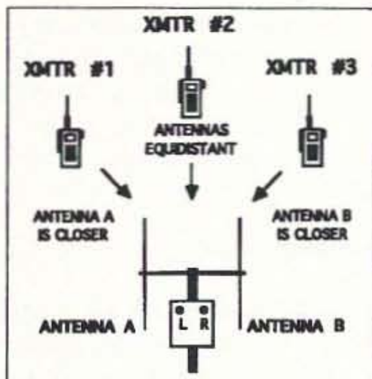
Fig. 1. TDOA RDF sets such as the VF-142Q get bearings by determining which of its two vertical antennas is closest to the transmitter. Differences in arrival time produce differences in the phase of the signals from each antenna. Accordingly, some hams prefer to call these units "phase front detectors."
