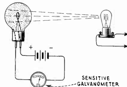
Fig. 14 - EFFECT OF LIGHT ON THE PHOTOTUBE.
