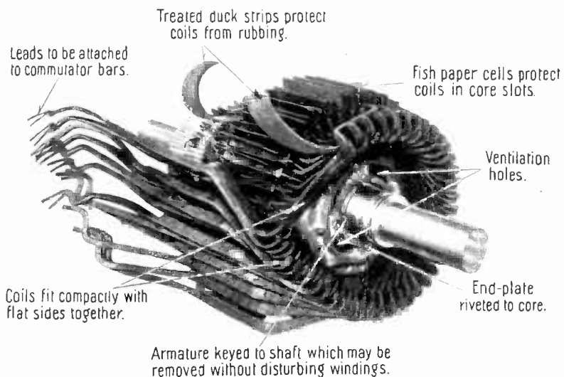
Partially Wound Armature
