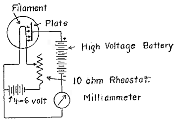
Fig. 96 Diagram of bulb showing flow of Electrons
