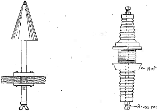
Fig. 76. Bradfield Deck Tube. Fig. 77. Electrose Deck Insulator.
