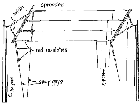
Fig. 75. Marconi Ship Aerial
