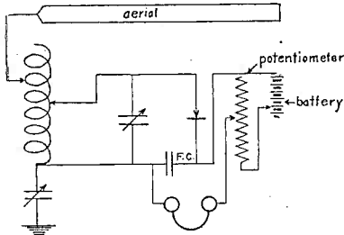
Fig. 81. Conductively Coupled Set.
