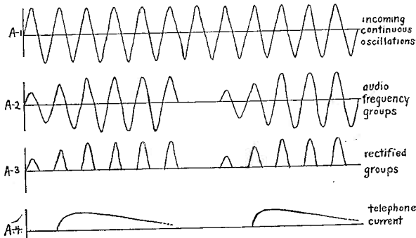
Fig. 91. Curves showing action of tapper or slipping contact detector.
