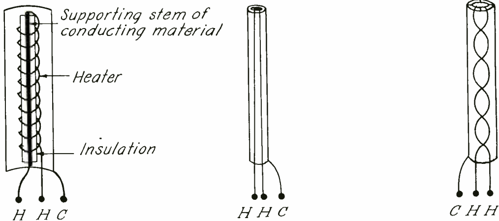
Fig. 5.—Mechanical arrangement of heaters.
