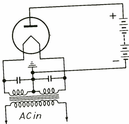
Fig. 17.—Use of a.c. to heat tube filament.
