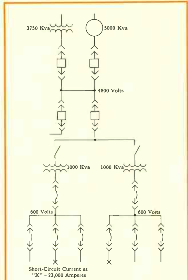
Fig. 1—Typical load-center system.
