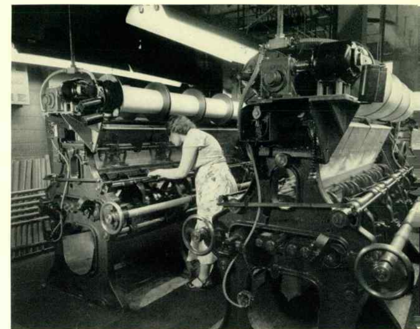
Failure to maintain tension very exactly on looms and warp-knitting machines shows up as a defect in the product. A new electronic beam let-off, as used on this tricot machine, prevents this.
