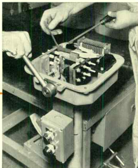
Fig. 3—The master switch used on the log-carriage drive.
