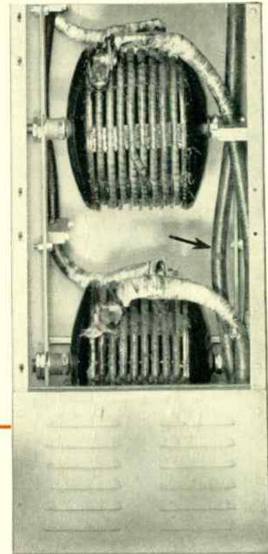
Fig. 5—Test installation of 0.025-ohm, 600-ampere, type-MSP reactors. Arrow indicates cable that was bent out of line by forces built up under short-circuit conditions.
