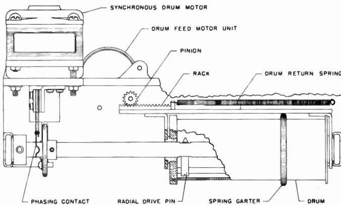
Figure 6. Desk-Fax drum and its drive mechanism
