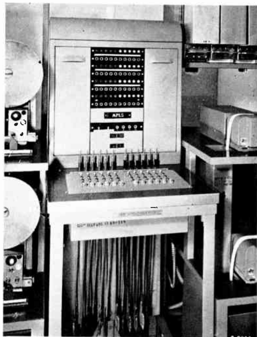
Figure 2. Turret switching table—Plan 31 switching unit, Chicago, Ill.
