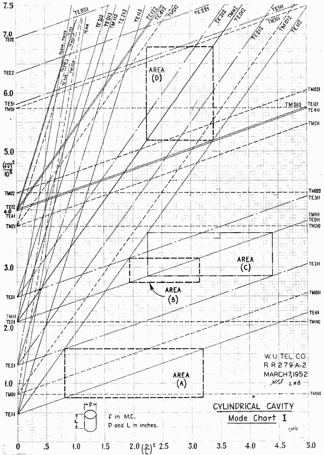
Figure 1. Cylindrical cavity mode chart
