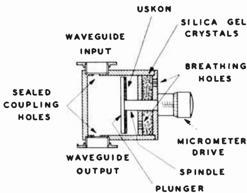
Figure 10. Cavity layout
