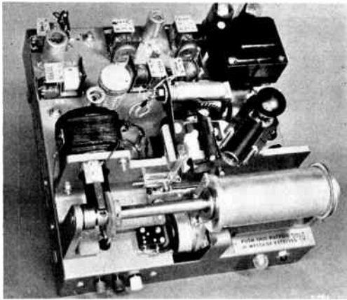
Figure 5. Complete assembly with tubes and control relays at rear, mechanical elements at front
