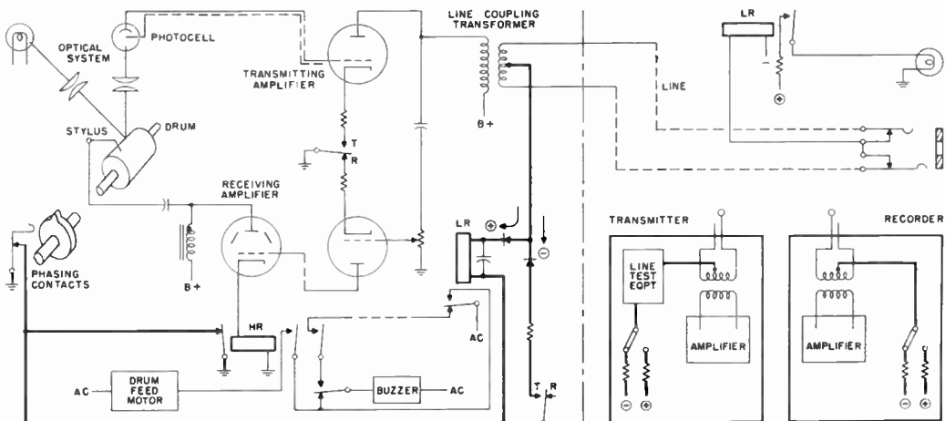
Figure 10. Simplified schematic circuits — see text
