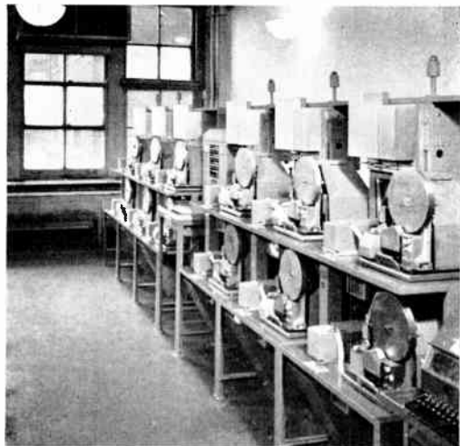
Figure 1. Plan 31 switching from branch offices, Chicago, Ill.
