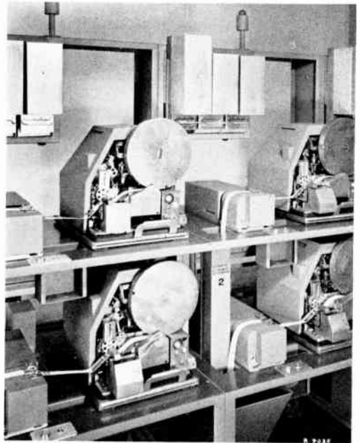
Figure 4. Plan 31 receiving reperforators and distributor transmitters
