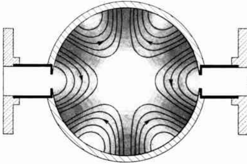
END PLATE CURRENTS FOR TE_{31} MODE
