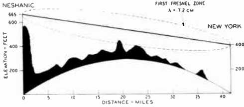
Figure 6. Profile of New York to Neshanic path
