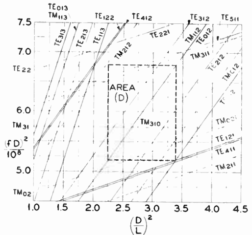
Figure 5. Mode chart Area D
