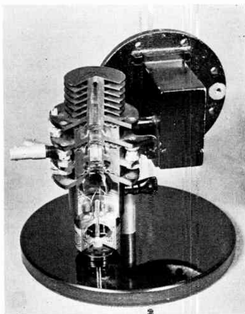
Figure 2. Sperry SAC-41 tube
