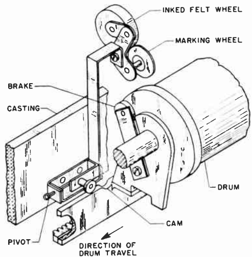
Figure 7. Inked wheel marks "sent" telegrams
