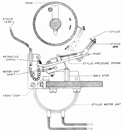
Figure 8. Separate motor actuates stylus-wire holder
