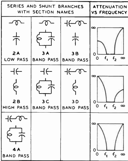
Figure 2. Filter sections associated with Figures 4, 5, and 6
