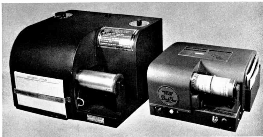
Figure 1. Optical facsimile transceiver of 1933 and new small Desk-Fax model
