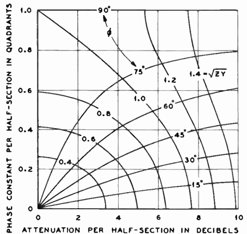
Figure 1. Propagation constant as a function of \sqrt{ZY} / \phi
