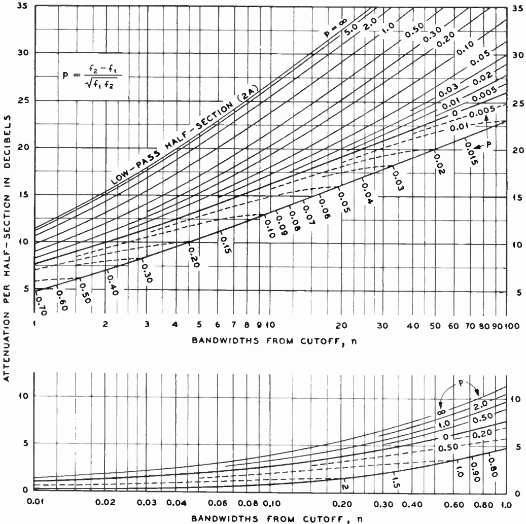
Figure 4. Chart for sections 2A, 3A, and 3B
