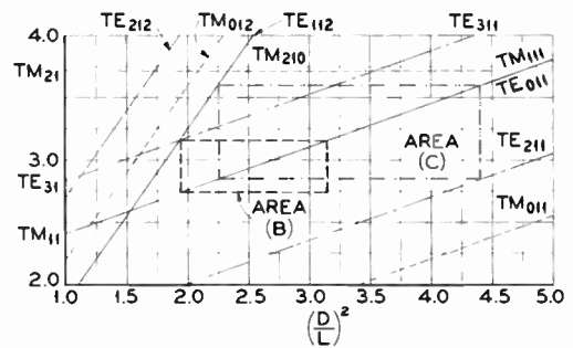
Figure 3. Mode chart Areas B and C
