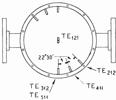
Figure 6. Positions for mode suppressors
