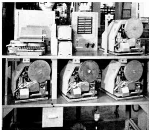
Figure 3. Plan 31 RQ-BQ switching position showing turret and receiving reperforators
