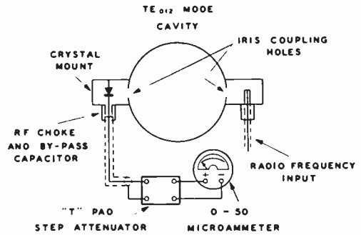
Figure 11. Circuit layout
