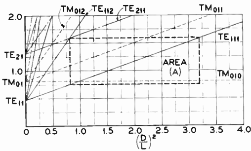
Figure 2. Mode chart Area A
