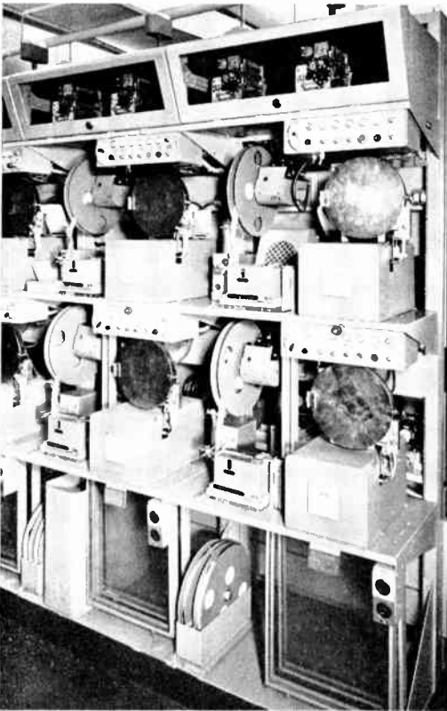
Figure 4. Trunk sending positions
