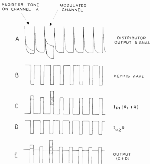
Figure 6. Synchronous gate—theory
