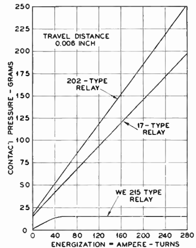
Figure 8. Relation between energization and contact pressure
