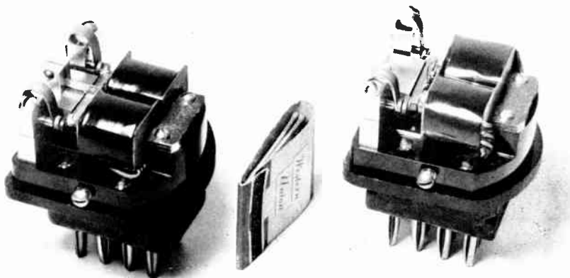
Figure 3. Type 202-A Relay
