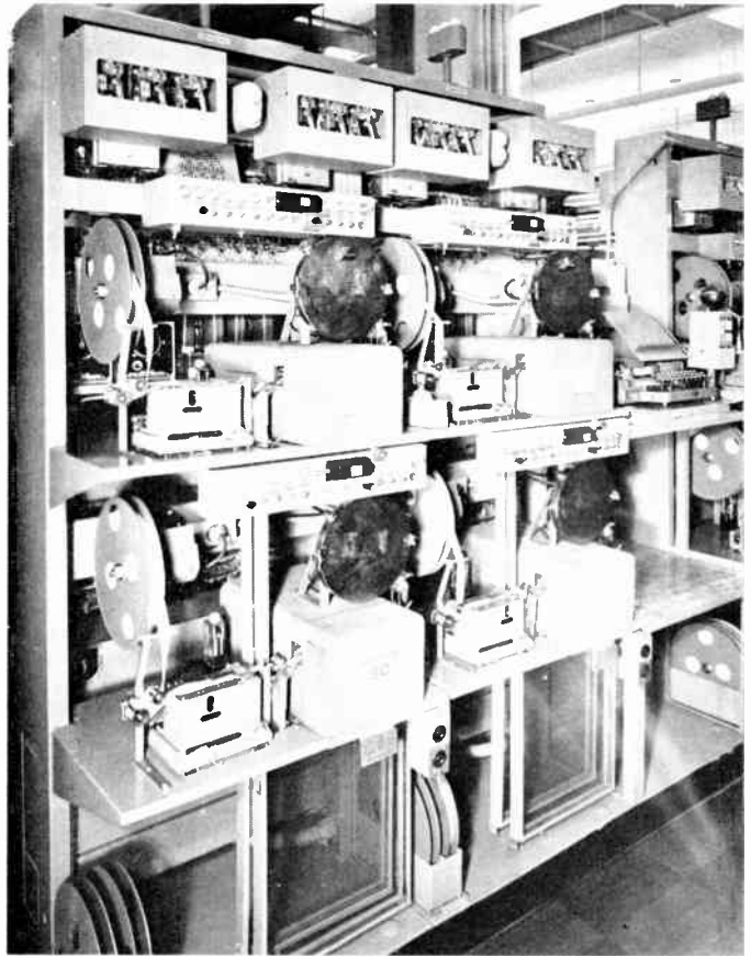
Figure 7. Line receiving position for heavily loaded tributary and branch office circuits
