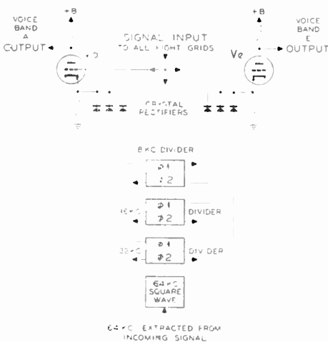
Figure 4. Receiving distributor—theory
