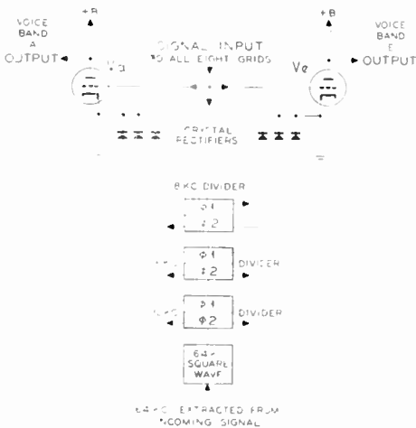
Figure 4. Receiving distributor—theory
