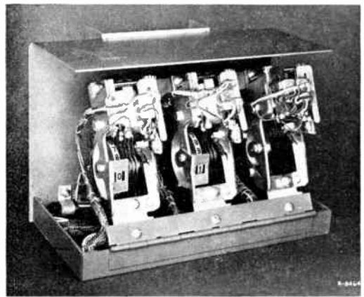
Figure 10. Sequence number indicator
