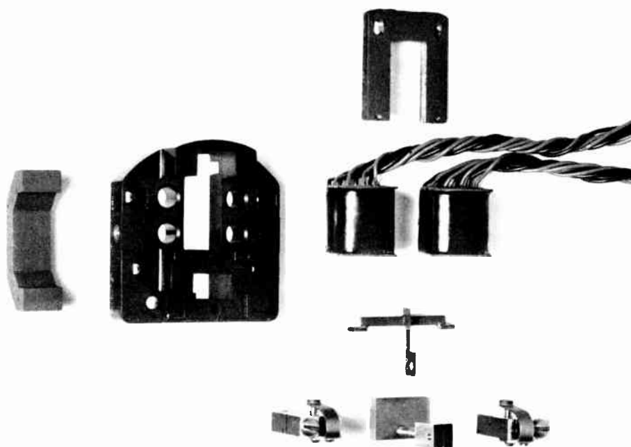
Figure 4. Functional components of Type 202-A Relay
