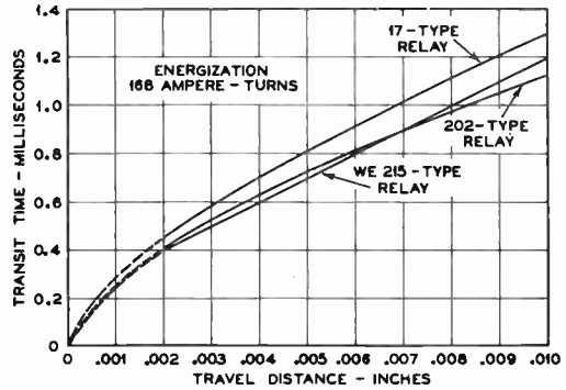
Figure 6. Relation between travel distance and transit time
