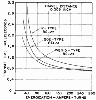
Figure 7. Relation between energization and transit time
