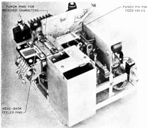
Figure 9. Intraoffice reperforator equipped with read-back pins
