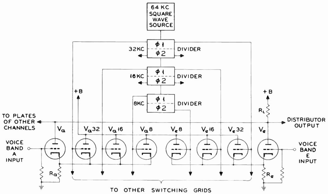
Figure 2a. Sending distributor—theory
