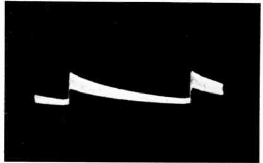
Figure 12. Output of pulse stretcher
