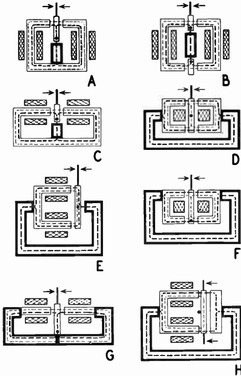
Figure 1. Magnetic circuits
