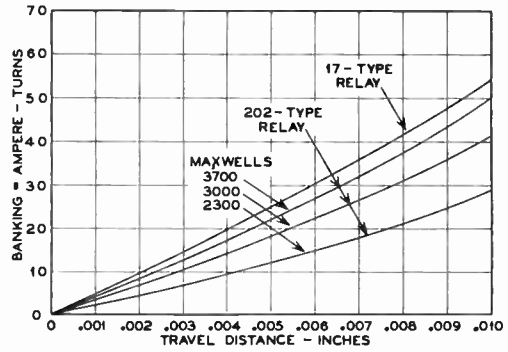
Figure 5. Relation between travel distance and banking
