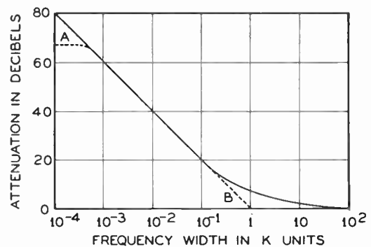
Figure 7. Graphical method of determining K
