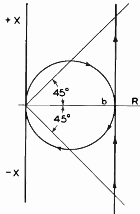
Figure 2. Impedance diagram, limiting case
