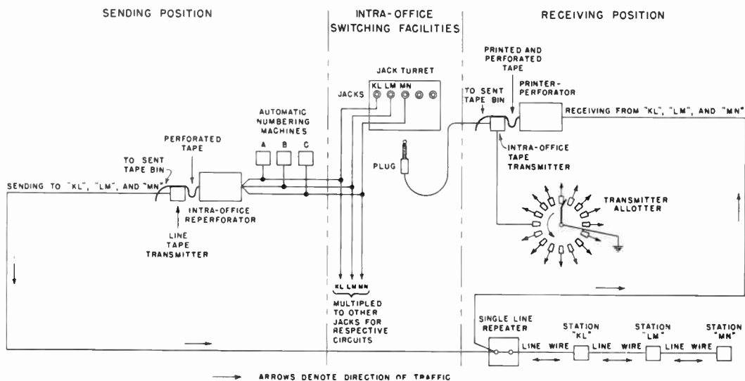
Figure 20. Way-circuit switching
