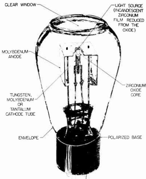
Figure 1. Concentrated-arc lamp—cut-away view
