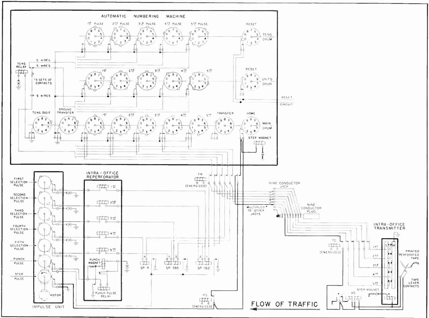
Figure 13. Intra-office transmission
