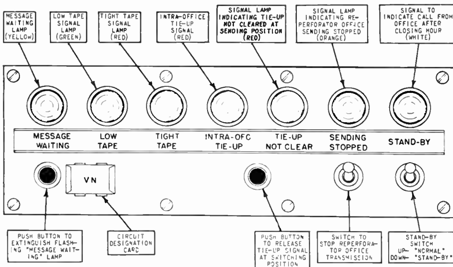
Figure 23. Teleprinter signal and control unit
