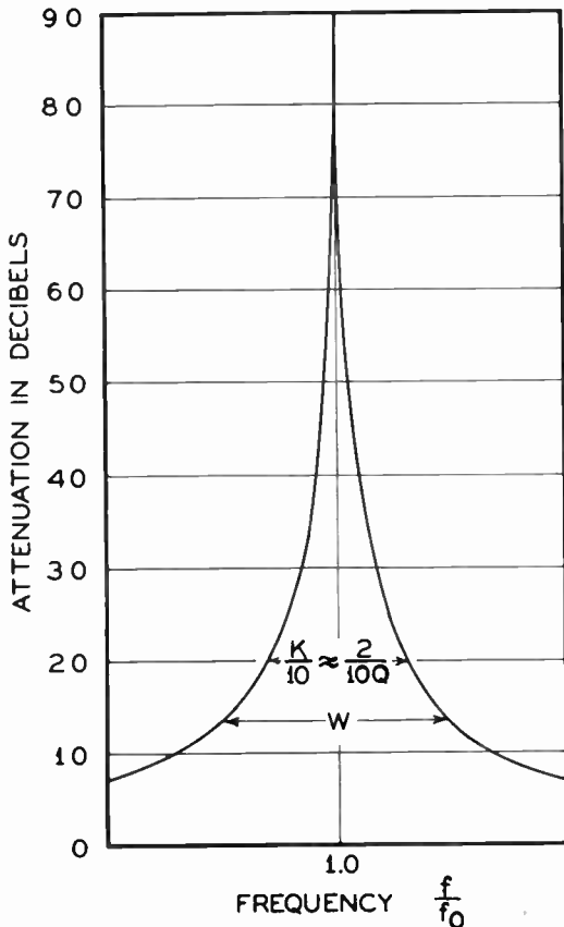
Figure 6. Attenuation of single rejection filter
