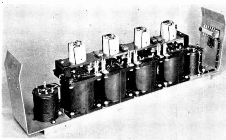
Figure 4. Tandem filter showing trimmer capacitors
