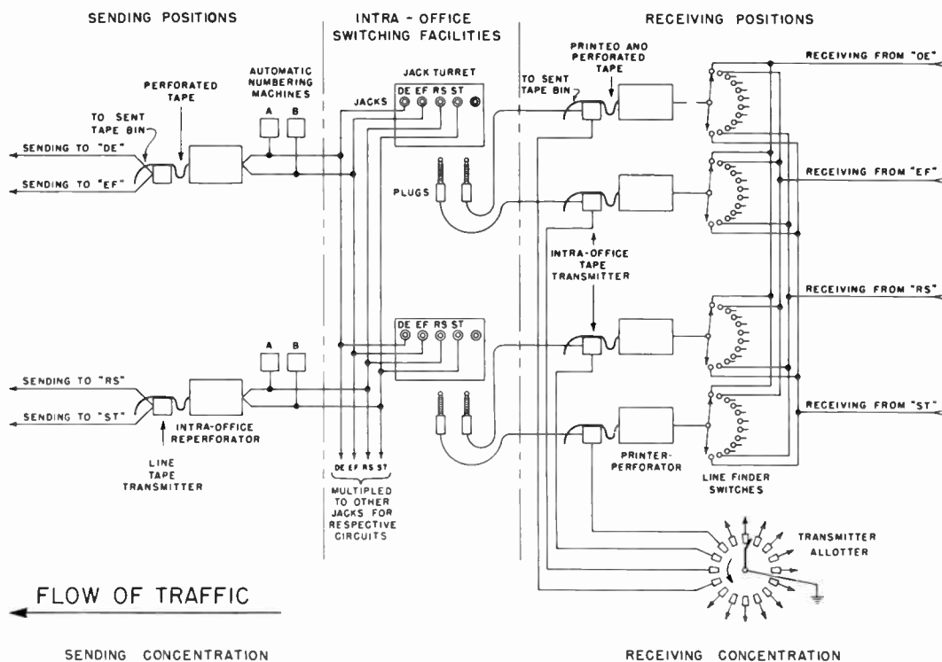
Figure 19. Receiving and sending concentration
