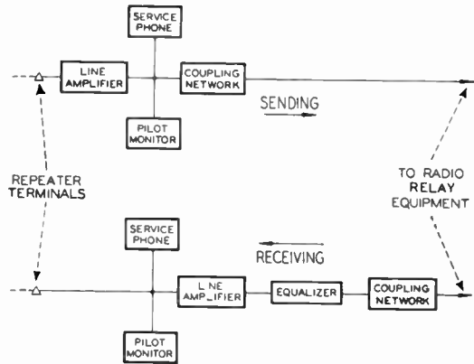
Figure 7. Terminal repeater
