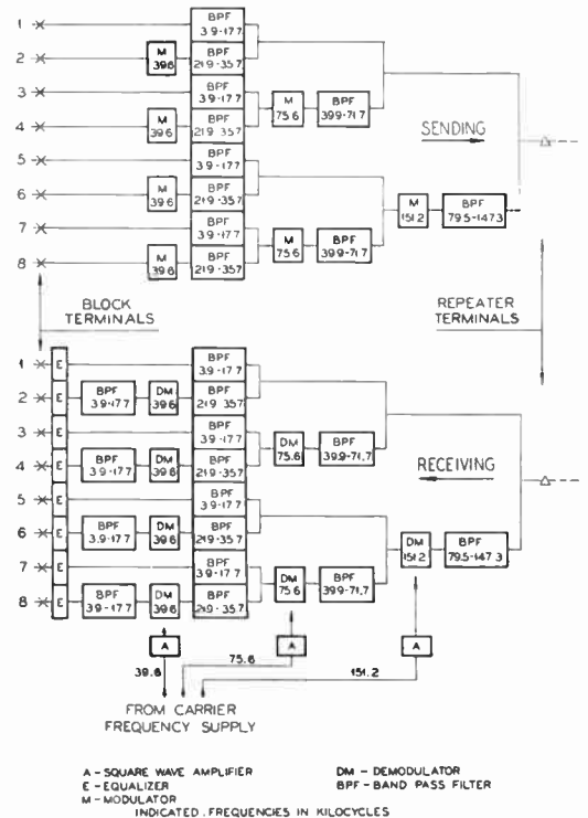
Figure 4. Block modulator group
