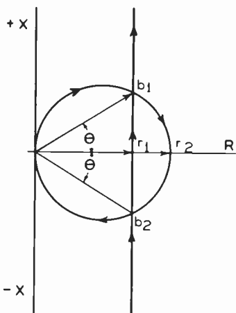
Figure 3. Impedance diagram, general case
