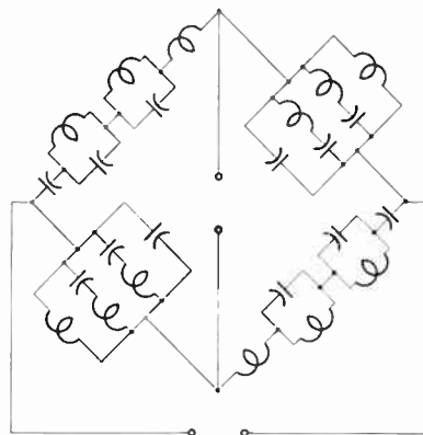
Figure 9. Multiple frequency rejection filter
