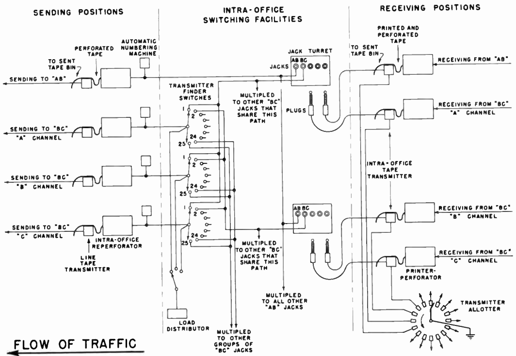
Figure 11. Switching to single-channel and multi-channel circuits
