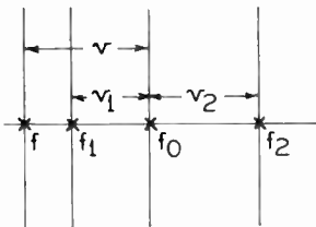
Figure 10. Relation of resonant and balance frequencies
