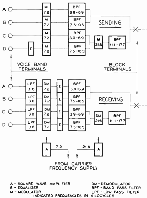
Figure 3. Voice band modulator group
