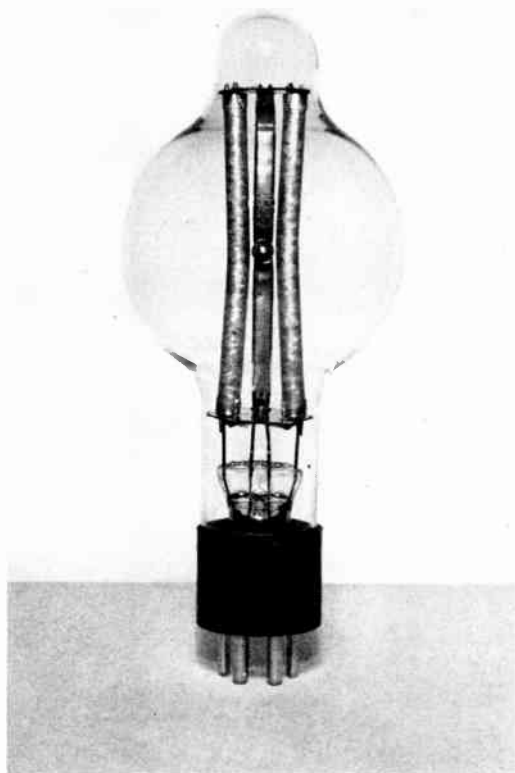
Figure 14. 300-watt Concentrated-arc lamp
