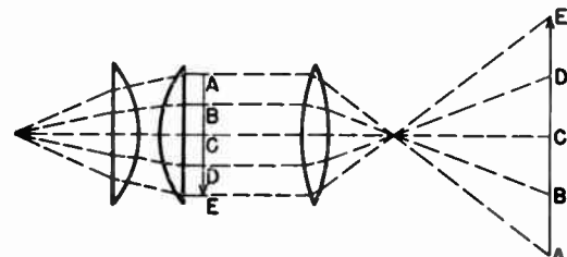
a—Light source at focal point of condenser.
