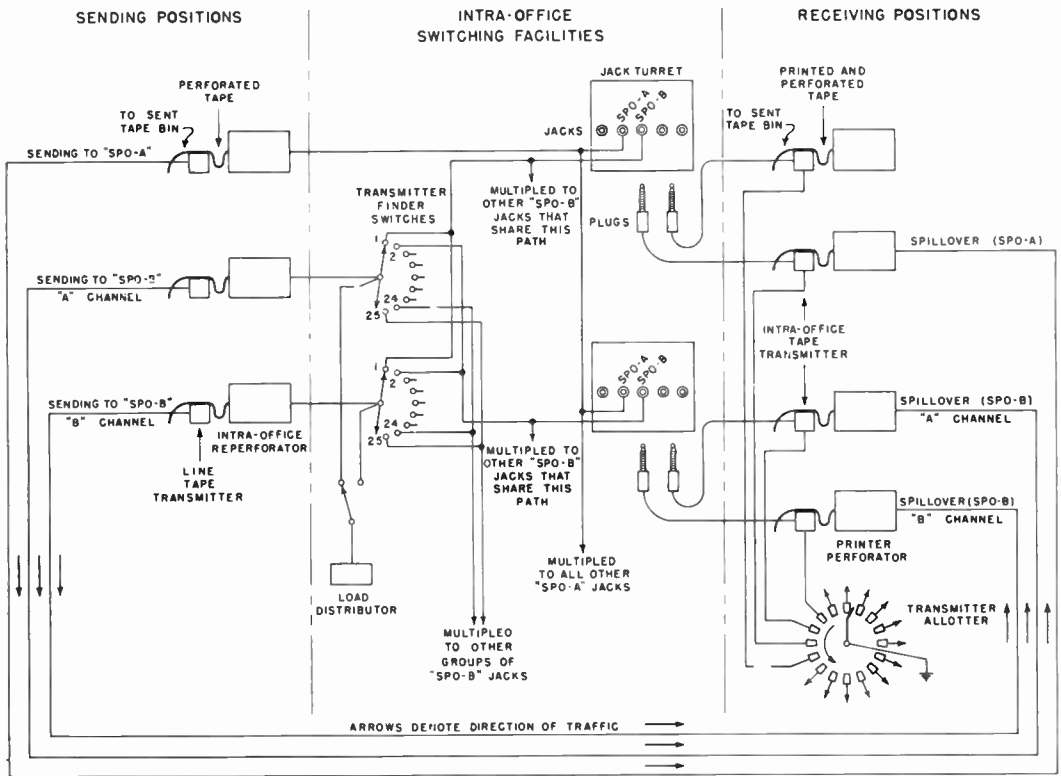
Figure 25. Single and multi-channel spillover positions
