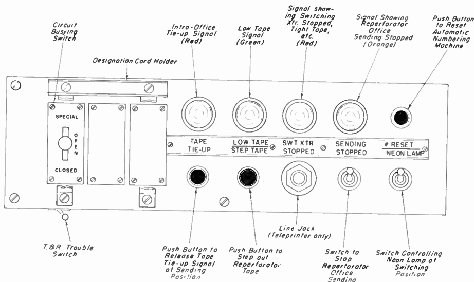
Figure 24. Sending position signal and control unit
