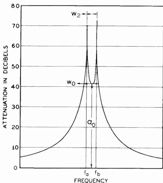
Figure 8. Attenuation characteristic of tandem rejection filters
