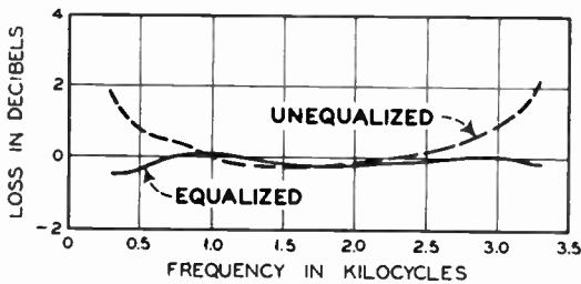
Figure 6. Voice band transmission frequency characteristic
