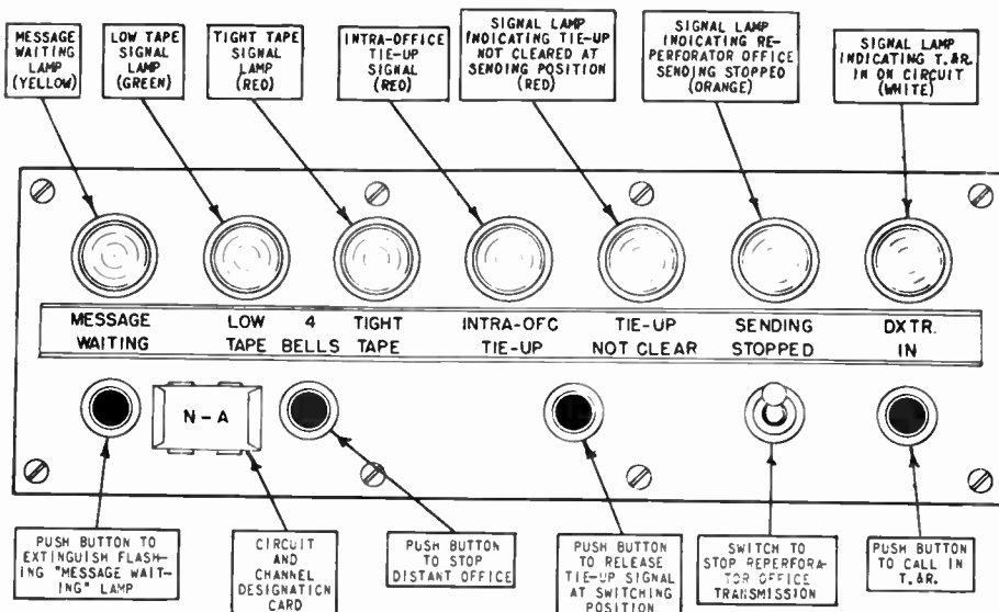
Figure 22. Multiplex signal and control unit
