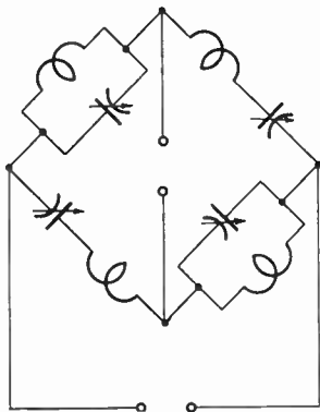
Figure 1. Basic circuit of the rejection filter
