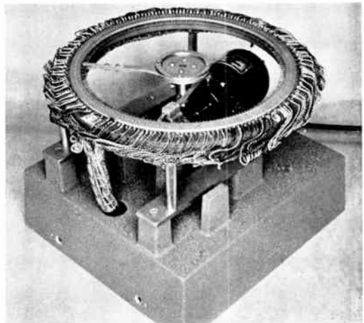
Figure 18. Transmitter allotter
