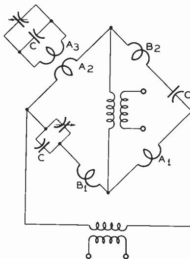
Figure 5. Practical circuit of the rejection filter
