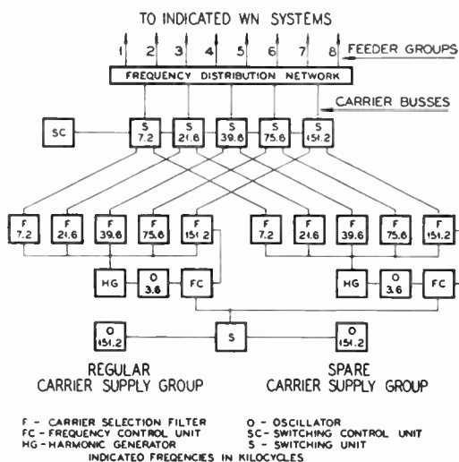
Figure 8. Carrier supply group
