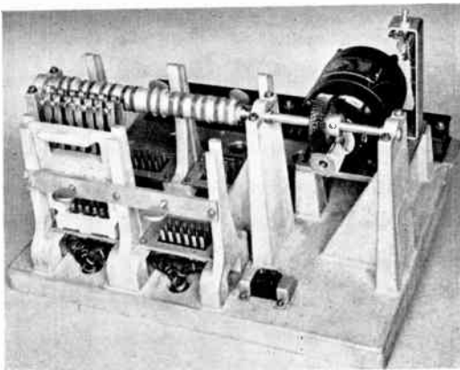
Figure 16. Impulse unit sub-base
