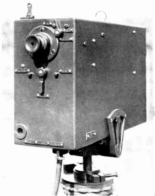
Figure 11. Light-beam telephone transmitter-receiver unit using Concentrated-arc lamp
