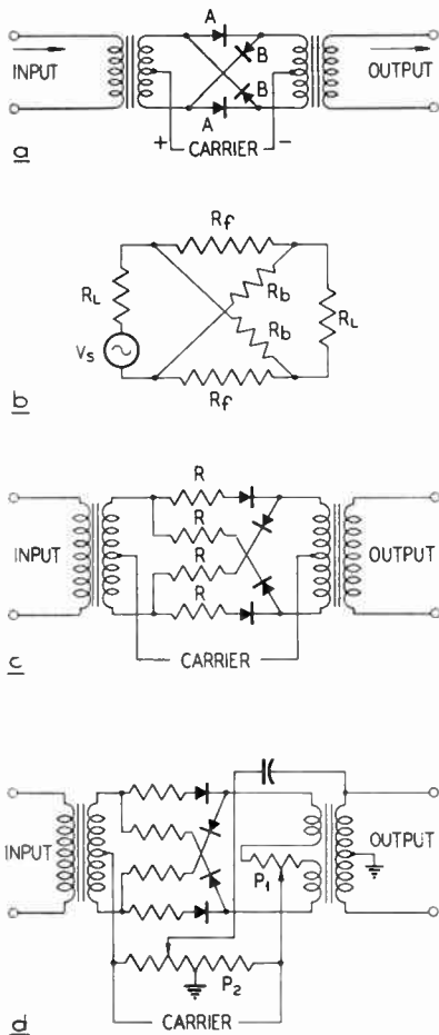
Figure 5. Modulator circuits
