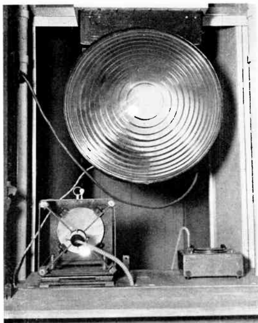
Figure 12. Light-beam transmitting and receiving equipment used on experimental circuit over New York City
