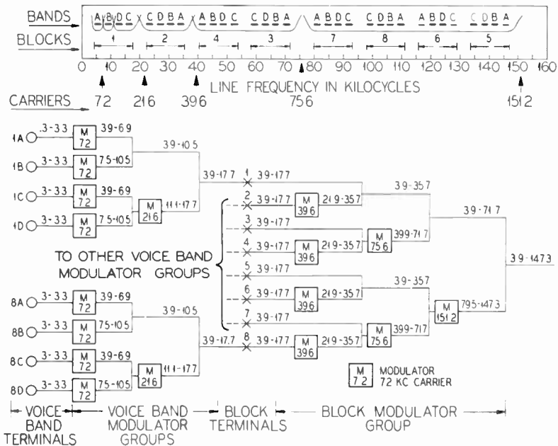
Figure 1. System theory and frequency allocations
