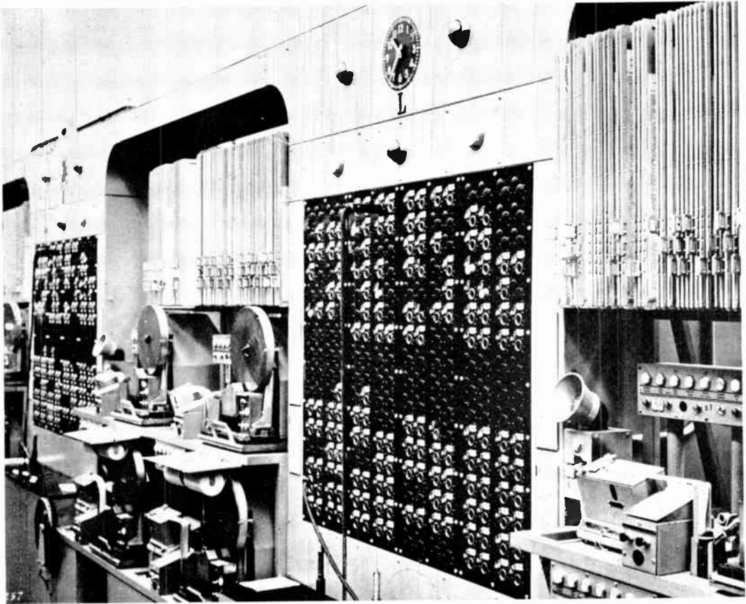
Figure 21. Line receiving position and jack turrets
