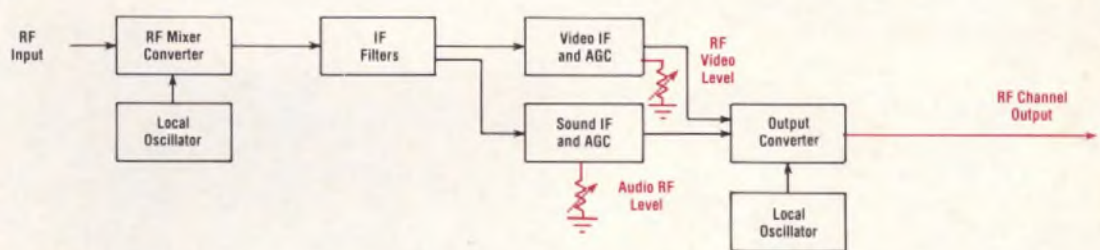
Heterodyne Processor Block Diagram
