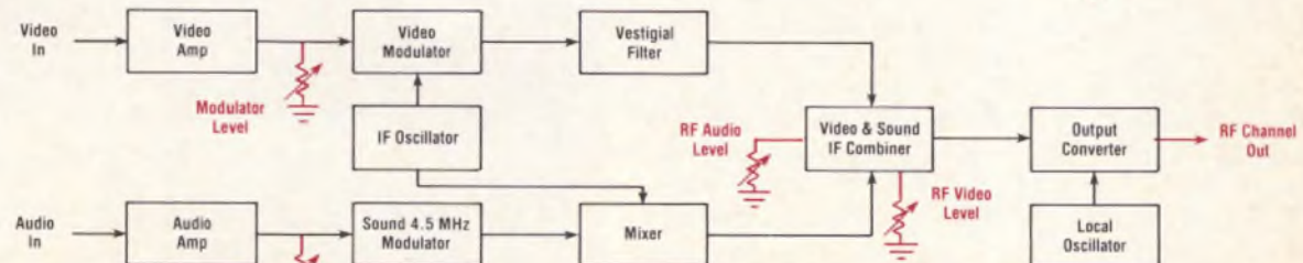
Block Diagram of Modulator
