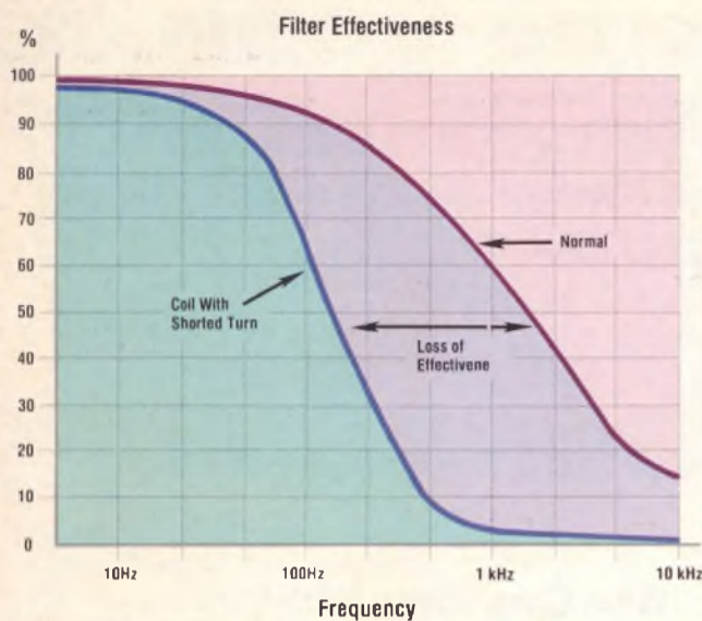
Fig. 2: Reduced Q causes the power filter to have a much lower effect on the ripple signal.
