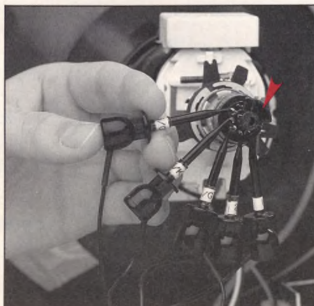
Fig. 4: Hook the Universal Adapter to the actual pins of the CRT using the setup book information. Count the CRT pins clockwise starting from the focus pin or keyway.
